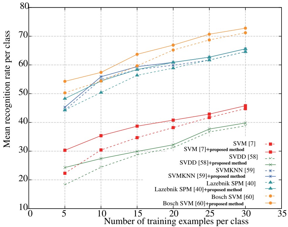
(a) Caltech 101.
