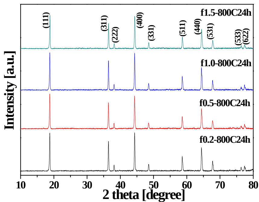
Figure 2. XRD patterns of the samples obtained at different fuel ratios and calcined at 800 °C for 24 h with fast cooling.
