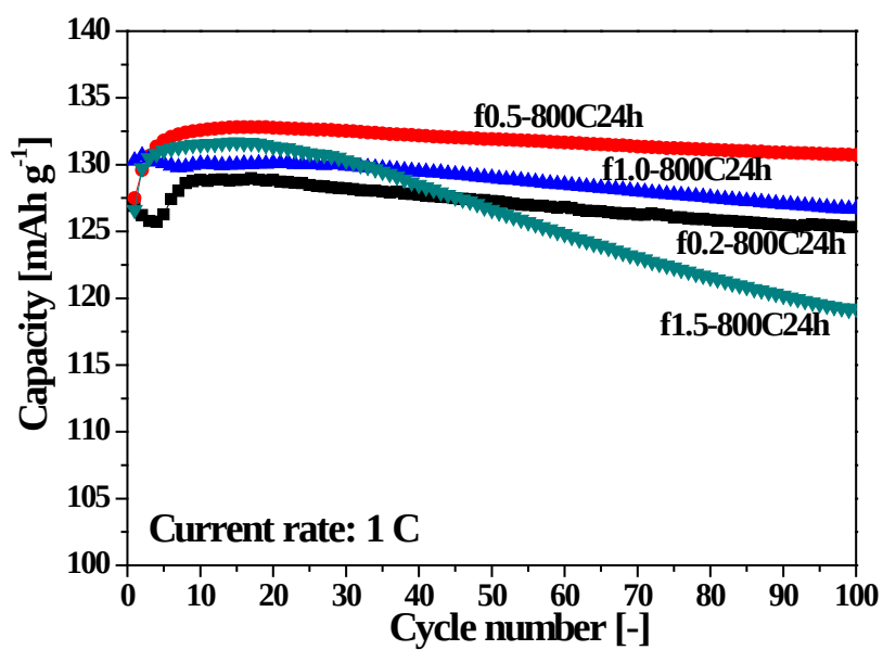
Figure 4. Cycling performance of the samples at a current rate of 1 C.
