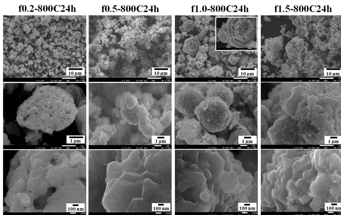
Figure 3. SEM images of the samples obtained with different fuel ratios and calcined at 800 °C for 24 h with fast cooling.
