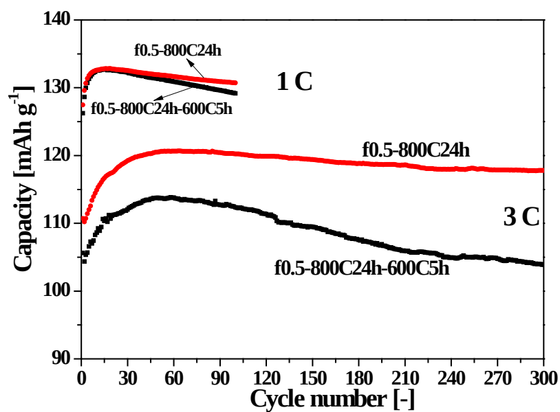
Figure 8. Cycling performance of f0.5-800C24h-600C5h and f0.5-800C24h samples.
