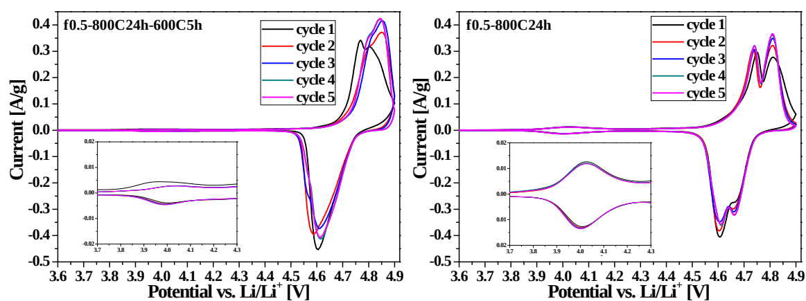
Figure 7. CV curves for the f0.5-800C24h-600C5h and f0.5-800C24h samples.
