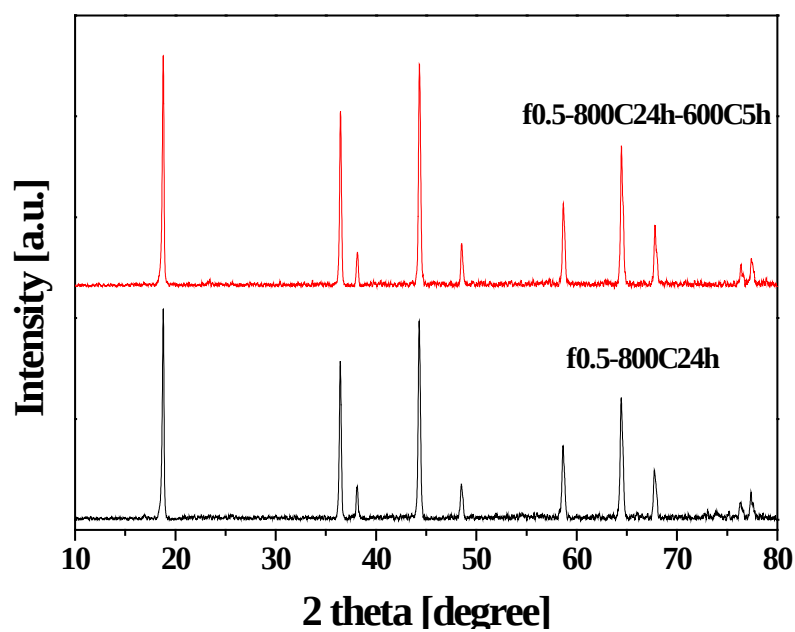
Figure 5. XRD patterns for the f0.5-800C24h-600C5h and f0.5-800C24h samples.
