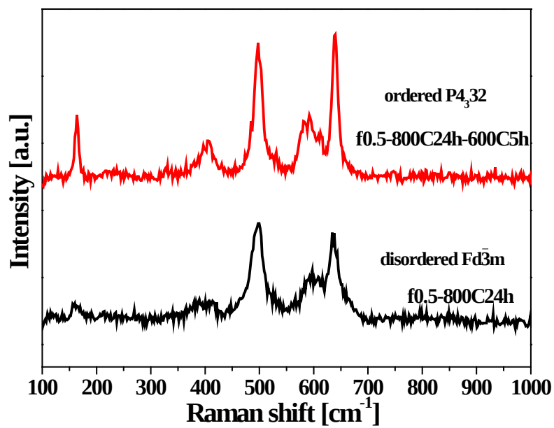
Figure 6. Raman spectra for the f0.5-800C24h-600C5h and f0.5-800C24h samples.
