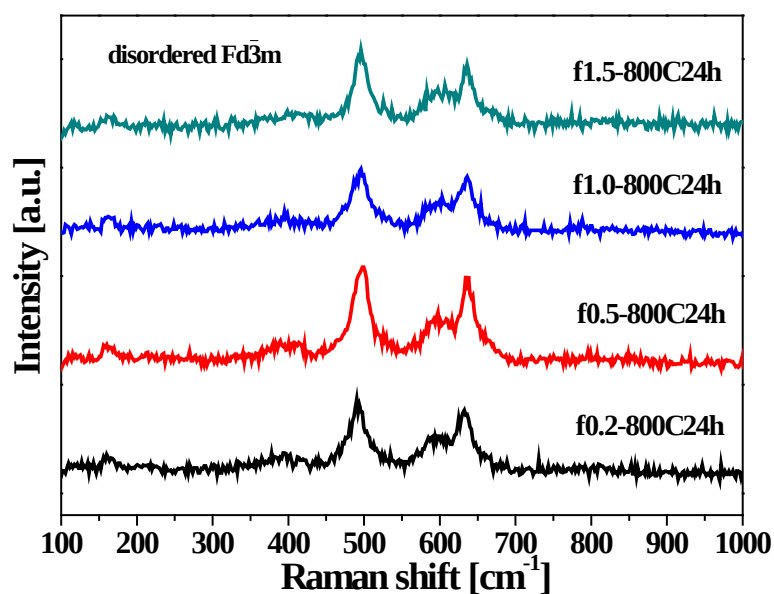
Figure 1. Raman spectra of the samples obtained at different fuel ratios and calcined at 800 °C for 24 h with fast cooling.
