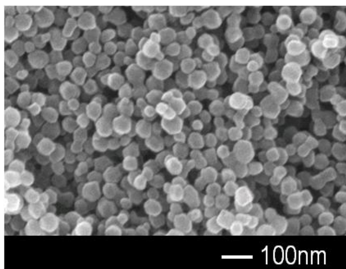
Figure 6.3 FE-SEM photographs of ZIF-8 crystals
