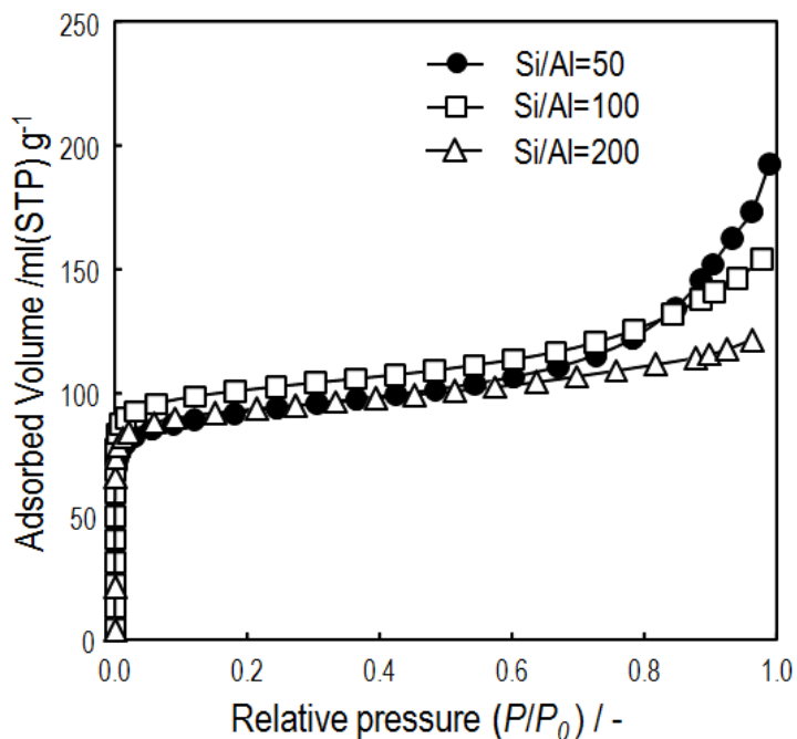
Figure 4.4 Nitrogen adsorption isotherms of nanometer-sized MTW crystals synthesized with different Si/Al ratios.
