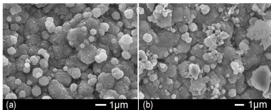
Figure 4.12 FE-SEM photographs of MTW nanocrystal-layered membrane surface areas ((a) before acetic acid /water pervaporation experiment, (b) after acetic acid /water pervaporation experiment).
