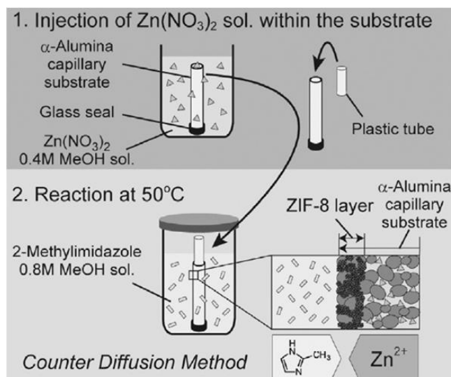
Figure 1.9 Schematic illustration of the counter diffusion method
