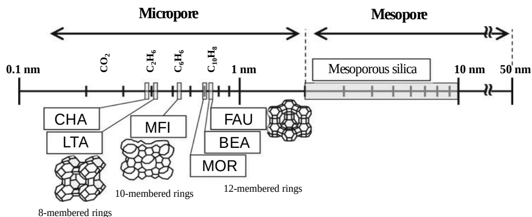
Figure 1.2 the comparison of zeolitic pore size and the hydrocarbon
