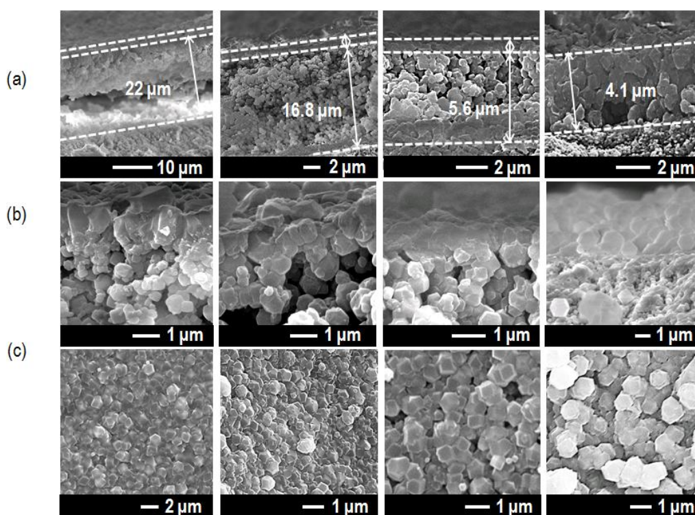
Figure 6.6 FE-SEM photographs of ZIF-8 membranes prepared with different thickness (a) cross section area, (b) protection layer by large magnification, and (c) top view.
