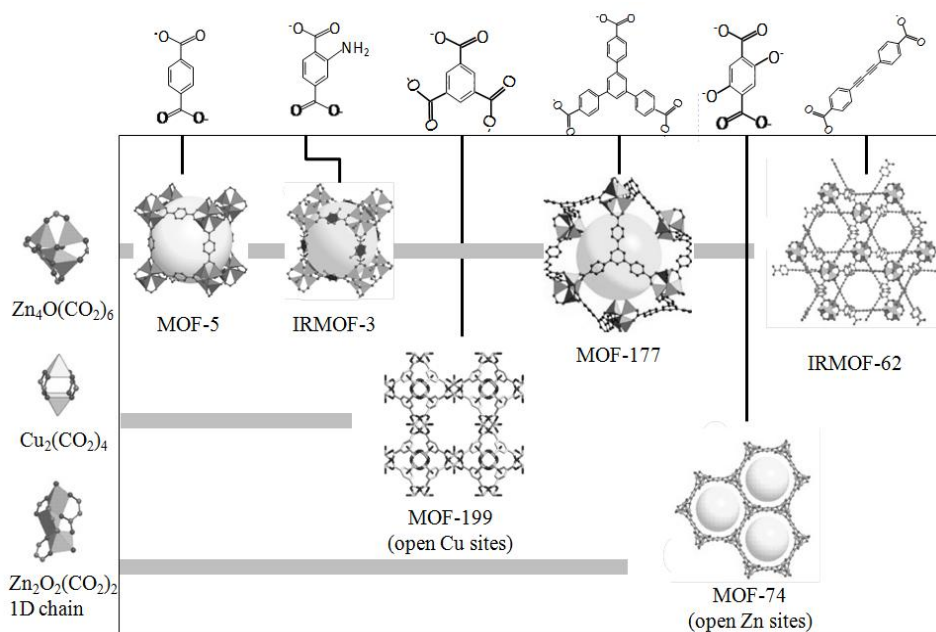
Fig. 1.7 The single-crystal x-ray structures of the benchmark MOFs: the \text{Zn}_4\text{O}(\text{CO}_2)_6 cluster linked by terephthalate (MOF-5), 2-aminoterephthalate (IRMOF-3), benzene-1,3,5-tris(4-benzoate) (MOF-177), and diacetylene-1,4-bis(4-benzoic acid) (IRMOF-62); the \text{Cu}_2(\text{CO}_2)_4 cluster linked by trimesate (MOF-199); and 1D \text{Zn}_2\text{O}_2(\text{CO}_2)_2 chains linked by 2,5-dihydroxyterephthalate (MOF-74).
