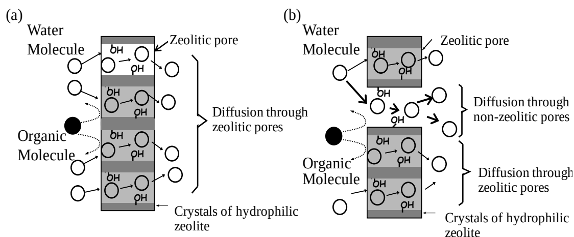
Figure 1.5 Representation of transport of an organic/water mixture through: (a) a hydrophilic zeolite membrane with only zeolitic pores; (b) a hydrophilic zeolite membrane containing hydrophilic non-zeolitic pores.
