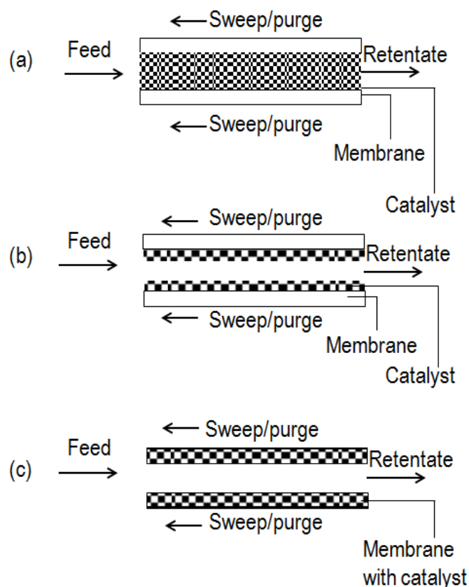
Different types of catalytic membrane reactors: (a) bore of tube filled with catalyst, (b) top layer with catalyst and (c) membrane wall with catalyst.
