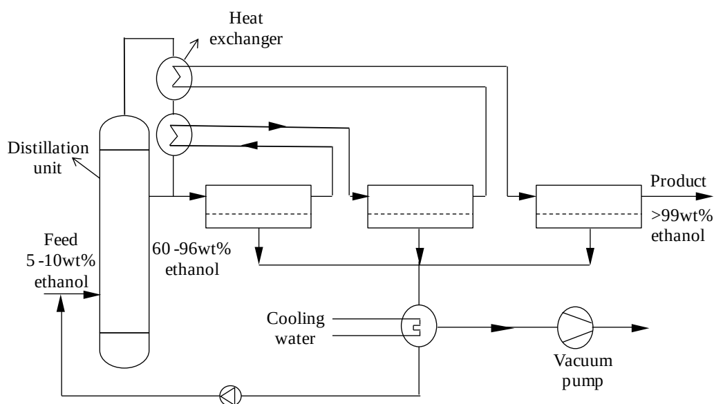
Figure 1.6 Flow diagram of a hybrid process for pure alcohol production,
