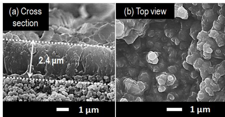
Figure 6.8 FE-SEM photographs of ZIF-8 membranes prepared by counter diffusion method (a) cross section area, (b) top view.
