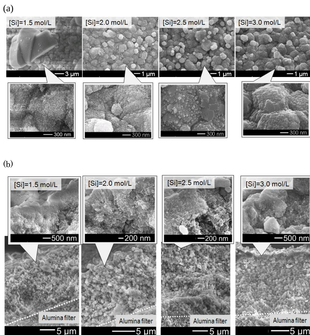
Figure 4.7 FE-SEM images of nanocrystal-layered MTW membranes with protection layers formation by using different mother liquid concentration. (a) Overhead view (b) cross-sectional view.
