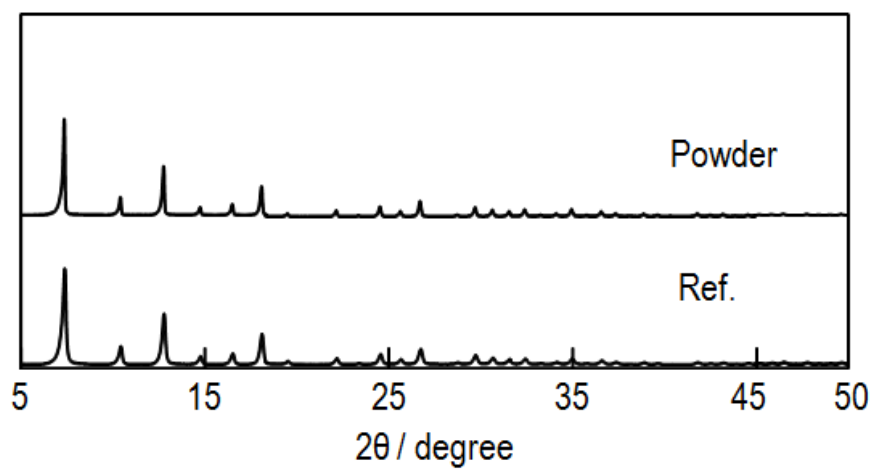
Figure 6.2 XRD patterns of (a) ZIF-8 crystals [15], (b) the powder obtained
