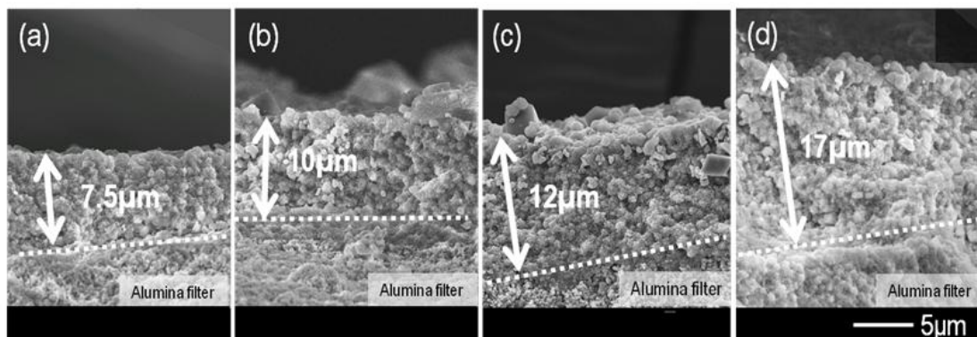
Figure 5.2 FE-SEM images of nanocrystal-layered MTW membranes prepared with different thicknesses.
