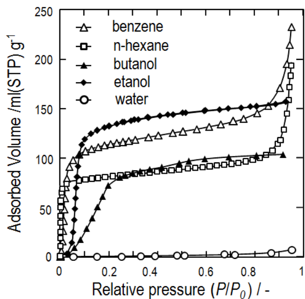
Figure 6.5 Gas adsorption isotherms of ZIF-8 nanometer size crystals.
