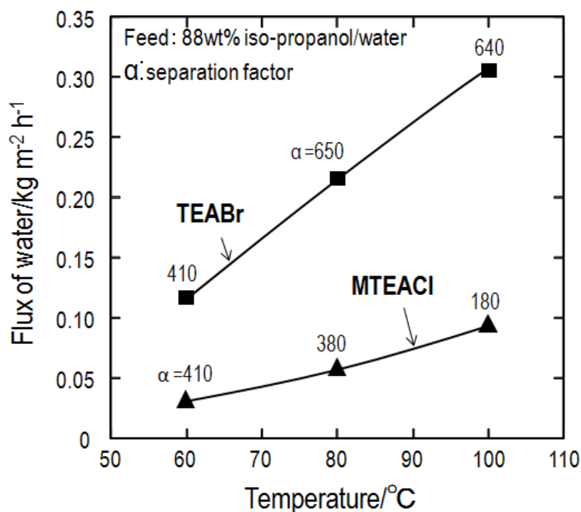
Figure 5.1 Water fluxes from water/2-propanol solutions through MTW membranes prepared using TEABr or MTEACl as the OSDA. The numerical values close to the lines indicate separation factors ( \alpha ).
