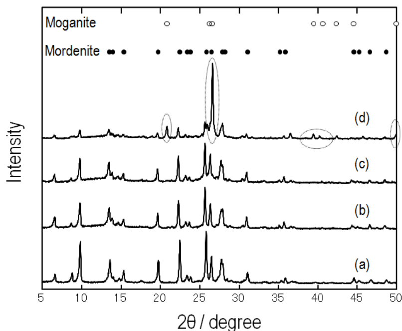
Figure 3.1 XRD patterns of (a) commercial mordenite, and powders obtained in solution after protection layer formation at (b) 150°C (c) 180°C and (d) 200°C.
