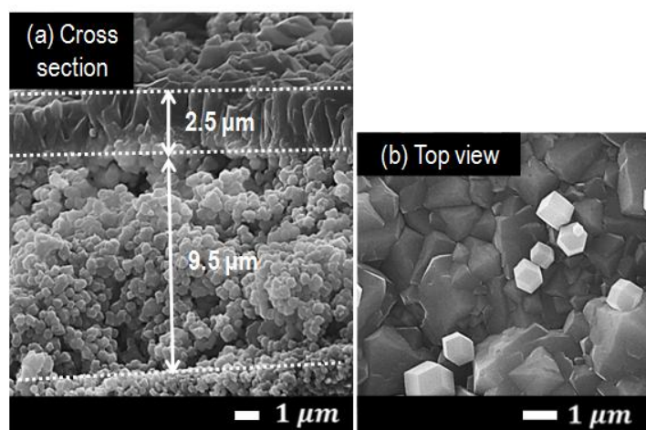
Figure 6.7 FE-SEM photographs of ZIF-8 membranes prepared by repeated synthesis. (a) cross section area, (b) top view.
