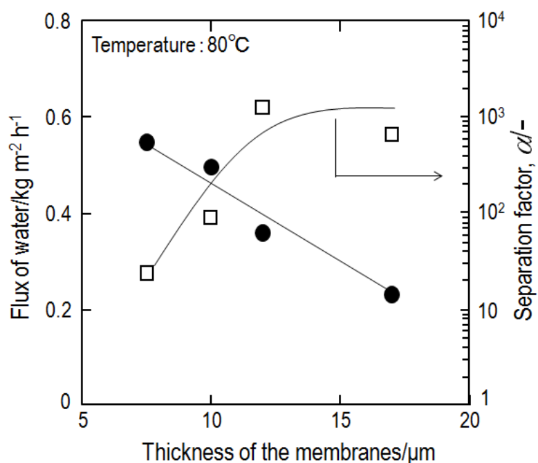
Figure 5.3 Effect of nanocrystal layer thickness in MTW membranes on permeability and separation ability from water/2-propanol solutions.
