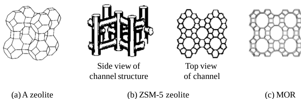
Figure 1.3 zeolite molecular sieve structure (a) A type zeolite, (b) ZSM-5 zeolite, (c) MOR
