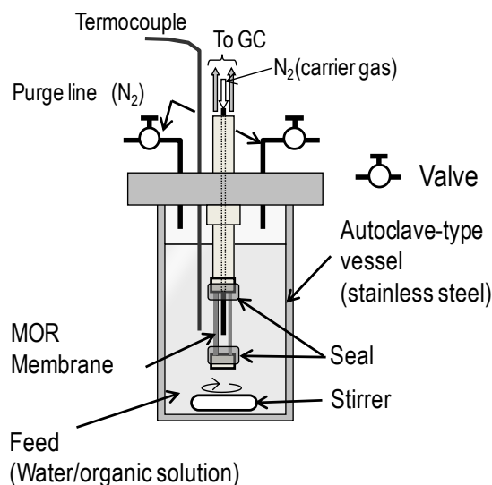
Figure 2.1 Schematic of the stainless steel autoclave vessel used for pervaporation experiments
