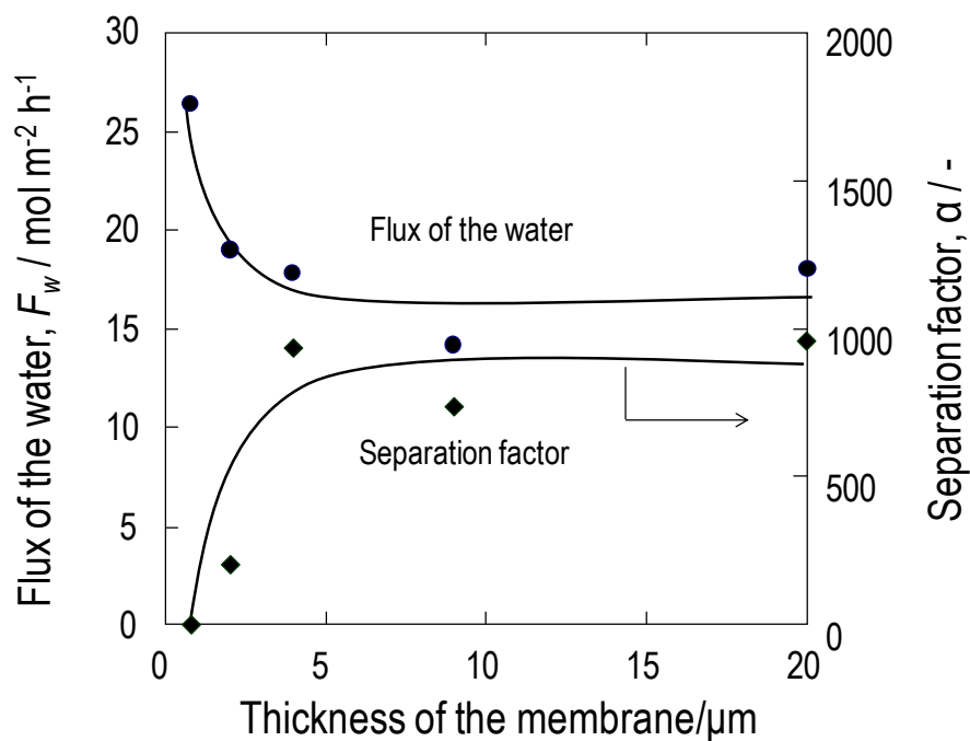
Figure 2.6 Effect of nanocrystal layer thickness in MOR membranes on water flux and separation ability from water / 2-propanol solutions.
