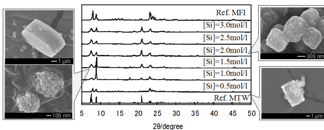
Figure 4.8 XRD patterns for MTW powders obtained in solution after protection layer formation in different concentration mother liquid.
