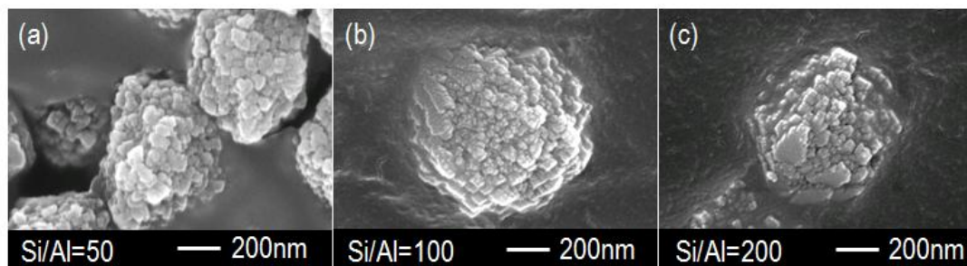
Figure 4.3 FE-SEM images of nanometer-sized MTW crystals synthesized with different Si/Al ratios.
