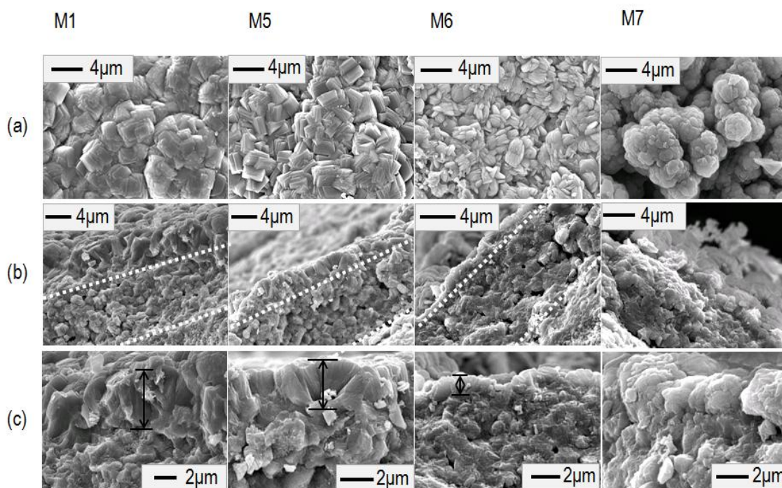
Figure 3.3 FE-SEM photographs of mordenite nanocrystal-layered membranes, containing a protection layer synthesized after pre-aging of the mother liquid: (a) top view, (b) cross-sectional area, and (c) interface area by large magnification.
