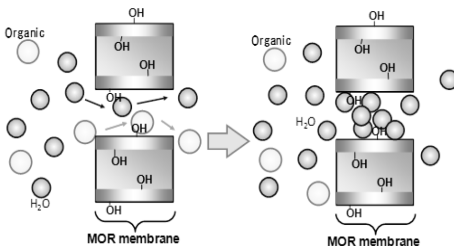
Figure 2.4 Formation of the water-acid site network.
