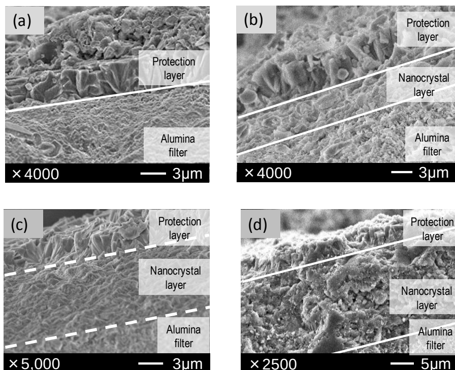
Figure 2.5 FE-SEM images of nanocrystal- layered MOR membranes prepared with different thickness of (a) 0.8 \mu\text{m} , (b) 4 \mu\text{m} , (c) 8 \mu\text{m} , and (d) 20 \mu\text{m} .
