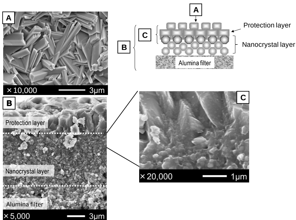
Figure 2.2 FE-SEM photographs of mordenite nanocrystal-layered membranes (A) top view, (B) cross-sectional area, and (C) magnified view of the indicated area.
