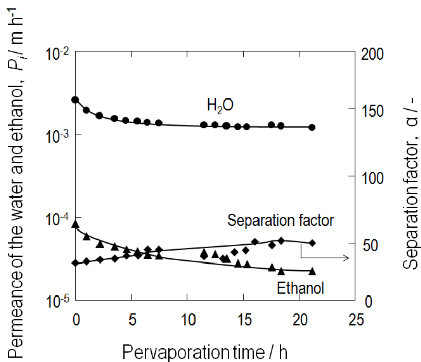
Figure 2.3 Permeance of the water and ethanol through the membrane and the changes of separation factors according to the pervaporation time.
