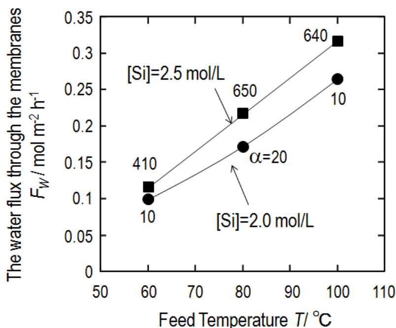
Figure 4.9 Water flux of membrane prepared with different concentration.
