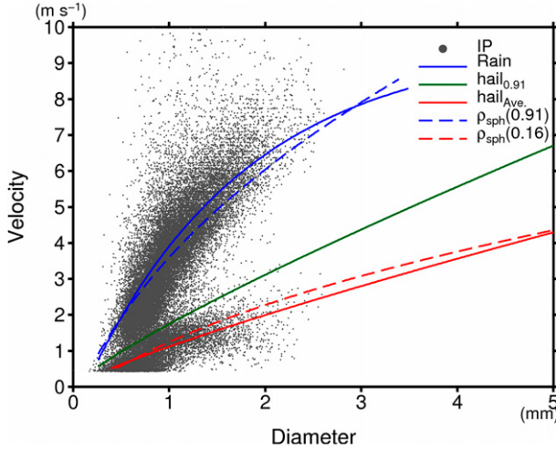
FIG. 9. Relationship between fall velocity and diameter of IPs observed from 0900 to 1000 LST. The solid blue line indicates velocity–diameter relationships for raindrops (Atlas et al. 1973), the solid green line indicates hailstones with a density of 0.91 \text{ g cm}^{-3} , and the solid red line indicates the average density of hailstones ( 0.44 \text{ g cm}^{-3} ) (Knight and Heymsfield 1983). The dashed blue line indicates terminal fall velocities for smooth ice spheres with densities of 0.91 \text{ g cm}^{-3} , and the dashed red line indicates those for smooth ice spheres with densities of 0.16 \text{ g cm}^{-3} (Mikhailov and Silva Freire 2013). The fall velocity relationships for hail are extrapolated to particles smaller than 5 mm in size that are typically not considered to be hail.
