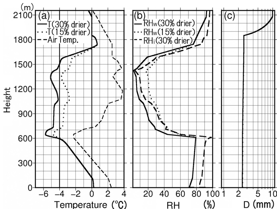
FIG. 12. Vertical profiles of simulated particles in the environments altered from Fig. 10 at 600–1700 m. (a) Particle temperature: solid line shows particle temperature with 30% drier relative humidity than in Fig. 10, dotted line shows particle temperature with 15% drier relative humidity than in Fig. 10, and dashed line denotes air temperature. (b) Relative humidity: solid line indicates 30% drier, dotted line 15% drier, and thick dashed line denotes relative humidity of ice in the 30% drier simulation. (c) Particle diameter: solid line indicates 30% drier, dotted line 15% drier. The dotted line overlaps the solid line. Initial snowflake conditions of this simulation: diameter is 10.0 mm and density is 0.02 \text{ g cm}^{-3} .
