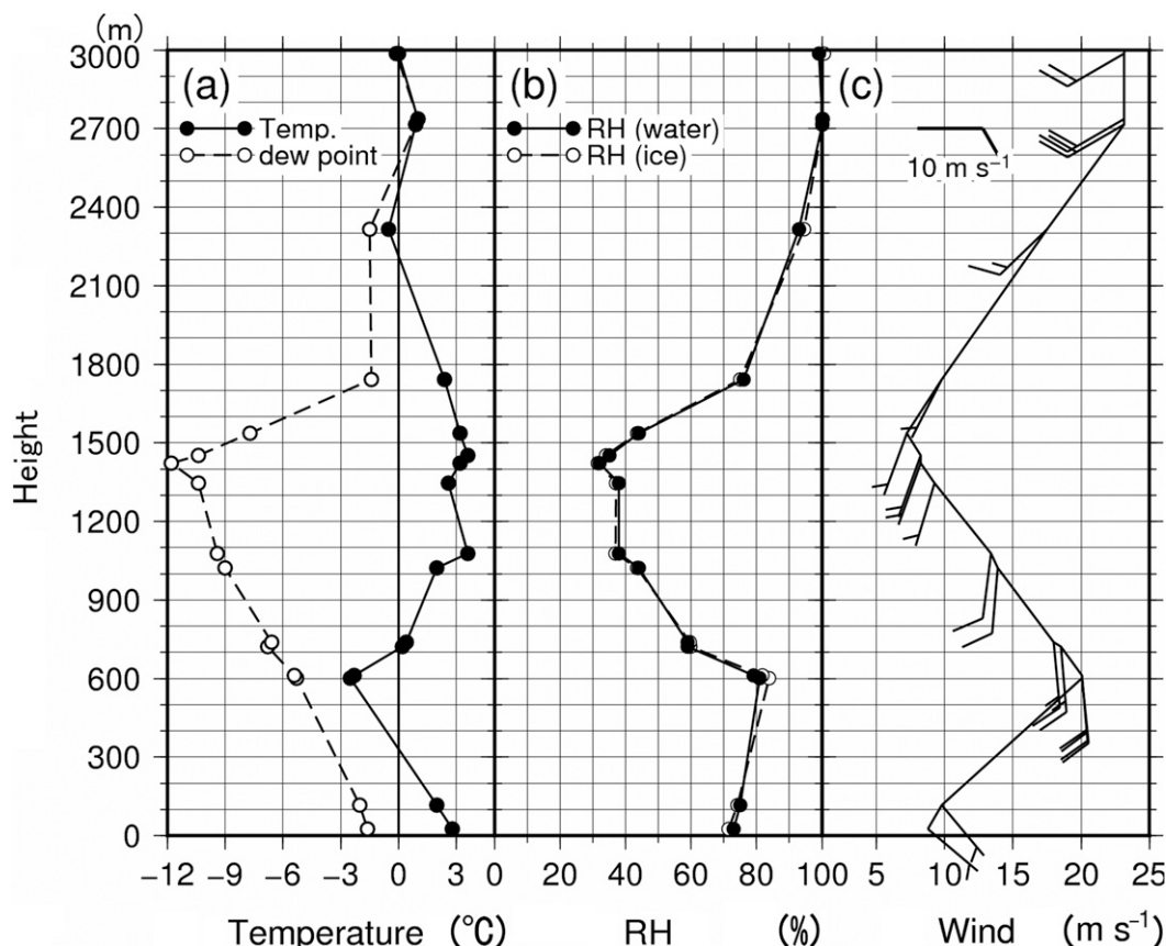
FIG. 3. Vertical profiles of (a) temperature (air temperature denoted by the solid line and dewpoint temperature denoted by the dashed line), (b) relative humidity, and (c) wind speed and wind direction observed at SDMO at 0900 LST (0000 UTC) 10 Apr 2005. Heights are in m AGL.
