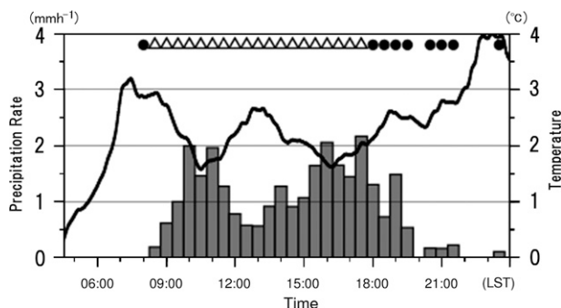
FIG. 6. Temporal evolution of precipitation rate (bars) and surface air temperature (solid line) with observed precipitation types on 10 Apr 2005. Black circles denote raindrops, and white triangles denote ice pellets. All data were obtained at ILTS.
