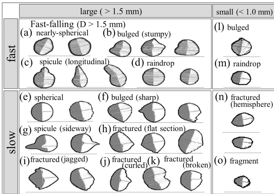
FIG. 13. IP silhouettes from 2DVD. Typical images of (a)–(d) large, fast-falling pellets; (e)–(k) large, slow-falling pellets; (l), (m) small, fast-falling pellets; and (n), (o) small, slow-falling pellets.
