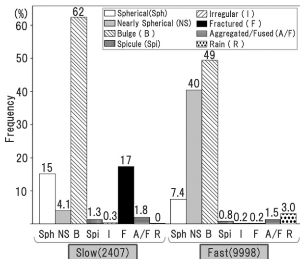
FIG. 14. Histogram of classes of fast- and slow-falling ice pellets larger than 1.5 mm in diameter, with their total numbers in parentheses.
