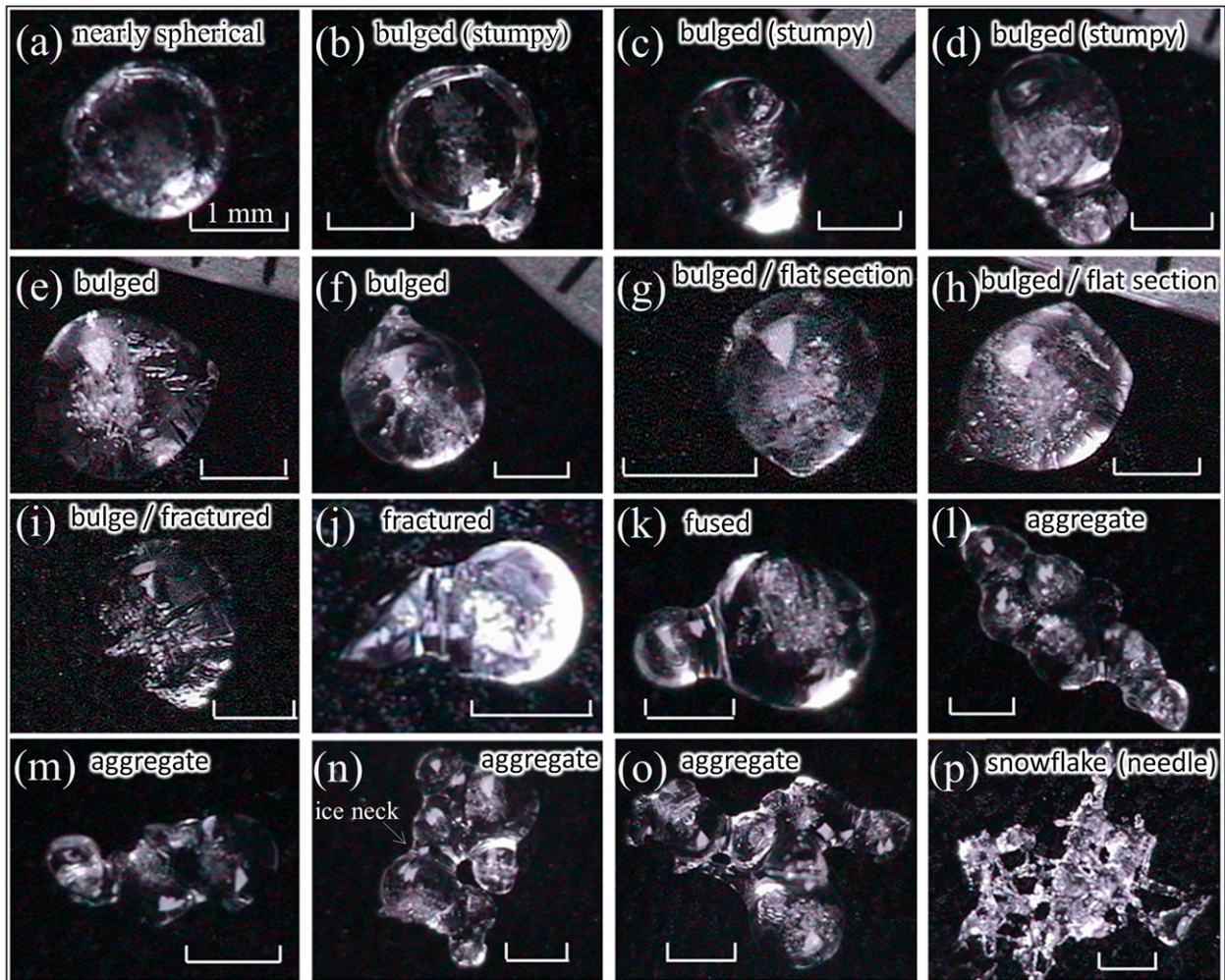
FIG. 8. Photographs of (a)–(o) ice pellets taken from 1400 to 1500 LST 10 Apr 2005, and (p) the only snowflake found during this period (representatives of 39 total photographs).
