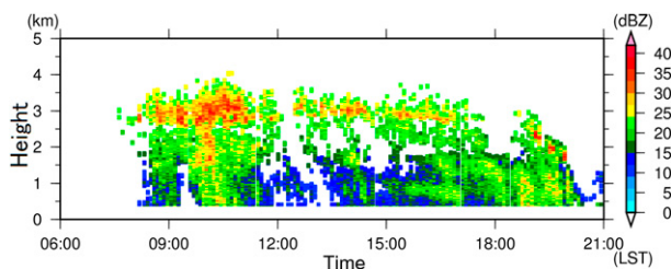
FIG. 5. Time–height cross section of the radar reflectivity factor over Sapporo on 10 Apr 2005 (LST). Heights are in km AGL.
