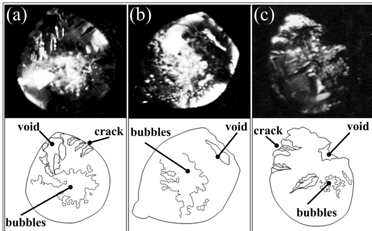
FIG. 15. As in Fig. 8, but for enlarged and contrast-enhanced photographs of (top) fractured ice pellets and (bottom) outlines. Solid lines in the outline depict silhouette and fracture points (cracks and voids) and dashed lines depict peripheries of bubbles.
