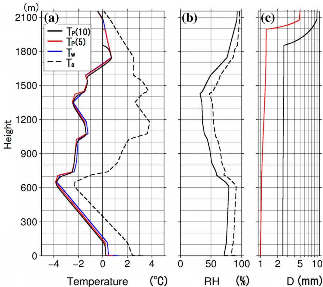
FIG. 10. Vertical profiles of environmental and simulated particle conditions. (a) Particle temperature T_p , air temperature T_a , and wet-bulb temperature T_w based on sounding data in Fig. 3. (b) Relative humidity profile with respect to liquid (solid line) and ice (dashed line). (c) Simulated particle diameter at each vertical level. Black lines denote initial particle diameters of 10.0 mm, and red lines denote those of 5.0 mm.
