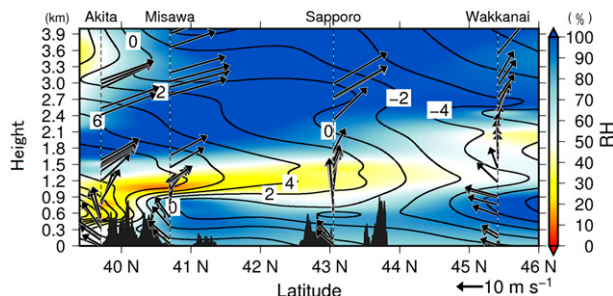
FIG. 4. Latitude–height cross section of air temperature (black contours) and relative humidity (color shade) at 0900 LST 10 Apr 2005, composited using observed data at four upper-air sounding stations located between 39° and 46°N. Air temperature is in ^{\circ}\text{C} and relative humidity is in %.
