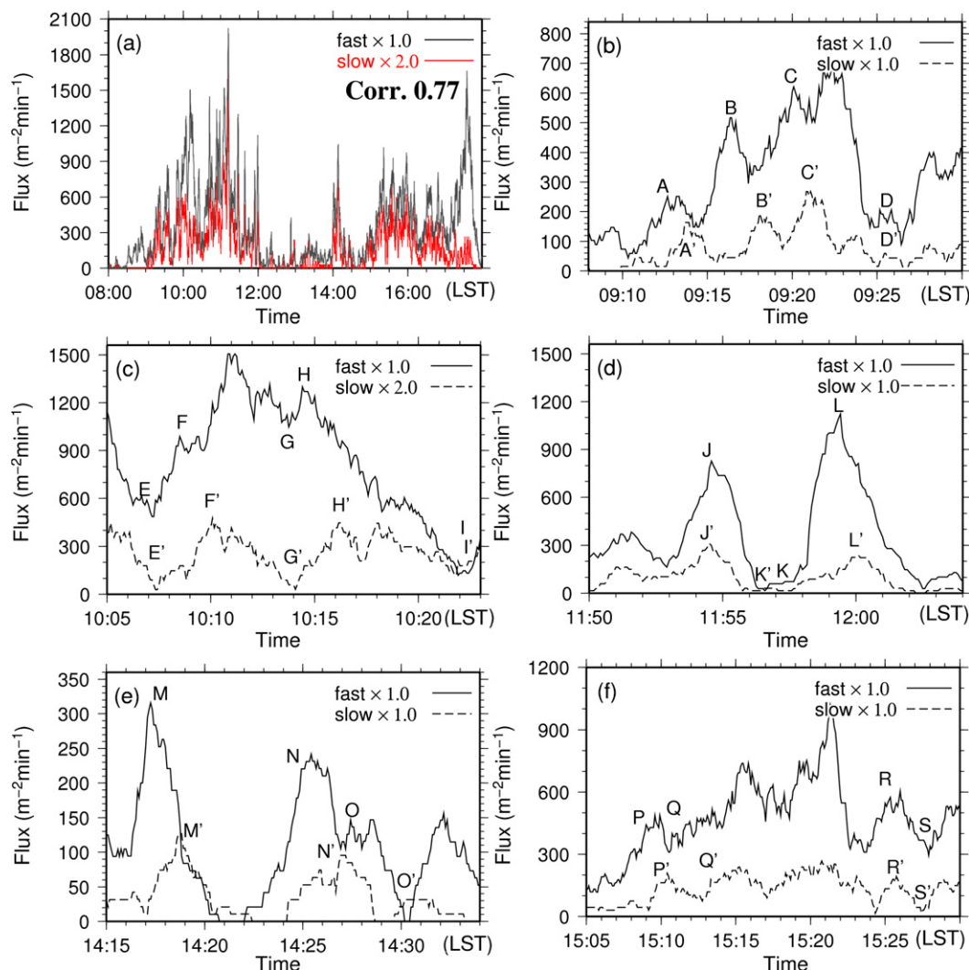
FIG. 16. Time series of particle number concentration fluxes ( \text{m}^{-2} \text{min}^{-1} ) of both fast- and slow-falling groups in the size range of 1.5–2.0 mm. Time resolutions are 5 s with a 75-s moving average for (a) the entire period of the ice-pellet event, (b) 0908–0930, (c) 1005–1023, (d) 1150–1204, (e) 1415–1434, and (f) 1505–1530 LST 10 Apr 2005. A–S indicate local peaks of fast-falling pellets, and A'–S' indicate local peaks of slow-falling pellets.
