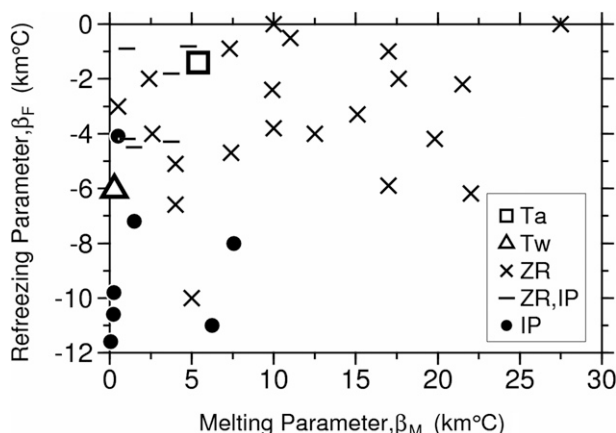
FIG. 11. Melting parameter vs refreezing parameter based on Zerr (1997). The square ( T_a ) denotes the parameters computed from the air temperature from a sounding at SDMO at 0900 LST. The triangle ( T_w ) denotes those from the simulated wet-bulb temperature. Other data points are observations presented in Zerr (1997). ZR denotes freezing rain, and IP denotes ice pellets.
