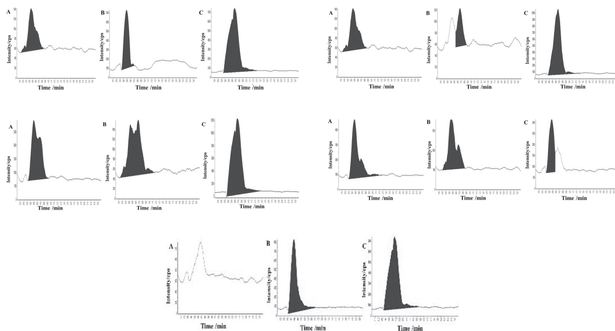
Fig.4. GC-ECD chromatogram showing the concentration of fipronil residues in A, Muscle. B, Liver and C, Abdominal fat Japanese quail of control group(1), LD 50 group(2), \frac{1}{2} LD 50 fipronil group(3), \frac{1}{5} LD 50 fipronil group, and \frac{1}{10} LD 50 fipronil group(5). Retention time is (0.543) 0.543minutes
