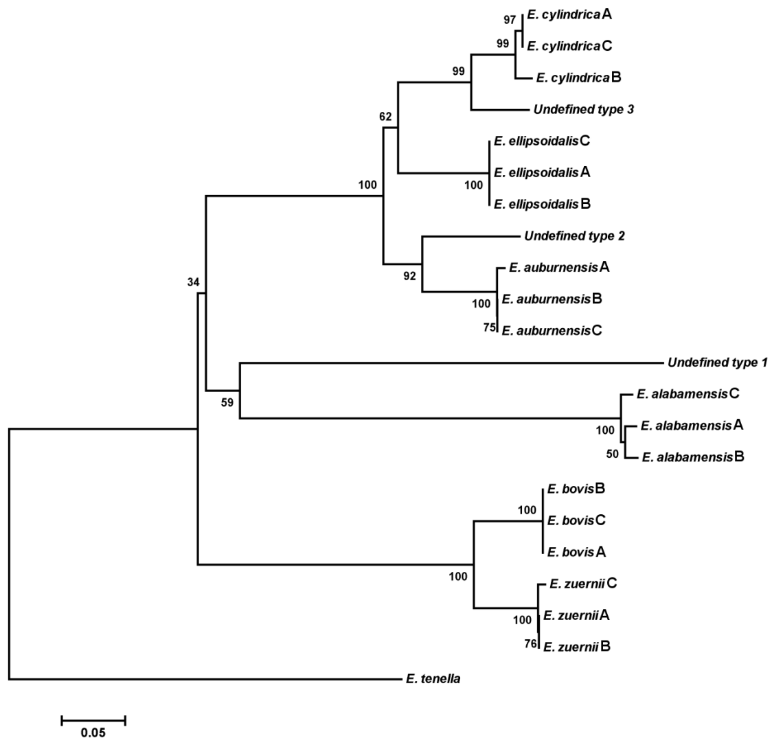
Fig. 1-1. Phylogenetic tree for all available ITS-1 sequences. The tree was rooted on Eimeria tenella , branch lengths indicated computed evolutionary distances using the neighbor-joining (NJ) method. Bootstrap support values from NJ are displayed on the nodes.
