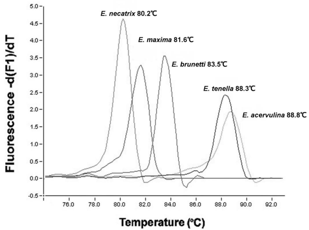
Fig. 2-3. Melting-curves of the control samples by real-time polymerase chain reaction assay.
