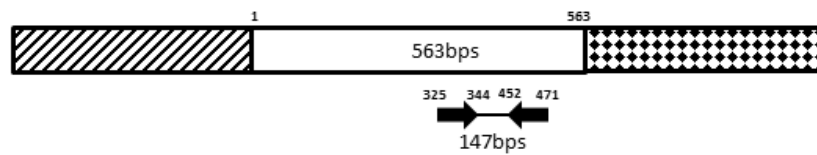
Fig. 2-1. Primer mapping on the shape of each species DNA sequences. Striped box, 18S rRNA gene; Opened box, ITS-1 region; Dotted box, 5.8S rRNA gene; Solid arrow, species-specific primer set; bps, size of ITS-1 region or PCR product; Small number, the order of nucleic acid residue based on ITS-1 region.
