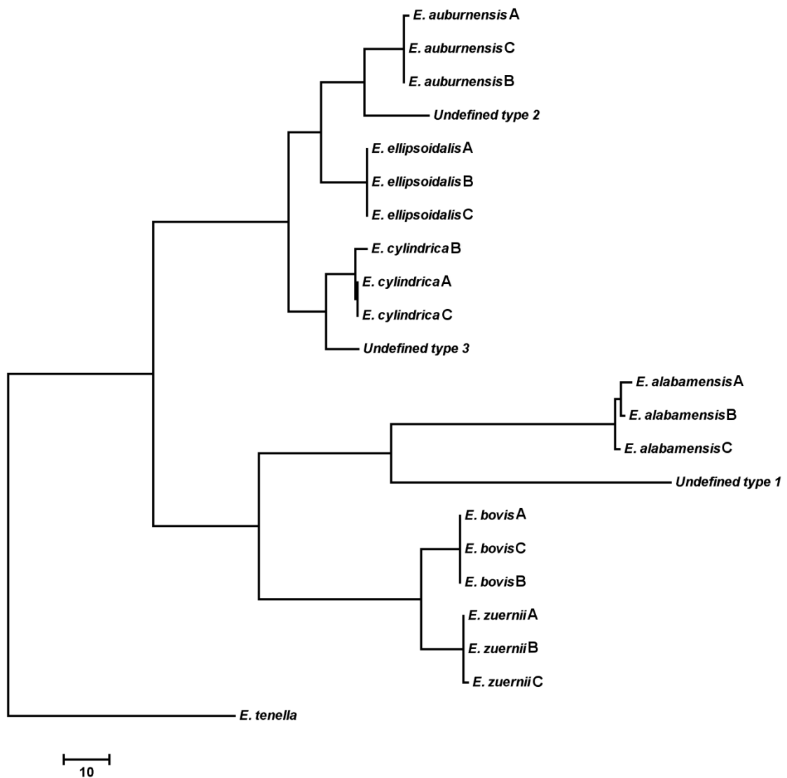
Fig. 1-2. Phylogenetic tree for all available ITS-1 sequences. The tree was rooted on Eimeria tenella , branch lengths indicated computed evolutionary distances using the maximum parsimony method.
