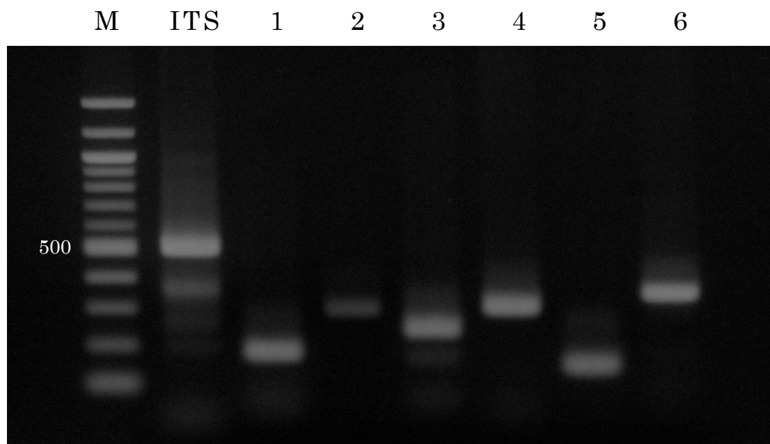
Fig. 1-5. Agarose gel electrophoresis of the PCR products amplified with species-mixed DNA samples by genus-common and species-specific primer sets. M: marker ladder (100 base pair). The different primer sets used are as follows: ITS, genus-common; 1, E. alabamensis -specific; 2, E. auburnensis -specific; 3, E. bovis -specific; 4, E. cylindrica -specific; 5, E. ellipsoidalis -specific; 6, E. zuernii -specific.
