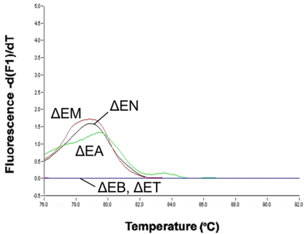
Fig. 2-4. Melting-curves of five DNA samples which were combined with different four species by real-time polymerase chain reaction assay. \Delta EA , mixed DNA without E. acervulina ; \Delta EB , mixed DNA without E. brunetti ; \Delta EM , mixed DNA without E. maxima ; \Delta EN , mixed DNA without E. necatrix ; \Delta ET , mixed DNA without E. tenella .
