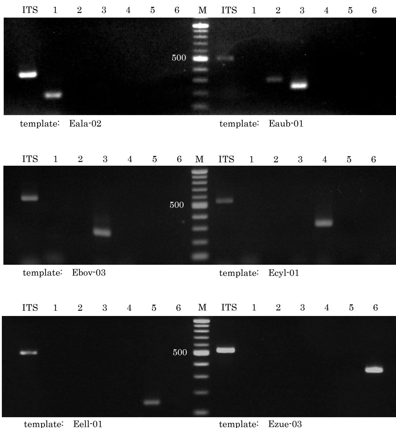
Fig. 1-4. Agarose gel electrophoresis of the PCR products obtained from the inter-species specificity assessment of six Eimeria species. M: marker ladder (100 base pair). The different primer sets used were as follows: ITS, genus-common; 1, E. alabamensis -specific; 2, E. auburnensis -specific; 3, E. bovis -specific; 4, E. cylindrica -specific; 5, E. ellipsoidalis -specific; 6, E. zuernii -specific. The six species-specific primer sets were tested in their efficiency using genomic DNA template indicated at the bottom.
