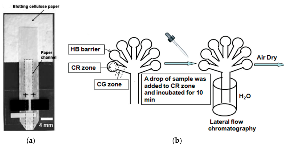
Figure 5. Detection methods for metals. (a) Electrochemical device for SWASV analysis of lead in water with screen-printed carbon working and counter electrodes and Ag/AgCl pseudo-reference electrode. Reprinted with permission from reference [47]. Copyright 2009 The Royal Society of Chemistry. (b) Multiplexed colorimetric detection of metals based on B-GAL and CPRG interaction in the presence of Hg^{2+} , Cu^{2+} , Cr^{6+} and Ni^{2+} mixture. Reprinted with permission from reference [31]. Copyright 2011 American Chemical Society.
