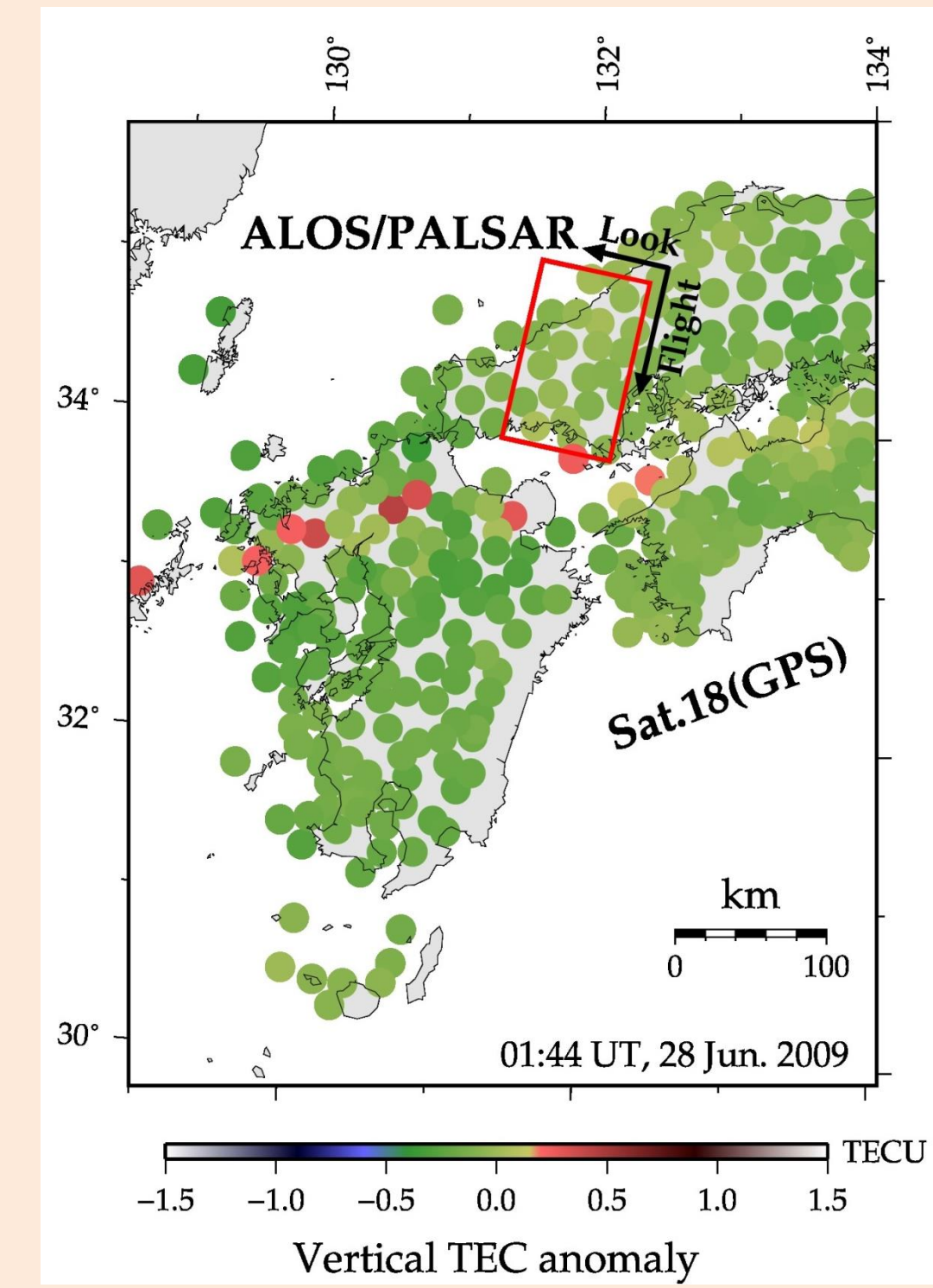
Fig.3 Vertical TEC anomaly map at 01:44 UT derived from GPS Satellite 18 when ALOS acquired the SAR image (red framed region). ALOS was on a descending orbit and observed Es looking the right side. Vertical TEC anomaly map shows a large-scale frontal structure which elongates over 250 km in the ENE-WSW direction. The SAR observation area corresponds to the eastern part of the frontal structure.
