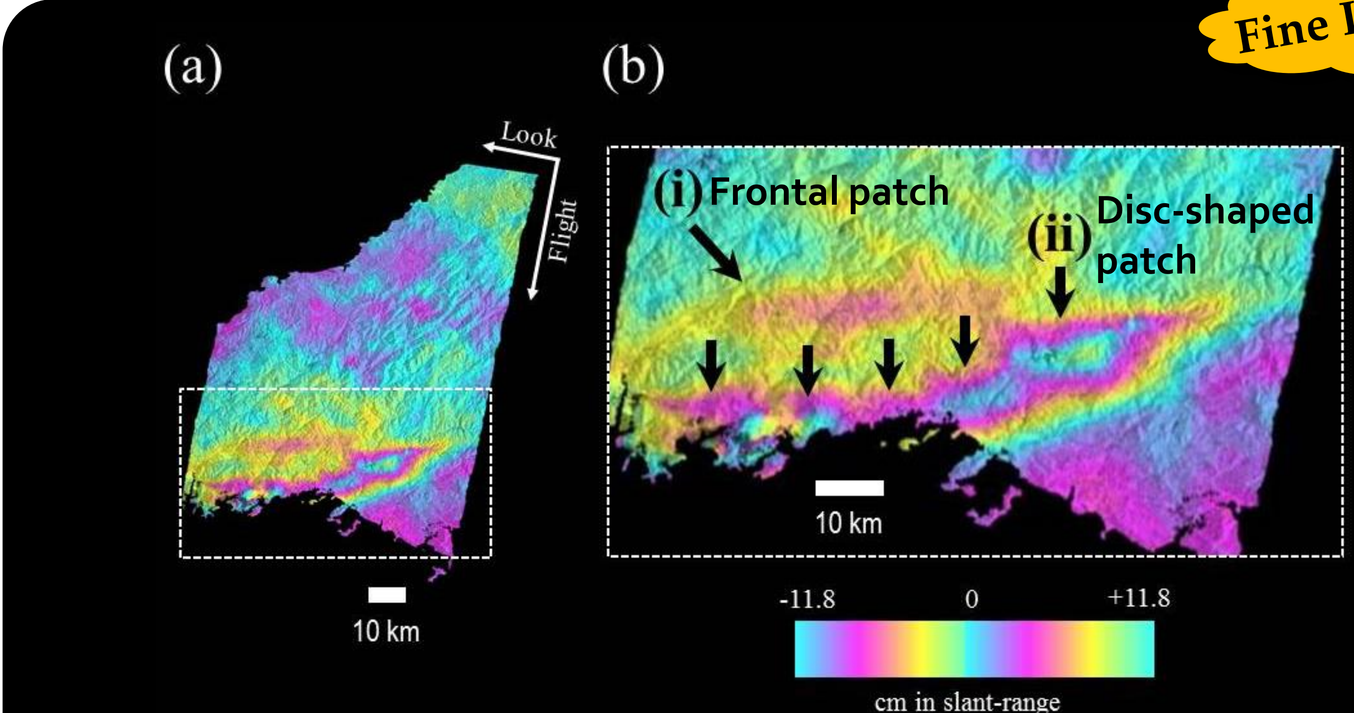
Fig.4 Interferogram derived from ALOS/PALSAR data (Path-frame: 72-2920~2930). The phase changes are shown as slant range changes in centimeter. Beginning with pale blue, the color changes into purple and into yellow represent positive and negative slant range changes, respectively. In an enlarged image in (b), (i) a frontal patch (pointed by a slant arrow) and (ii) a chain of disc-shaped patches (pointed by short black arrows) are clearly seen.
