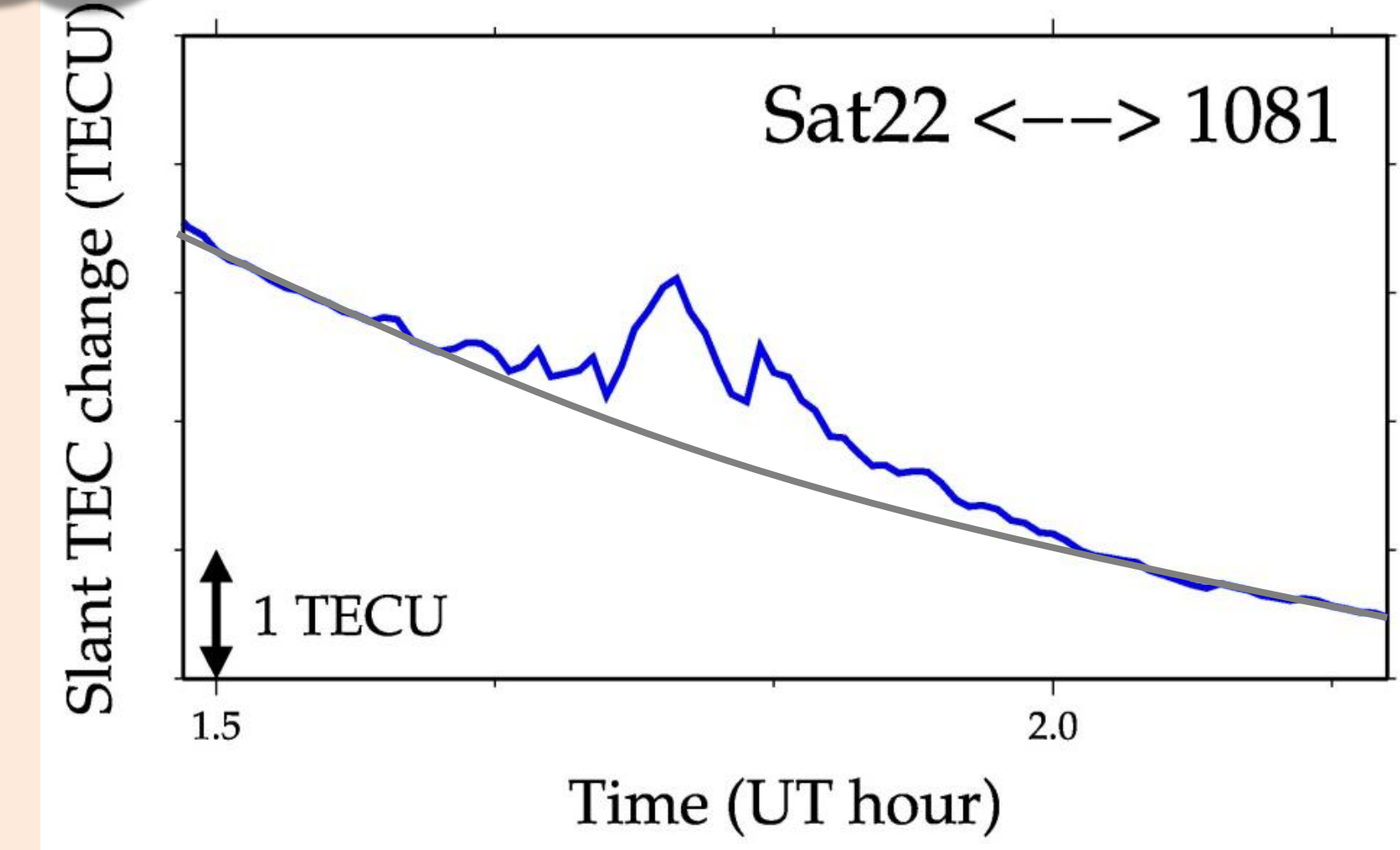
Fig.1 Slant TEC time series (observed / model). Es leaves peculiar signature of pulse-like positive TEC enhancement in the slant TEC time series. By analyzing the slant TEC time series with the corresponding SIP track, small-scale structures can also be inferred with GPS-TEC observation.
