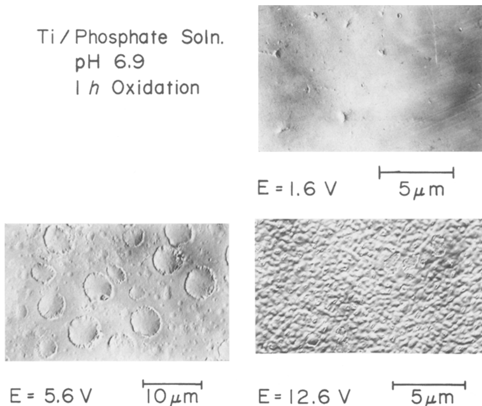
Fig. 7. Electron microscopic appearance of the surface of titanium covered with the anodic oxide film. The oxidation was made potentiostatically for 1 h in 0.1 mol dm -3 neutral phosphate solution.
