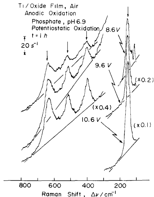
Fig. 5. Ex situ Raman spectra of the anodic oxide films formed on titanium at constant potential for 1 h in 0.1 mol dm -3 neutral phosphate solution. The bandpass of the spectrometer was about 10 cm -1 .
