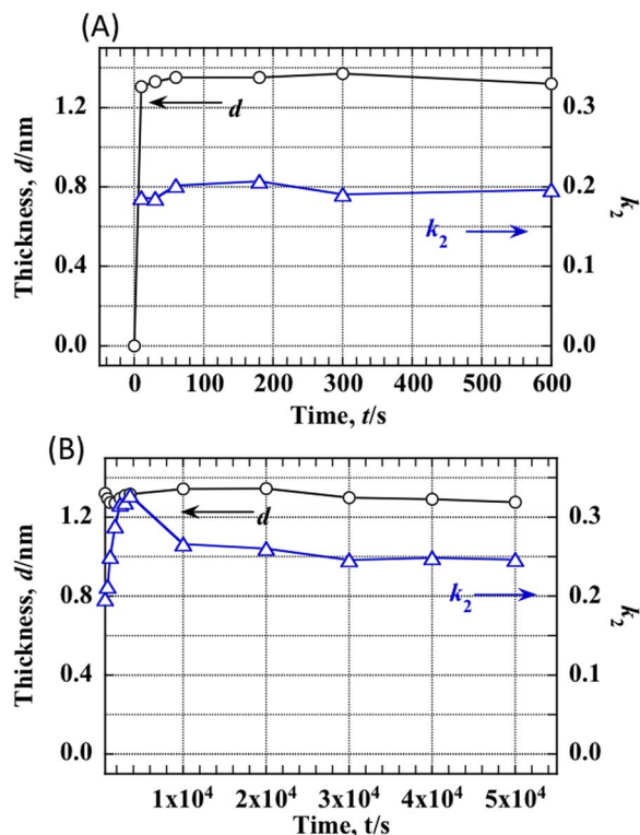
Figure 10. Film thickness of the passive oxide ( d ) as a function of oxidation time ( t ) at a constant potential at 0.6 V (A) for the initial period to 600 s (10 min), and (B) the period from 600 s to 50 ks (13.9 h).
