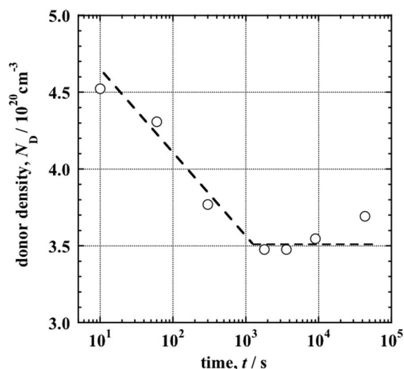
Figure 13. Donor density of the passive oxide film formed on SUS304 SS at 0.6 V vs. SSC for various times in a 0.1 M \text{H}_2\text{SO}_4 solution. The dielectric constant of the passive oxide was assumed to be 15.6.
