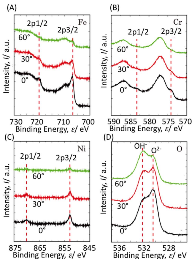
Figure 5. XPS spectra of (A) Fe, (B) Cr, (C) Ni, and (D) O of the passive oxide on SUS304 SS formed at 0.1 V vs. SSC for 1 h as a function of detection angle.
