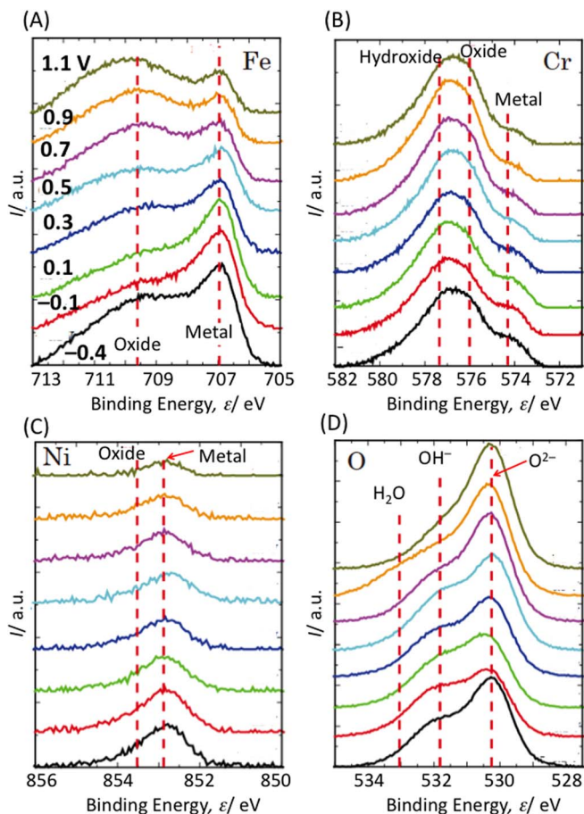
Figure 2. XPS spectra of (A) Fe2p3/2, (B) Cr2p3/2, (C) Ni2p3/2, and (D) O1s of the reduced and passivated type 304 SS at various potentials for 1 h in a 0.1 M H 2 SO 4 solution. The spectra were plotted from the bottom at -0.4 V, -0.1 V, 0.1 V, 0.3 V, 0.5 V, 0.7 V, 0.9 V, and 1.1 V vs. SSC.
