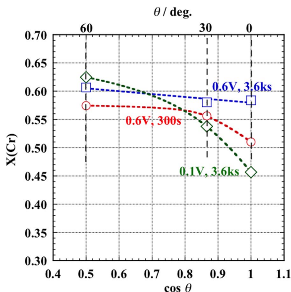
Figure 6. Dependence of the Cr ratio on the angle of detection ( \theta ) of photoelectrons for the passive oxide formed on SUS304 SS at 0.1 V for 3.6 ks, at 0.6 V for 300 s, and at 0.6 V for 3.6 ks in 0.1 M \text{H}_2\text{SO}_4 solutions.
