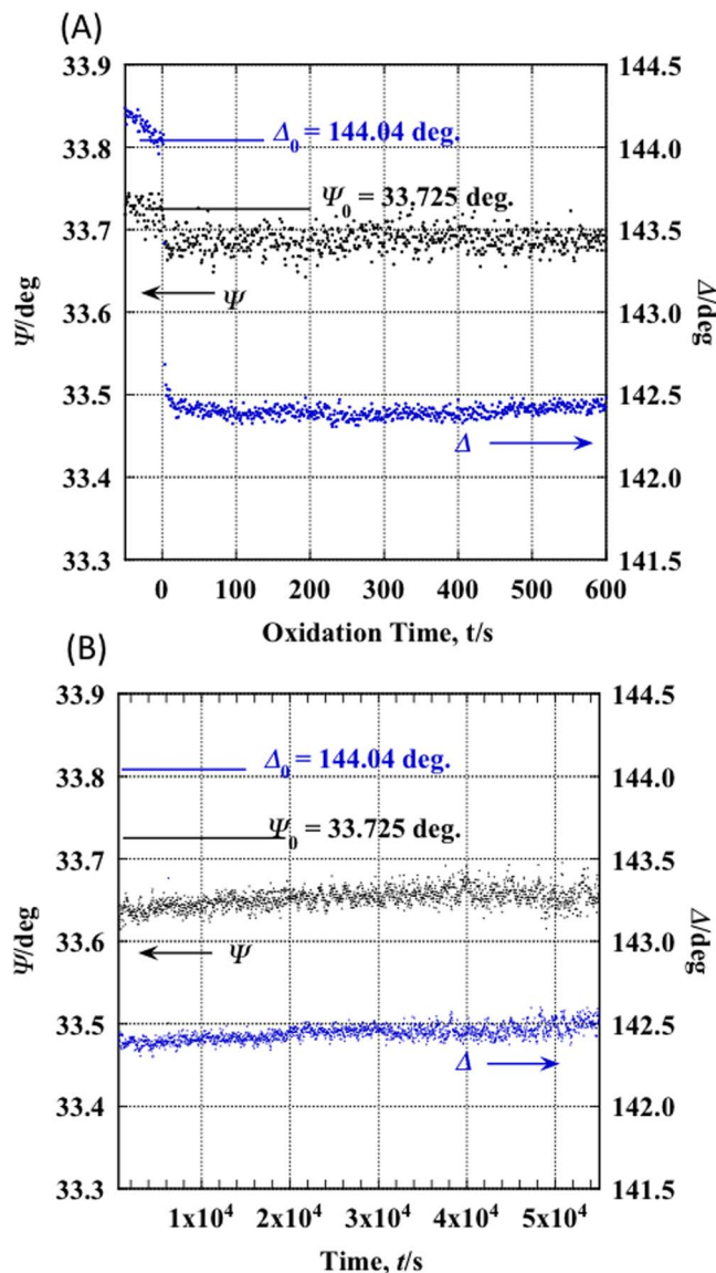
Figure 9. Change in \Psi and \Delta from the initial values at \Psi_0 = 33.725 deg. and \Delta_0 = 144.04 deg. during the oxidation time at a constant potential of 0.6 V, (A) the initial period to 600 s (10 min), and (B) the period from 600 s to 55 ks (15.3 h).
