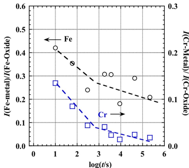
Figure 11. Intensity of the XPS peak of Fe(0) and Cr(0) relative to those of Fe(oxide) and Cr(oxide), respectively, as a function of time.
