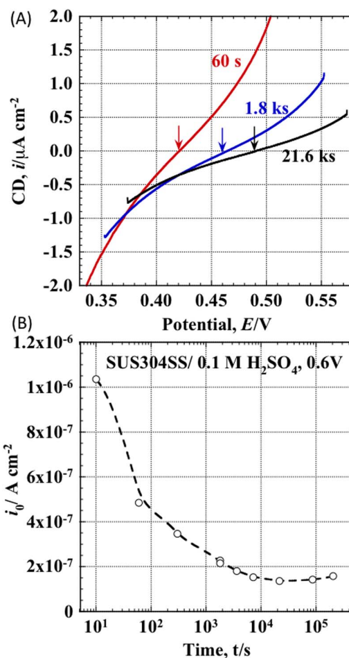
Figure 15. (A) CD as a function of the potential for the \text{Fe}^{3+}/\text{Fe}^{2+} redox reaction on 304 SS passivated at 0.6 V for 60 s, 1.8 ks, and 21.6 ks in a 0.1 M \text{H}_2\text{SO}_4 solution. (B) Exchange CD for the \text{Fe}^{3+}/\text{Fe}^{2+} redox reaction on 304 SS passivated at 0.6 V for various times.
