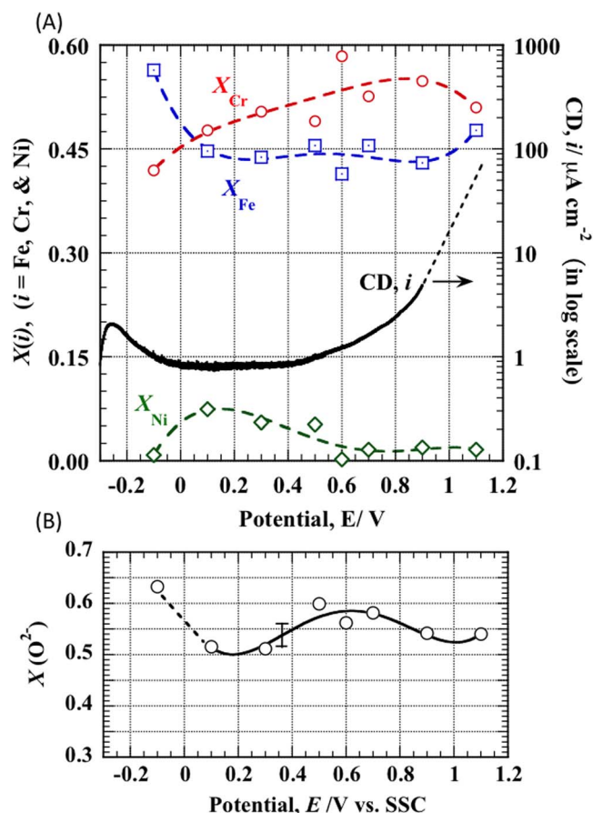
Figure 4. (A) Molar ratios of the Fe, Cr, and Ni cations and (B) molar ratio of \text{O}^{2-} to (\text{O}^{2-} + \text{OH}^-) in the passive oxide formed on SUS304 SS at various potentials in a 0.1 M \text{H}_2\text{SO}_4 solution. In Fig. (A), the log of CD as a function of potential was plotted with the data reported in Fig. 1.
