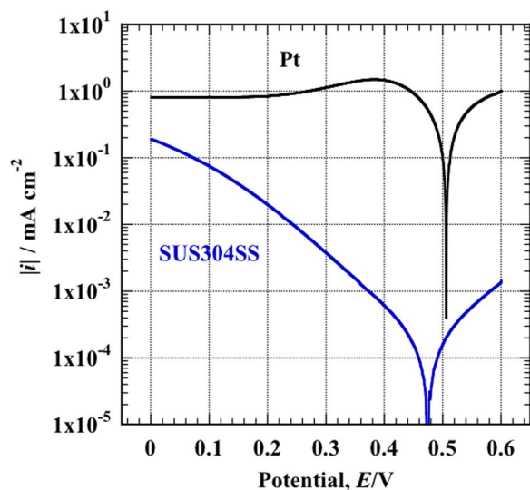
Figure 14. CD on a logarithmic scale as a function of the potential for the \text{Fe}^{3+}/\text{Fe}^{2+} redox reaction on SUS304 SS passivated at 0.6 V for 1 h in a 0.1 M \text{H}_2\text{SO}_4 solution. For comparison, the CD as a function of the potential on the Pt electrode was plotted. The sweep rate of the potential was 2 \text{ mV s}^{-1} .
