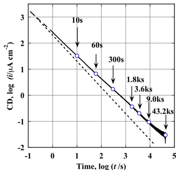
Figure 7. Decay of the current density under constant potential control at 0.6 V vs. SSC in a 0.1 M \text{H}_2\text{SO}_4 solution. The dashed line indicates the d(\log i)/d(\log t) = -1 relationship.
