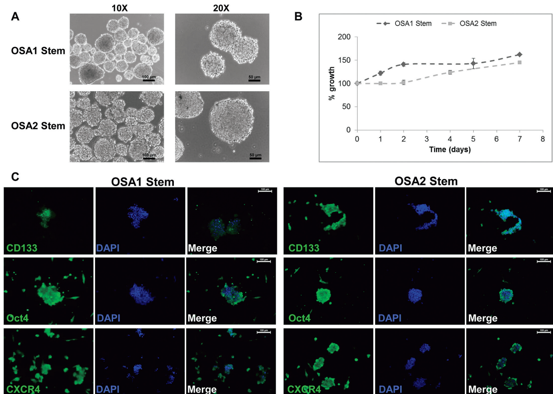
Fig. 2. A. Phase-contrast microphotographs of spheroids formed by OSA stem-like cells. Representative images of stem-enriched cultures (sarcospheres) obtained by shifting primary cultures into selective stem culture medium. Magnification 10X and 20X. B. Growth curves of OSA1 and OSA2 stem-like cells. Cell viability was assessed by MTT assay, at different time-points. Data are shown as mean \pm SE from three separate experiments. C. Analysis of the expression of CD133, Oct4 and CXCR4 in OSA stem-like cells by fluorescence microscopy. Photomicrographs represent marker-positive cells (green), DAPI counterstained nuclei (blue) and merged images. Magnification 20X. Scale bar = 100 \mu m.
