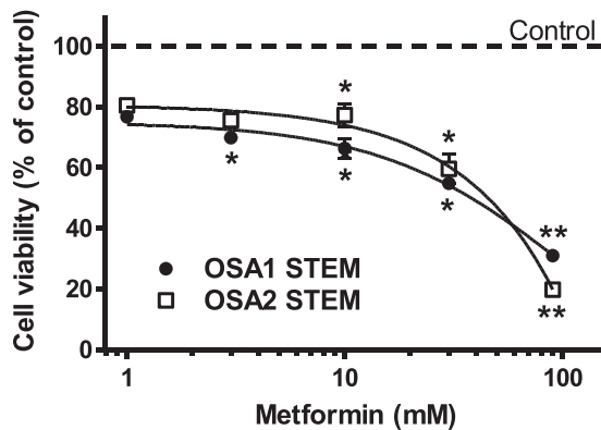
Fig. 5. Dose-response curves of OSA stem-like cells treated with metformin. Metformin exerts antiproliferative effects in cancer stem-like cells derived from OSA1 and OSA2 in a dose-dependent manner. Cells were plated in 48-well plates and treated for 48 h with increasing concentrations (1–90 mM) of metformin. Respective untreated controls are set as 100% and depicted as a broken line. Concentration is reported in a log scale and results, expressed as percentage \pm SEM, are reported as means from triplicates. * p < 0.05 , ** p < 0.01 , vs. untreated cells.
