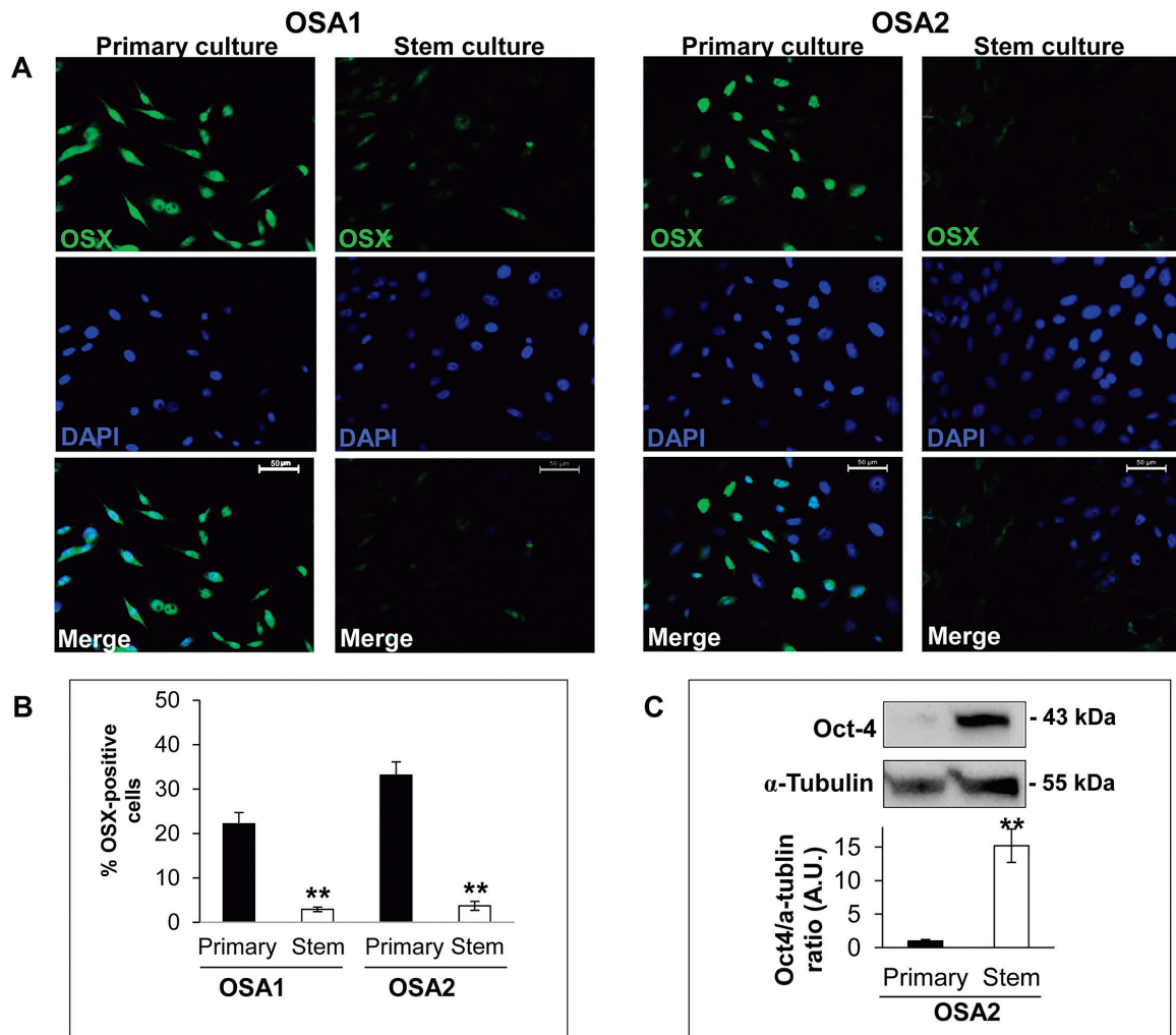
Fig. 4. A. Analysis of the expression of osterix (OSX) in OSA primary cultures and stem-like cells by fluorescence microscopy. Photomicrographs represent marker-positive cells (green), DAPI counterstained nuclei (blue) and merged images. Magnification 40X. Scale bar = 50 \mu m. B. OSX expression in OSA primary cultures and stem-like cells. The percentage of OSX expressing cells was determined by the number of nuclear immunopositive cells among the total number of counted DAPI-stained tumor cells (a minimum of 500 cells were counted per coverlips). A significant decrease in OSX-positive cells was observed in OSA stem cultures, compared to the respective primary cultures. (**p < 0.01). C. Western Blot analysis of Oct4 protein in OSA2 primary culture and stem-like cells. The histogram shows the quantitative densitometric analysis of Oct4 protein (normalized to \alpha -tubulin) and reported as arbitrary units (A.U.), **p < 0.01, vs. primary culture set at 1 A.U..
