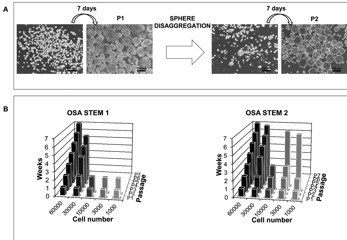
Fig. 3. A. Sphere-forming protocol. Figure depicts cell plating (time 0), and formation of primary spheres, followed by subsequent passages (P1, P2, ...) to obtain secondary spheres, repeated every 7–14 days. B. Sphere formation and self-renewal ability of OSA1 and OSA2 stem cells. Histograms represent the number of passages (sphere disaggregation/replating as single cells) throughout time (for up to 7 weeks), and their relationships to sphere-formation time intervals. The number of primary (P1), secondary (P2, generated from dissociated primary spheres), tertiary (P3, generated from dissociated secondary spheres) and subsequent (up to P7) sphere passages, obtained from different number of cells is shown.
