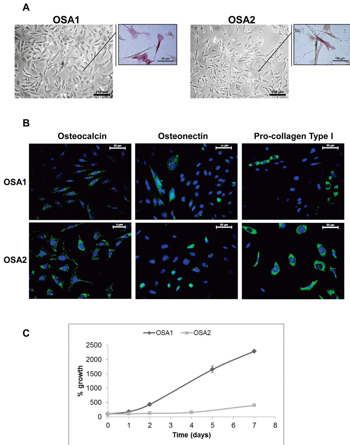
Fig. 1. A. Phase-contrast microphotographs of OSA primary cultures. Representative morphological appearance of canine primary OSA monolayers in FBS-containing medium. Magnification 10X. Inserts show the alkaline phosphatase staining of cells. B. Analysis of the expression of osteonectin, osteocalcin and type I procollagen in OSA primary cultures by fluorescence microscopy. Photomicrographs represent merged images (marker-positive, green; DAPI counterstained nuclei, blue). Magnification 40X. Scale bar = 50 µm. C. Growth curves of OSA1 and OSA2 primary cell cultures. Cell viability was assessed by MTT assay, at different time-points. Data are shown as mean \pm SE from three separate experiments.
