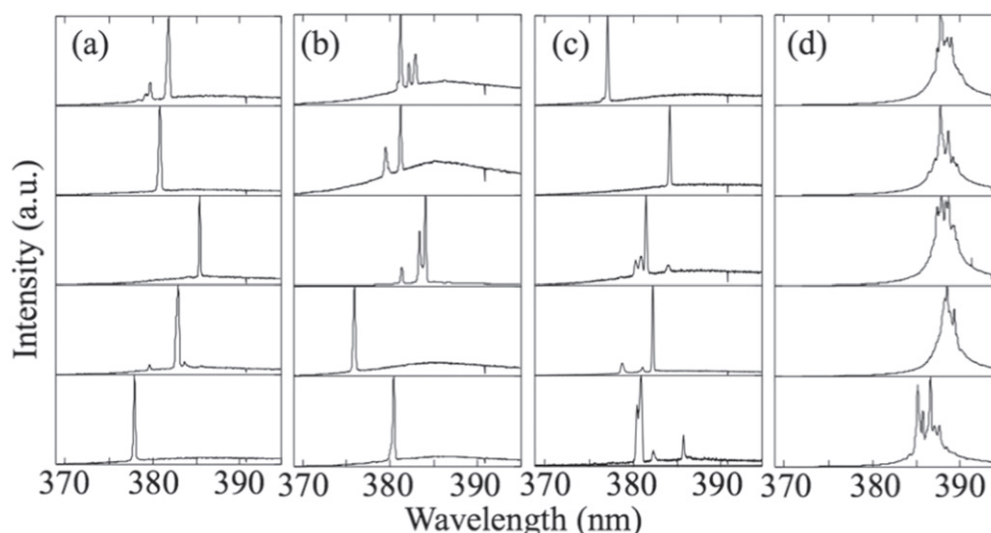
Figure 2. Typical lasing emission spectra at different defect sites. The defect particle sizes are (a) 300, (b) 900 and (c) 2000 nm, respectively. (d) Emission spectra at defect-free sites. Each spectrum was normalized by its maximum intensity.
