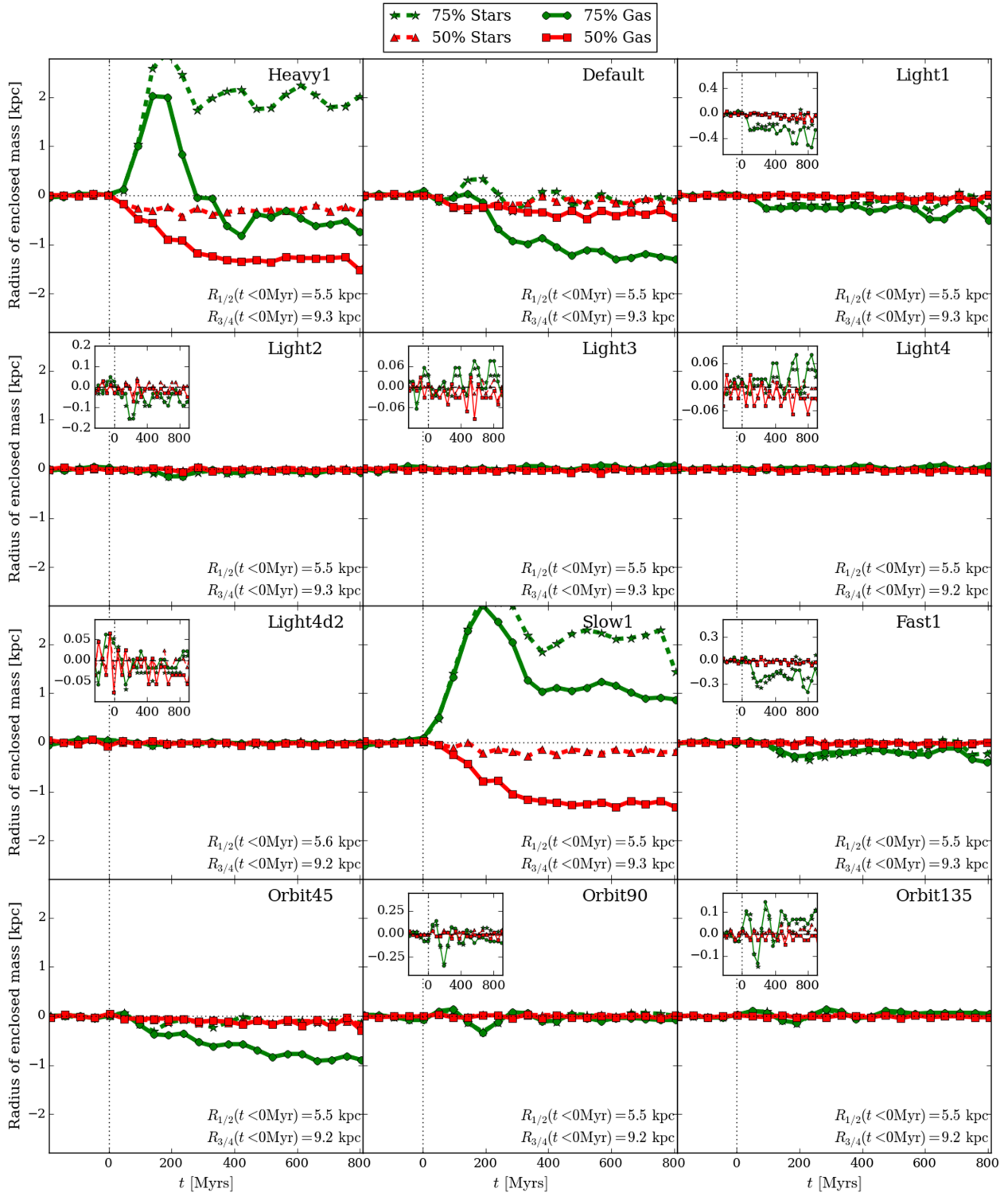
Figure 19. The evolution of the radius which encloses half ( R_{1/2} , red lines) or three-quarters ( R_{3/4} , green lines) of the total mass of stars (dashed lines) and gas in each of our main models (solid lines). The 0 Myr time corresponds to the time of closest approach of the companion. Radii are measured as offsets from the average value prior to the companion passage, with values given in the lower-right corner. All radii are shown to the same scale, with the inserts showing a zoom in of the same data for simulations where the response is small.
