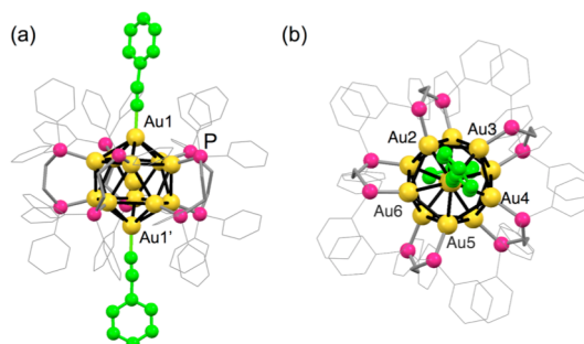
Fig. 1 (a) Side and (b) top views of the crystal structure of cationic moiety of 2 ·(PF 6 ) 3 . Phenylethynyl units (C \equiv CPh) are highlighted in light green and hydrogen atoms are omitted for clarity.
