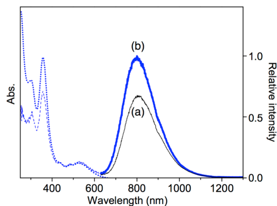
Fig. 5 Photoluminescence spectra of (a) 1 ·(PF 6 ) 3 ( \lambda_{\text{ex}} = 495 nm) and (b) 2 ·(PF 6 ) 3 ( \lambda_{\text{ex}} = 525 nm) in MeCN at 25 °C (absorbance at \lambda_{\text{ex}} = 0.1). Absorption (dotted) and excitation spectra ( \lambda_{\text{em}} = 800 nm; dashed) of 2 ·(PF 6 ) 3 are also provided for comparison.
