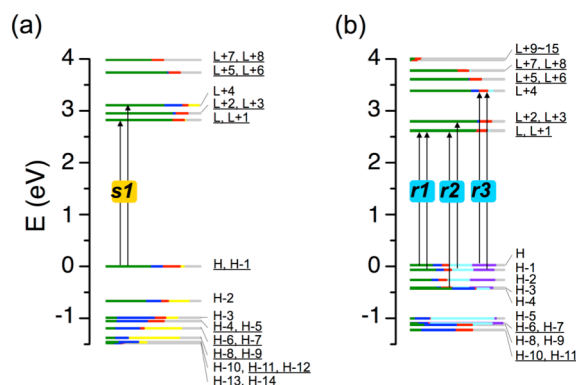
Fig. 3 Kohn–Sham (KS) orbital energy level diagrams of (a) 1 and (b) 2 . Each KS orbital energy is relative to the HOMO energy and is drawn to indicate the relative contributions (line lengths with color labels) of the atomic orbitals of Au (6sp) in green, Au (5d) in blue, P (3p) in red, Cl (3p) in yellow, C (2p) for C \equiv C and Ph of C \equiv CPh units in light blue and violet, respectively, and miscellaneous in gray. H – X and L + Y represent HOMO – X and LUMO + Y, respectively. Underlines indicate the degeneracies of energy levels.
