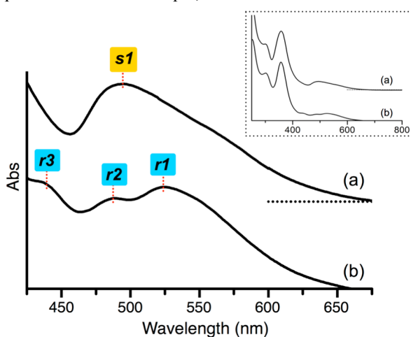
Fig. 2 Visible absorption spectra of (a) 1 ·(PF 6 ) 3 and (b) 2 ·(PF 6 ) 3 in MeCN at 25 °C. Inset shows the spectra over the whole measurement region.
