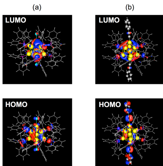
Fig. 4 HOMOs and LUMOs of (a) 1 and (b) 2 .
