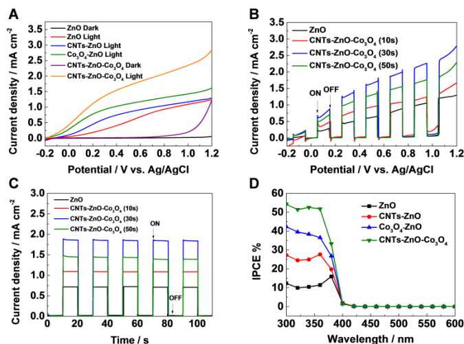
Figure 5. (A) Current-voltage curves of pristine ZnO NWs, binary CNTs-ZnO ( 0.25 \text{ mg mL}^{-1} ) NWs, \text{Co}_3\text{O}_4 -ZnO (30 s) NWs and ternary CNTs-ZnO- \text{Co}_3\text{O}_4 (30 s) NWs; (B) current-voltage curves of pristine ZnO NWs and ternary CNTs-ZnO- \text{Co}_3\text{O}_4 NWs under chopped light illumination; (C) amperometric I-t curves of pristine ZnO NWs and ternary CNTs-ZnO- \text{Co}_3\text{O}_4 NWs measured at 0.6 \text{ V} ; (D) IPCE spectra of pristine ZnO NWs, binary CNTs-ZnO NWs, \text{Co}_3\text{O}_4 -ZnO NWs and ternary CNTs-ZnO- \text{Co}_3\text{O}_4 NWs at 0.6 \text{ V} vs. Ag/AgCl.
