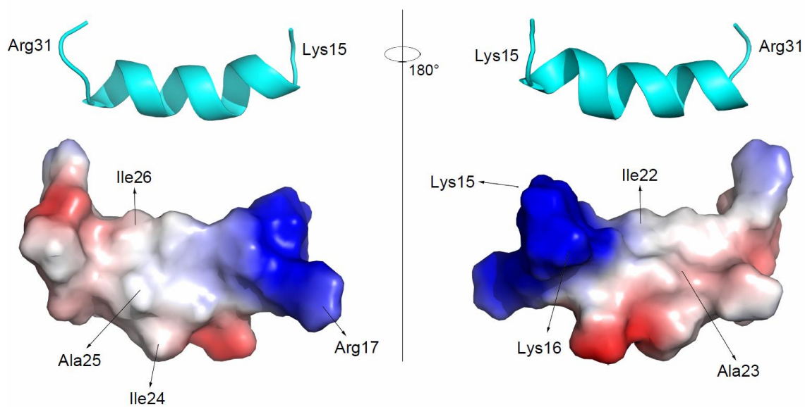
Figure 6. Representative ribbon conformations (upper) and electrostatic surface potentials (lower) of the LPS-bound CP1 (Lys15–Arg31) structure generated by PyMOL, where the positive potentials are drawn in blue, and the negative potentials are drawn in red.
