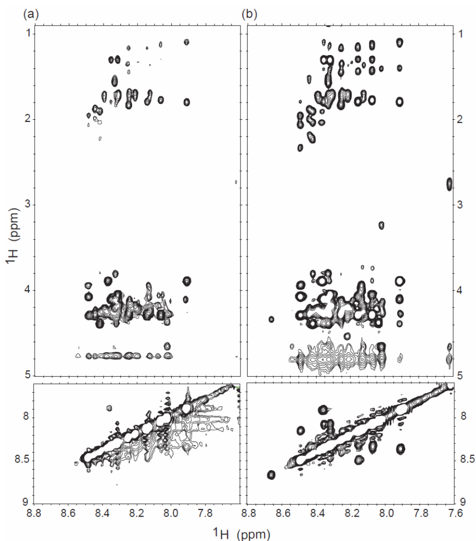
Figure 2. Two-dimensional NOESY spectra of CP1 with/without LPS. The fingerprint region and amide region of the NOESY spectra of CP1 showing HN-H \alpha , HN-HN, and HN side-chain resonances. (a) NOESY spectrum of CP1 in the absence of LPS and (b) the Tr-NOESY spectrum of CP1 in the presence of LPS showed a significant number of NOE cross-peaks compared with those in the free state. The Tr-NOESY spectra of CP1 were acquired in the presence of 50 \mu M LPS. Tr-NOESY experiments were carried out at 600 MHz and 298 K, with a mixing time of 150 ms.
