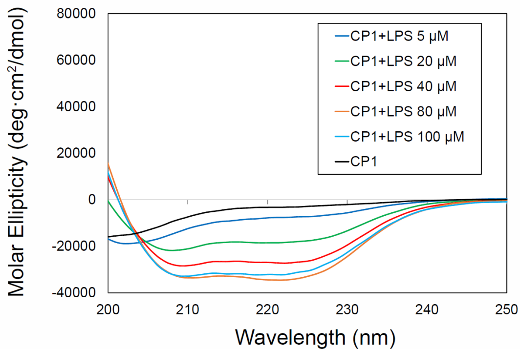
Figure 1. Secondary structures of 20 \mu M CP1 in free and LPS-bound forms, as determined by CD spectroscopy. CD spectra of CP1 were obtained at various concentrations of LPS (0, 5, 20, 40, 80, and 100 \mu M) from E. coli O111:B4 in 10 mM sodium phosphate (pH 6.0).
