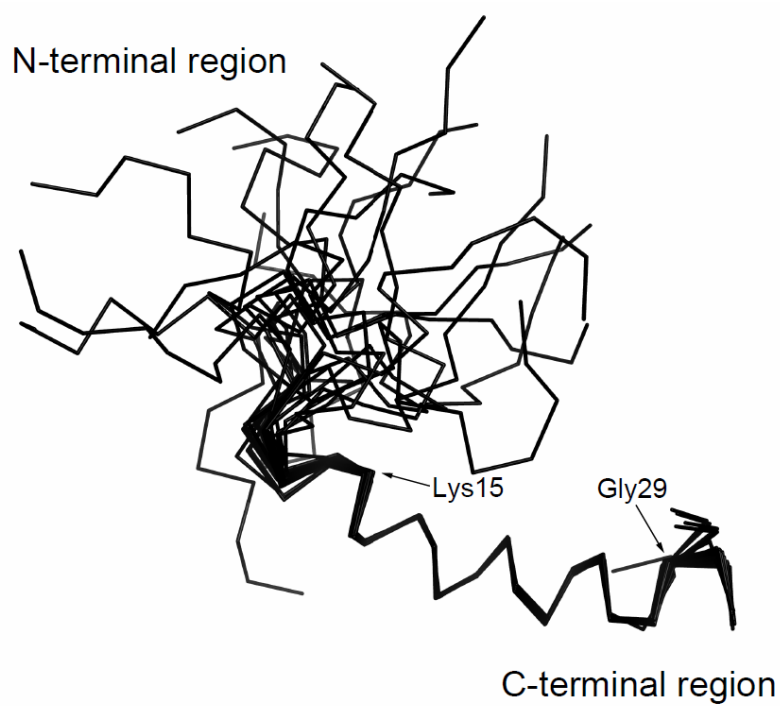
Figure 5. Backbone traces of the 20 lowest energy structures of CP1 bound to LPS, obtained from CYANA. CP1 in the LPS-bound state exhibits an \alpha -helix structure along the residues from Lys15 to Gly29 in the C-terminal region.
