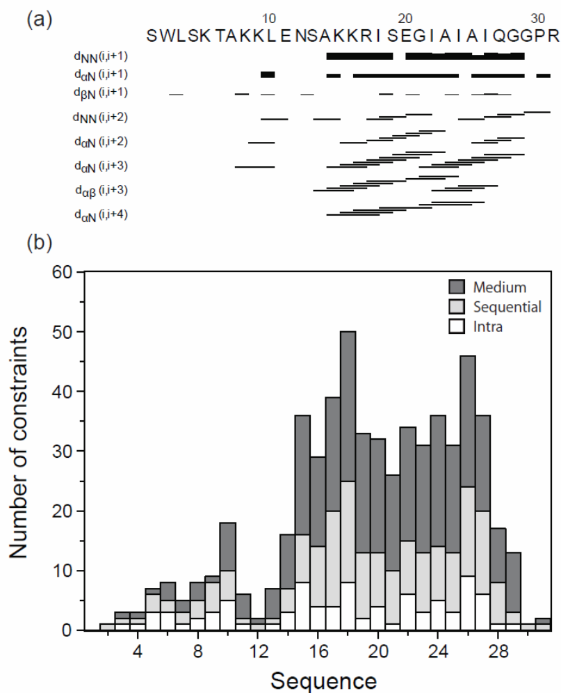
Figure 4. Summary of NMR structural parameters of CP1 in LPS micelles. (a) Bar diagram showing sequential and medium range NOEs of CP1 in the presence of LPS. The thickness of the bars indicates the intensity of the peaks, which are assigned as strong, medium, and weak. The amino acid sequence of CP1 is shown at the top. (b) A histogram showing the number of Tr-NOEs of CP1 as a function of residue number in complex with LPS micelles.
