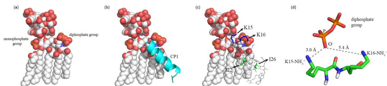
Figure 7. (a) LPS structure used in the docking calculation (PDB ID 1QFG). (b, c) The complex structure of CP1 and LPS. CP1 is shown as a cartoon (b) and sticks (c). (d) The distance between Lys15-NH 3 + /Lys16-NH 3 + and phosphate group. The docking model was calculated by using the model structure of CP1 in its LPS-bound state and the crystal structure of LPS.
