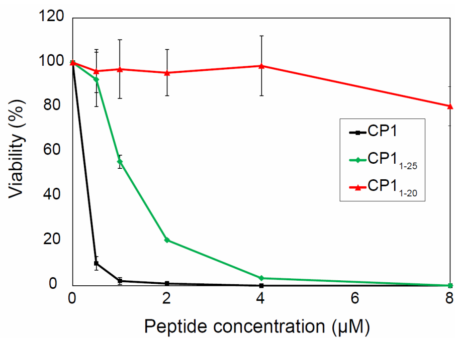
Figure 8. Viability of bacteria ( E. coli ML35) exposed to different concentrations of CP1 and its analogs CP1 1-25 and CP1 1-20 .
