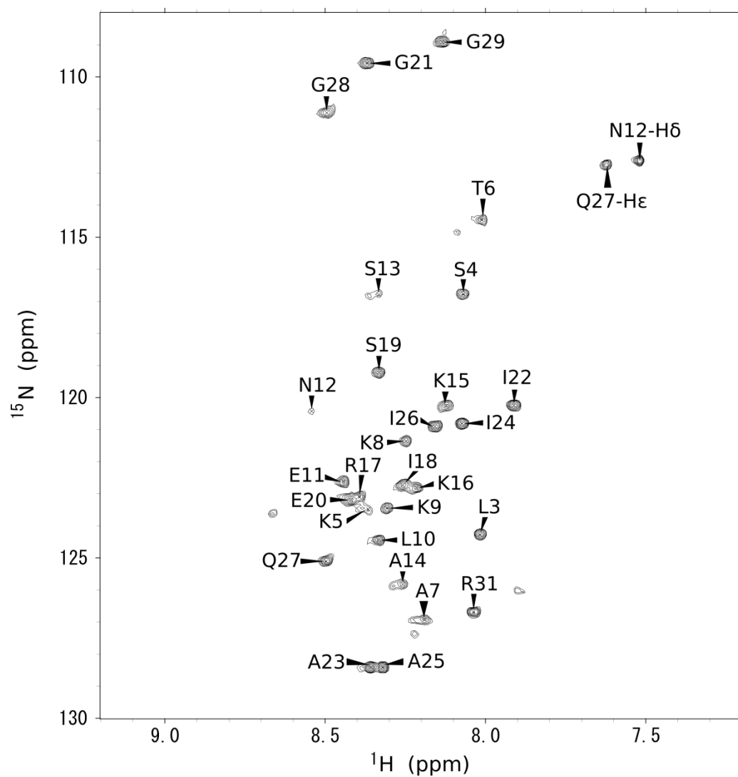
Figure 3. ^1\text{H} - ^{15}\text{N} HSQC 600 MHz NMR spectrum of CP1 at pH 5.0 and 298 K. The spectrum showed excellent chemical shift dispersion, indicating a single species with no evidence of heterogeneity.
