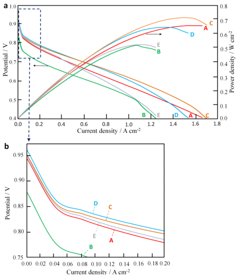
Fig. 2.4 Comparison of unit cell performance between current-voltage curves of electrodes and power density curves of electrodes with prepared and commercial catalysts as respective anode electrocatalyst: (a) full range (b) zoom at activity loss range: (A) Pt 2 Ru 3 /C commercial catalyst, (B) Pt 2 Ru 3 /RC1000ac0, (C) Pt 2 Ru 3 /RC1000ac37, (D) Pt 2 Ru 3 /RC1000ac58, and (E) Pt 2 Ru 3 /RC1000ac88.
