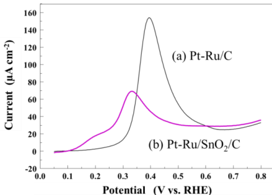
Fig. 5.4 CO stripping voltammetry at 60 °C for (a) PtRu/C and (b) PtRu/SnO 2 /C. CO was (1) fed for 20 min at 0.05 V in 0.1 M HClO 4 ; (2) purged for 30 min; and (3) swept at 60 °C between 0.05 V and 0.8 V at 10 mV/s.
