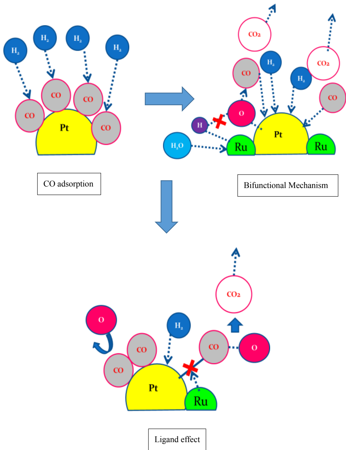
Fig. 1.3 CO adsorption and removal by the bifunctional mechanism and ligand effects.
