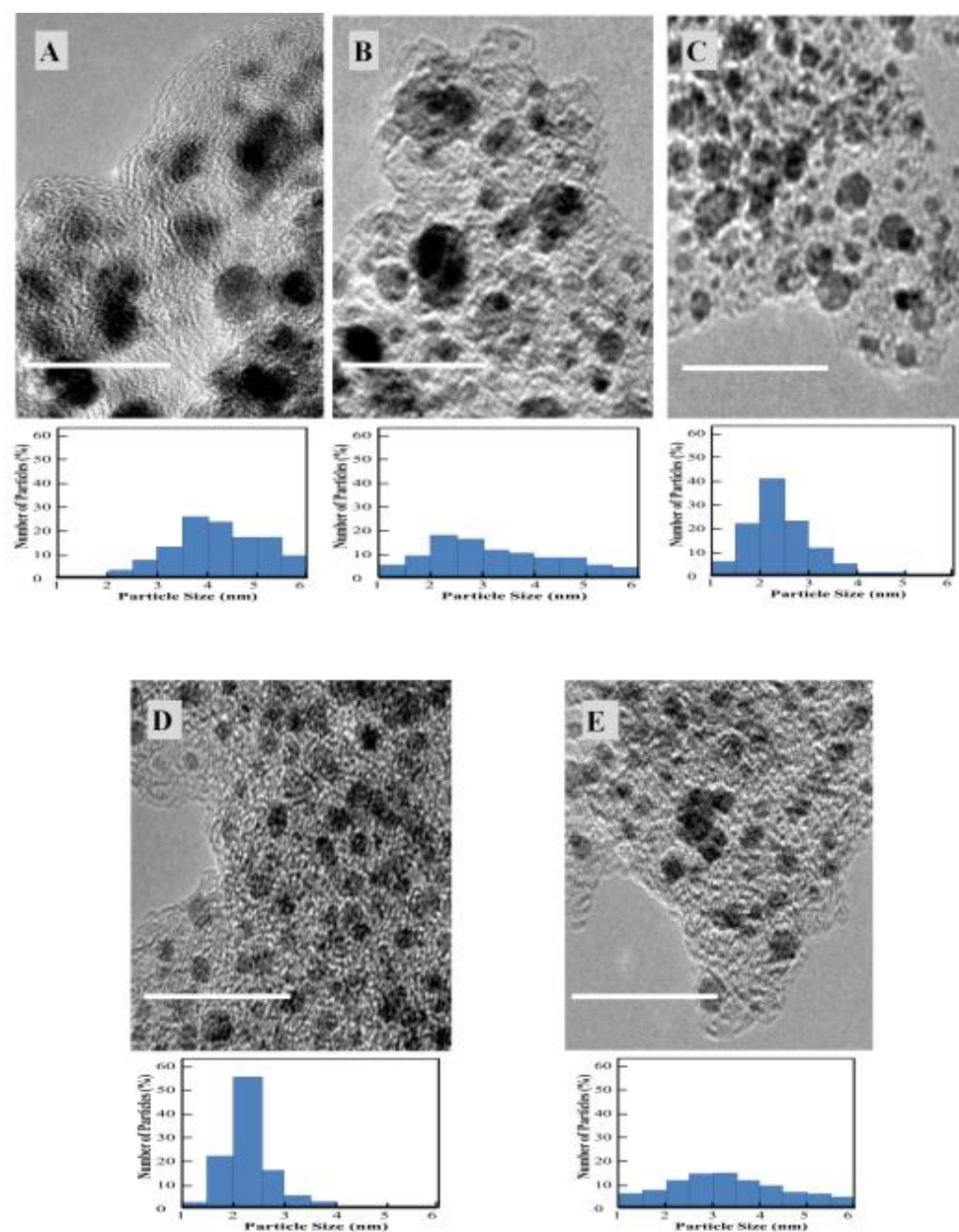
Fig. 2.3 TEM micrograph: (A) Pt 2 Ru 3 /C commercial catalyst, (B) Pt 2 Ru 3 /RC1000ac0, (C) Pt 2 Ru 3 /RC1000ac37, (D) Pt 2 Ru 3 /RC1000ac58, and (E) Pt 2 Ru 3 /RC1000ac88 at scale bars = 20 nm.
