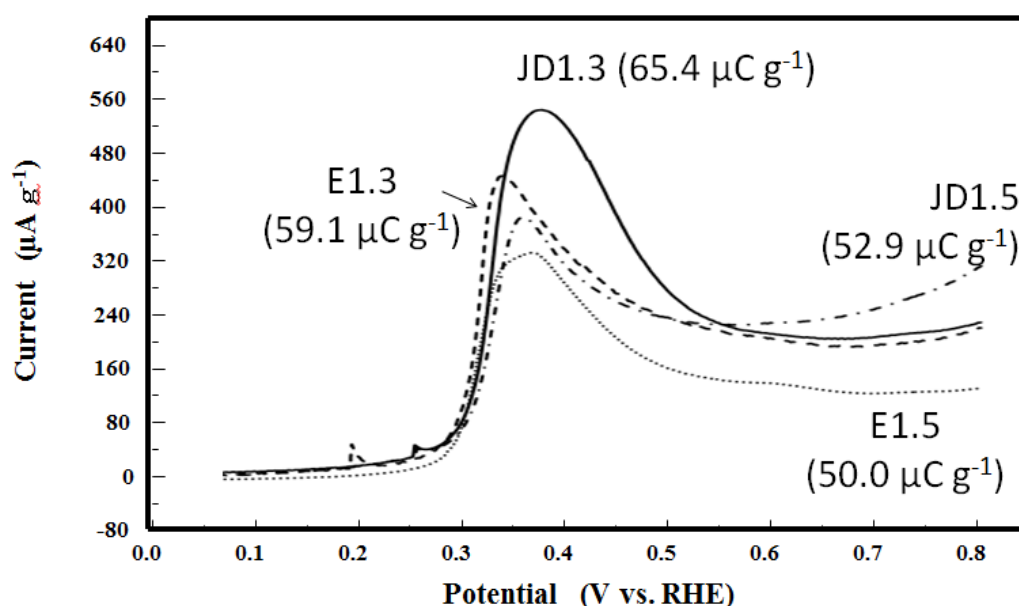
Fig. 3.7 CO stripping results for E1.3, E1.5, JD1.3 and JD1.5 catalysts recorded during potential cycling with 10 \text{ mV s}^{-1} from 0.05 V to 1.2 V vs RHE in 75 mL of 0.1 M \text{HClO}_4 at 25^\circ\text{C} . Prior to the measurement, \text{HClO}_4 solution was cleaned by Ar gas flow for 15 min and then CV measurement between the above-mentioned potentials was performed for 10 cycles with a scan speed of 50 \text{ mV s}^{-1} . Then CO gas was introduced into the system for 10 min to let CO adsorb on the catalysts and then the solution was purged with Ar gas for 15 min. The potential during CO adsorption and Ar purging was kept constant at 0.1 V vs RHE. In all cases the gas flow rates were 200 \text{ mL min}^{-1} .
