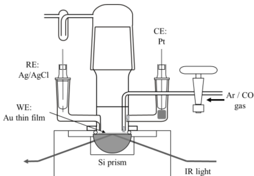
Fig. 5.1 Schematic diagram of surface-enhanced infrared absorption spectroscopy (SEIRAS) glass cell.
