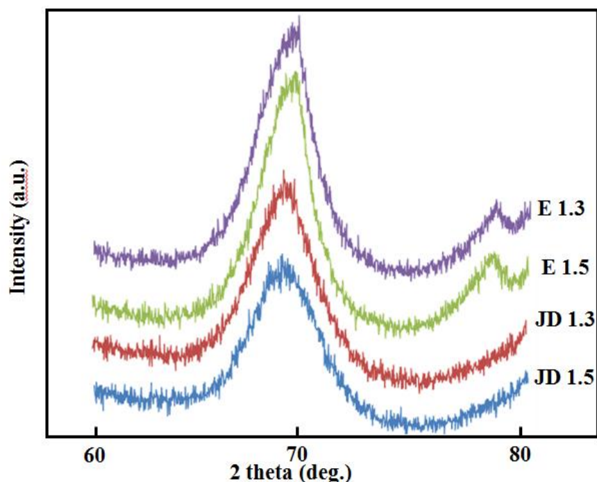
Fig. 3.2 XRD patterns of E1.3, E1.5, JD1.3 and JD1.5 catalysts.
