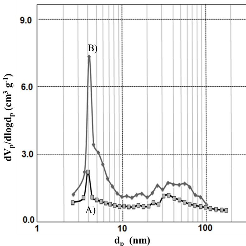
Fig. 3.1 Pore size distribution of A) ECP300J and B) ECP600JD.
