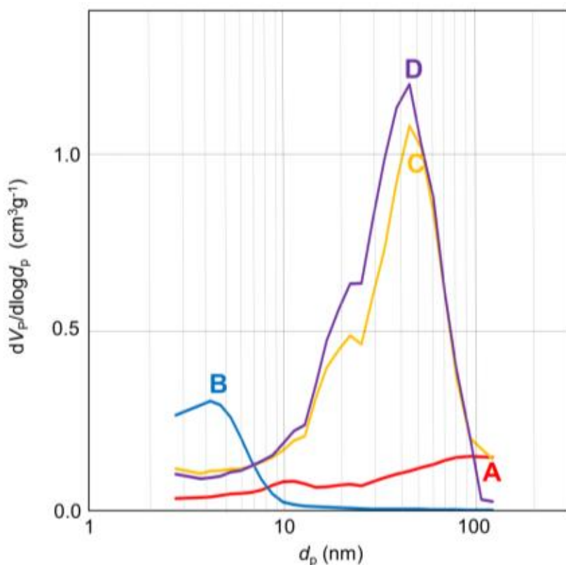
Fig. 4.5 Pore size distribution of all Pt 2 Ru 3 catalysts after mixing of Nafion ® : (A) Pt 2 Ru 3 /C commercial catalyst, (B) Pt 2 Ru 3 /RC200ac58, (C) Pt 2 Ru 3 /RC800ac58, and (D) Pt 2 Ru 3 /RC1000ac58.
