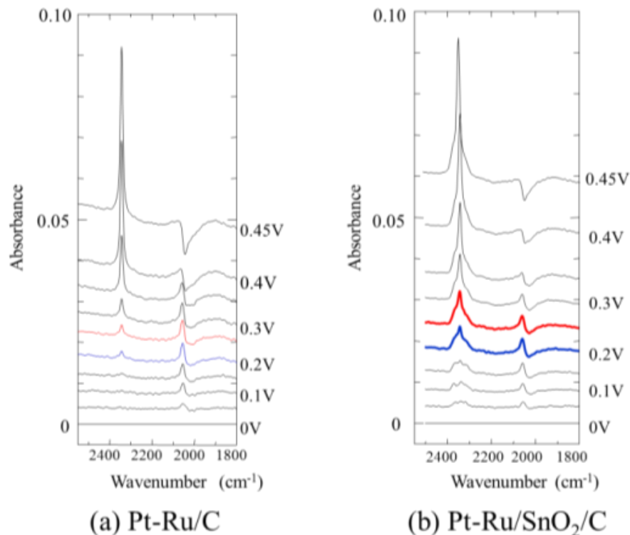
Fig. 5.5 IRRAS spectra of (a) PtRu/C and (b) PtRu/SnO 2 /C deposited on a gold substrate surface CO was (1) fed for 20 min at 0 V in 0.1 M HClO 4 ; (2) purged for 35 min; (3) the electrode was pushed onto the CaF 2 prism window with the thin-layer geometry; the in situ IR spectra were recorded with a scan rate of 0.25 mV/s; 25 interferograms were co-added to each spectrum.
