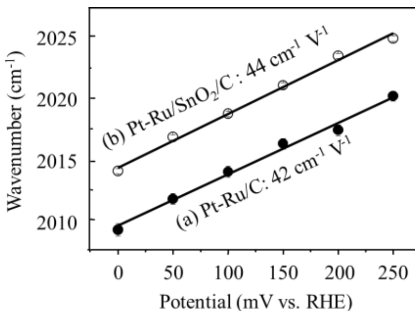
Fig. 5.7 The CO stretching peak frequency vs. potential for (a) PtRu/C and (b) PtRu/SnO 2 /C.
