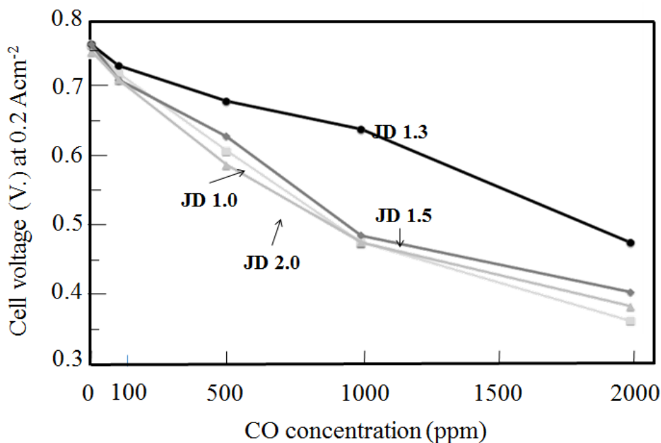
Fig. 3.5 Effect of CO concentration on cell voltage at 0.2 \text{ A cm}^{-2} . Cell temp.: 70^\circ\text{C} , electrolyte: Nafion ® NRE 212, cathode: Pt/C ( 0.5 \text{ mg-Pt cm}^{-2} ), \text{O}_2 humidified at 68^\circ\text{C} , flow rate: 80 \text{ mL min}^{-1} , anode: JDx ( 0.5 \text{ mg-PtRu cm}^{-2} ), \text{H}_2 containing 0 ppm, 100 ppm, 500 ppm, and 2,000 ppm CO humidified at 70^\circ\text{C} , flow rate: 80 \text{ mL min}^{-1} .
