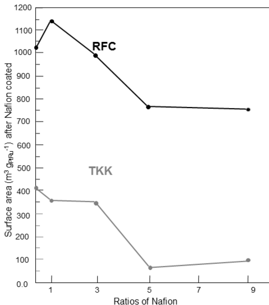
Fig. 6.1 The BET surface area of all catalysts.
