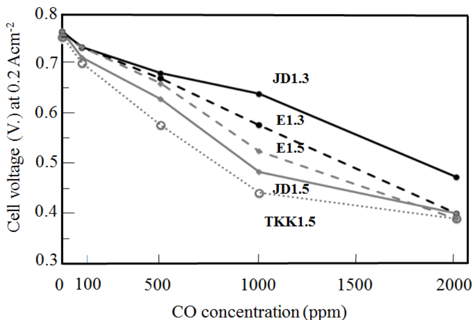
Fig. 3.6 Effect of CO concentration on potential at 0.2 \text{ A cm}^{-2} . Cell temp.: 70^\circ\text{C} , electrolyte: Nafion ® NRE 212, cathode: Pt/C ( 0.5 \text{ mg-Pt cm}^{-2} ), \text{O}_2 humidified at 68^\circ\text{C} , flow rate: 80 \text{ mL min}^{-1} , anode: E1.3, E1.5, JD1.3, JD1.5, and TKK1.5 ( 0.5 \text{ mg-PtRu cm}^{-2} ), \text{H}_2 containing 0 ppm, 100 ppm, 500 ppm, and 2,000 ppm CO humidified at 70^\circ\text{C} , flow rate: 80 \text{ mL min}^{-1} .
