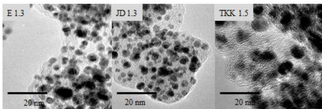
Fig. 3.3 TEM images of E1.3, JD1.3 and TKK1.5 catalysts.
