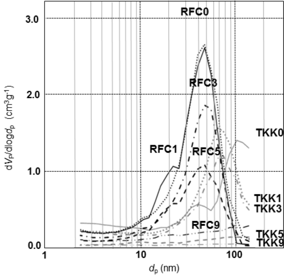
Fig. 6.4 Pore distribution of all catalysts.
