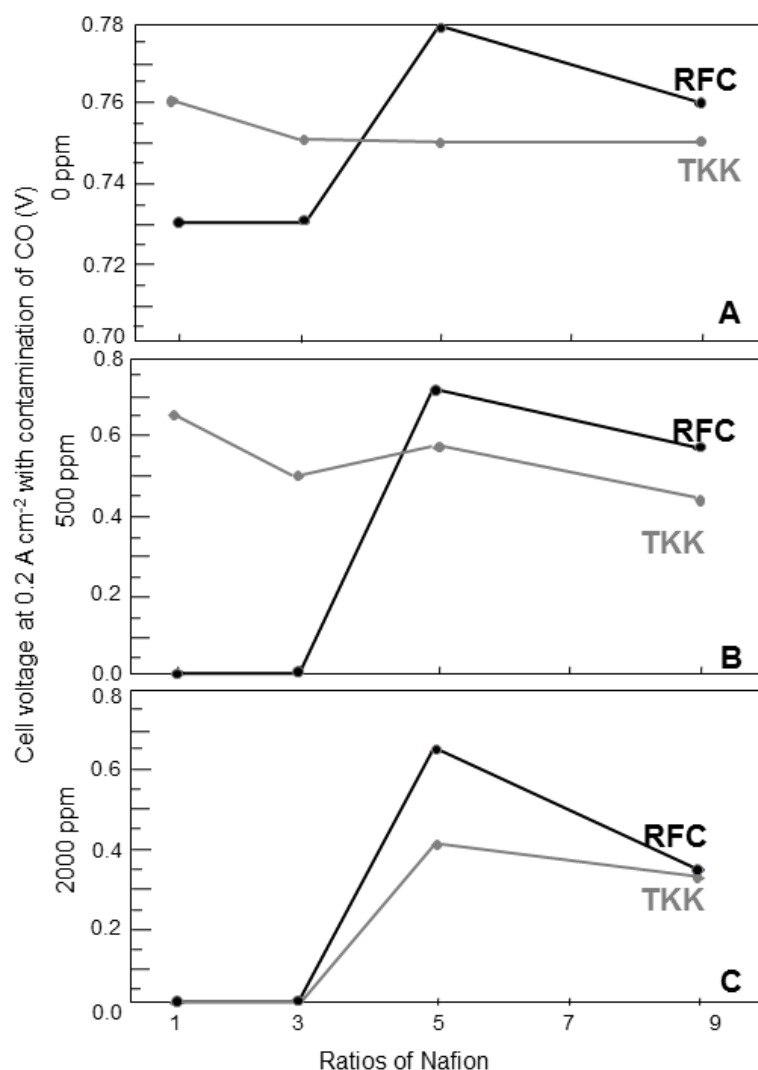
Fig. 6.3 The CO tolerance of Nafion ® mixed catalysts: (A) Pure H 2 , (B) 500 ppm CO/H 2 , and (C) 2,000 ppm CO/H 2 .
