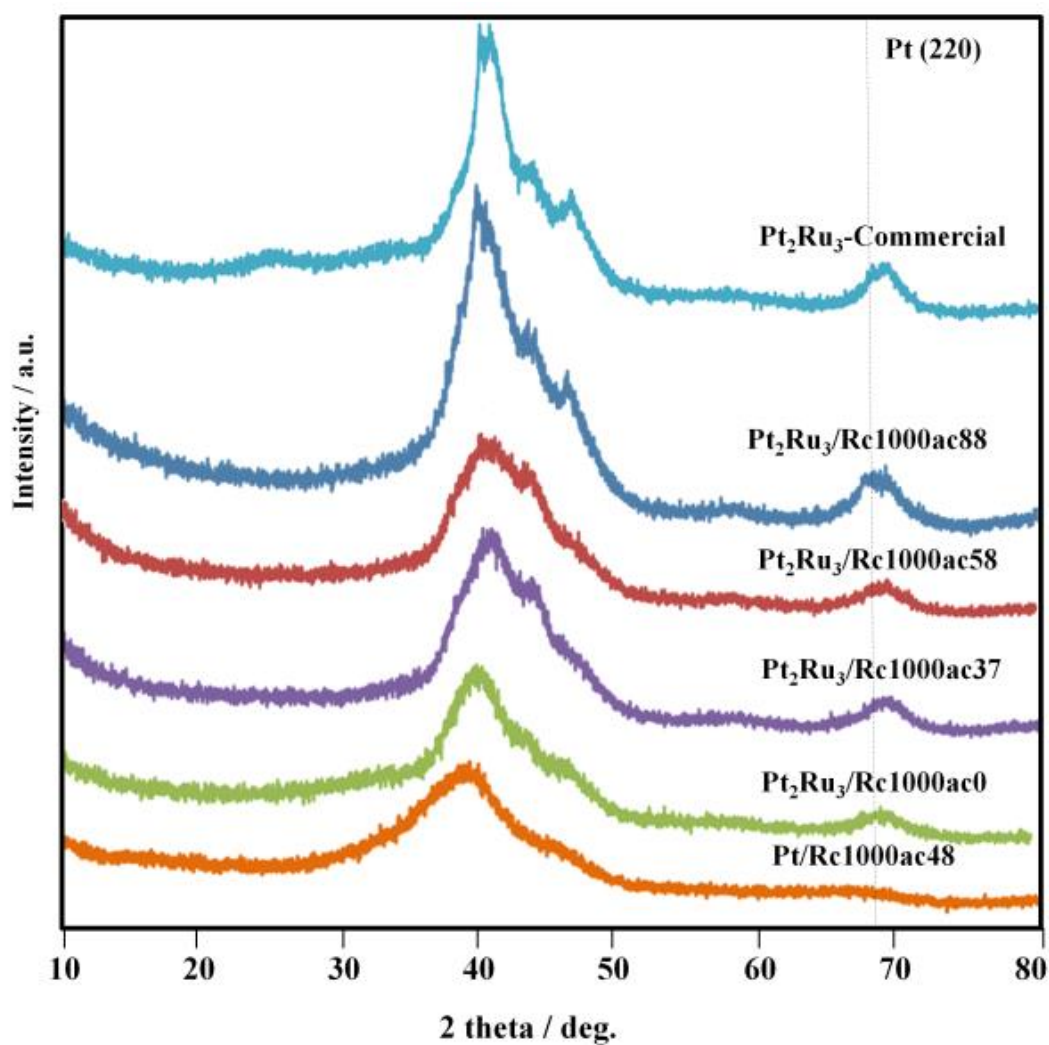
Fig. 2.1 XRD patterns of \text{Pt}_2\text{Ru}_3 -commercial catalyst and prepared catalysts.
