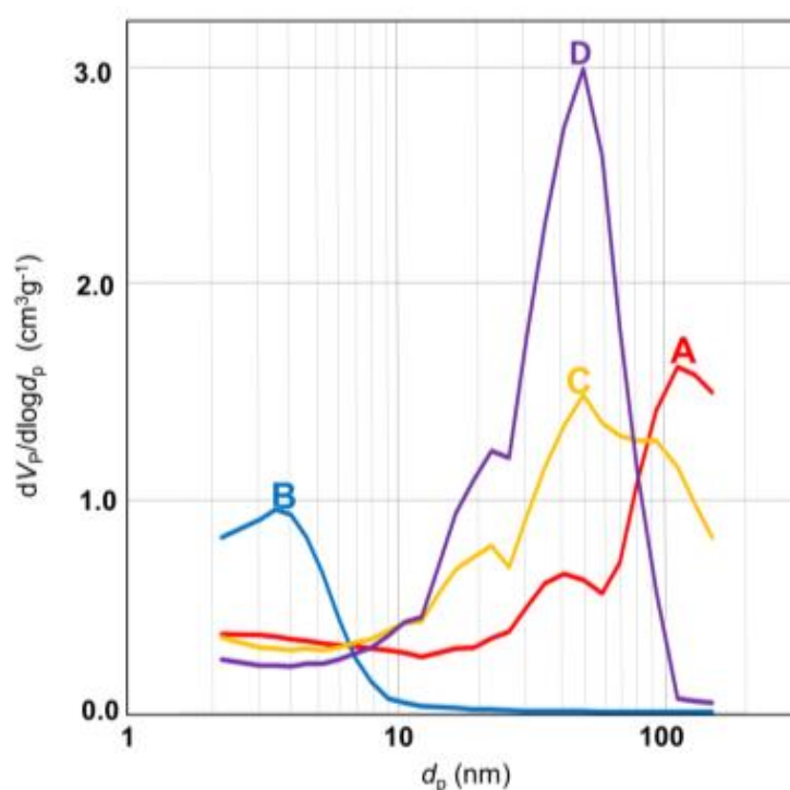
Fig. 4.4 Pore size distribution of all Pt 2 Ru 3 catalysts after deposition of PtRu: (A) Pt 2 Ru 3 /C commercial catalyst, (B) Pt 2 Ru 3 /RC200ac58, (C) Pt 2 Ru 3 /RC800ac58, and (D) Pt 2 Ru 3 /RC1000ac58.
