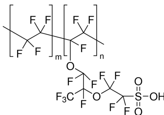
Fig. 1.2 Structure of Nafion ® .
