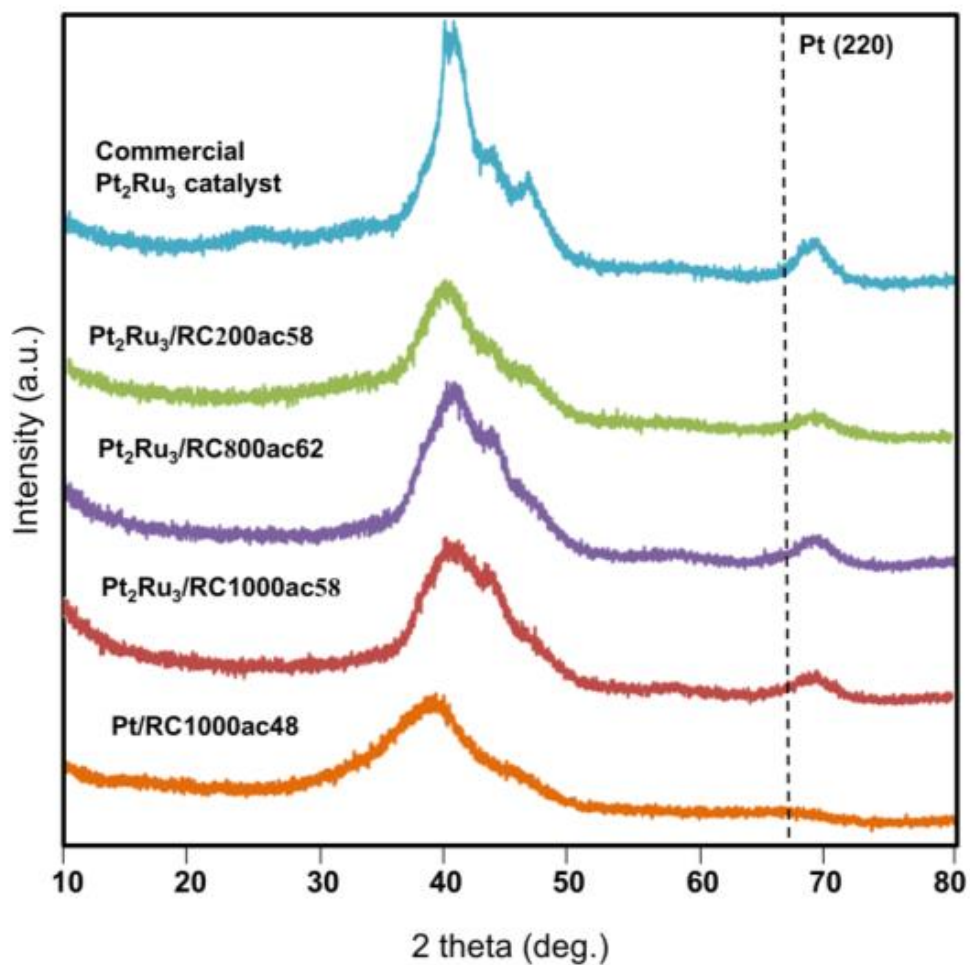
Fig. 4.1 XRD patterns of commercial \text{Pt}_2\text{Ru}_3 catalyst and prepared catalysts.
