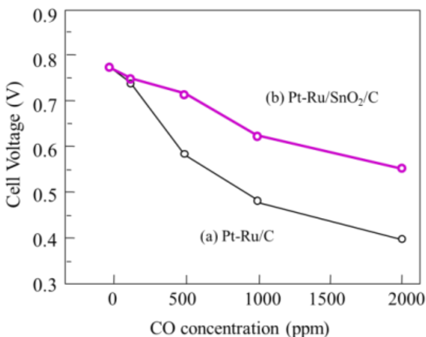
Fig. 5.8 Effect of CO concentration on cell voltage at 0.2 A cm -2 . Cell temp.: 70 °C; electrolyte: Nafion ® NRE 212; cathode: Pt/C (0.5 mg cm -2 ); O 2 humidified at 70 °C; flow rate: 80 mL/min; anode: (a) PtRu/C and (b) PtRu/SnO 2 /C (0.5 mg PtRu cm -2 ); H 2 containing 0-2,000 ppm CO humidified at 70 °C; and flow rate: 80 mL/min.
