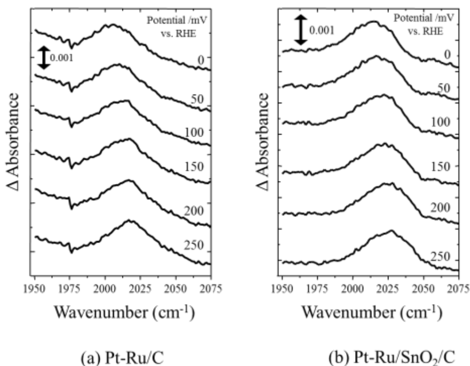
Fig. 5.6 SEIRAS spectra of adsorbed CO as a function of potential on (a) PtRu/C and (b) PtRu/SnO 2 /C in 0.5 M H 2 SO 4 .
