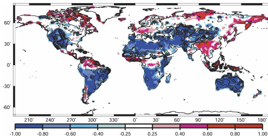
FIG. 6. Same as in Fig. 1, but for JJA mean sensible heat flux and latent heat flux in LND. (Contours show the same values as in Fig. 1b.)
