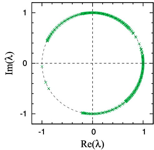
FIG. 8. The eigenvalue \lambda (green crossed) of the time-evolution operator of the nonunitary quantum walk with parameters in Eq. (43) plotted on a complex plain.
