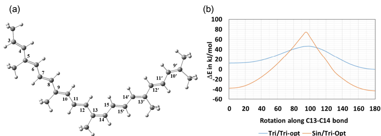
Figure 10. (a) Optimized structure of the 13,14- cis -SPO. (b) Singlet-triplet crossing of the 13,14- cis SPO. Tri/Tri-Opt and Sin/Tri-Opt represent the triplet and singlet energies obtained at the triplet optimized structures.
