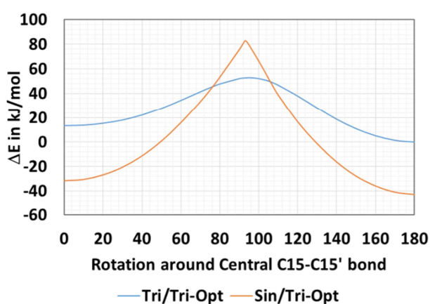
Figure 5. Potential curves for singlet and triplet states of the 15,15'- cis -SPO. Tri/Tri-Opt and Sin/Tri-Opt represents the triplet and singlet energies obtained at the triplet-state optimized structure.
