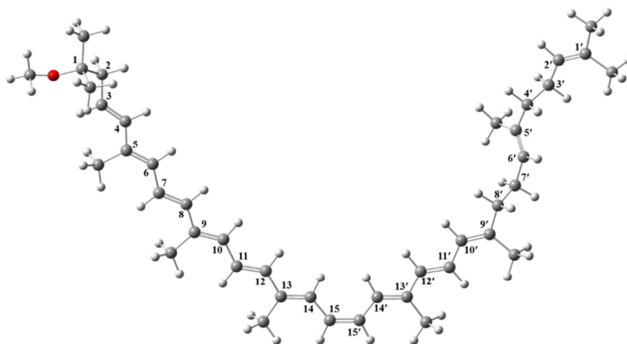
Figure 2. Structure (optimized) with important carbon atom numbering of 15,15'- cis -spheroidene.
