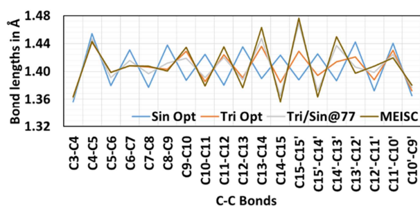
Figure 7. Conjugated C-C bond lengths in singlet, triplet, Singlet-triplet crossing ( \phi_{S-T}=77^\circ ), and MEISC ( \phi=58.4^\circ ) BP86/6-311G(d) optimized structures.
