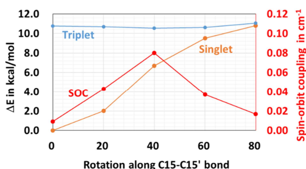
Figure 9. Spin-orbit coupling between the singlet and triplet states of 15,15'- cis -SPO. CASSCF potential energy curves of these two states along the C15-C15' bond twisting.
