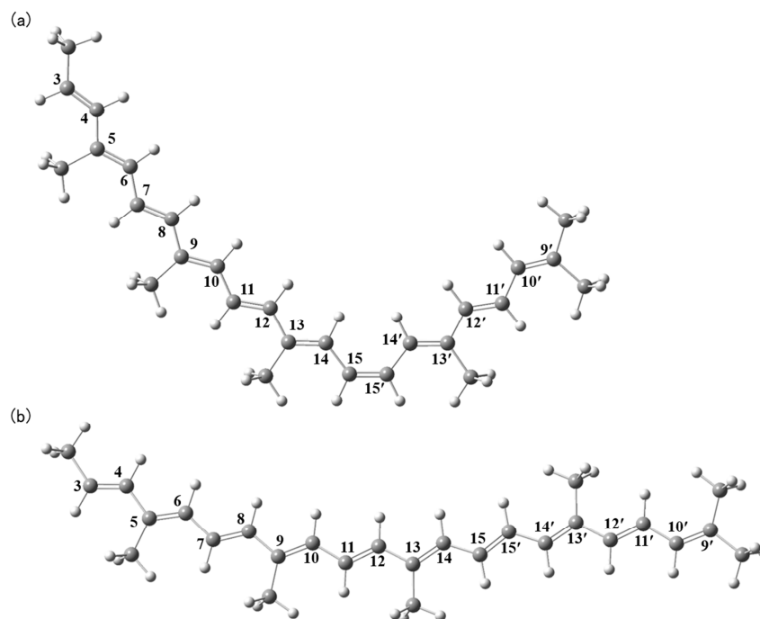
Figure 3. Structure (optimized) of the truncated (a) 15,15'- cis -SPO (b) trans -SPO.
