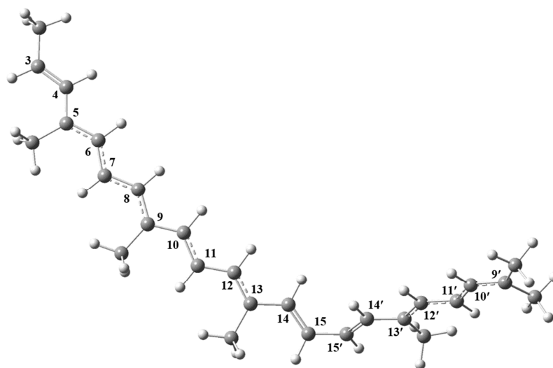
Figure 6. MEISC structure at BP86/6-311G( d ).
