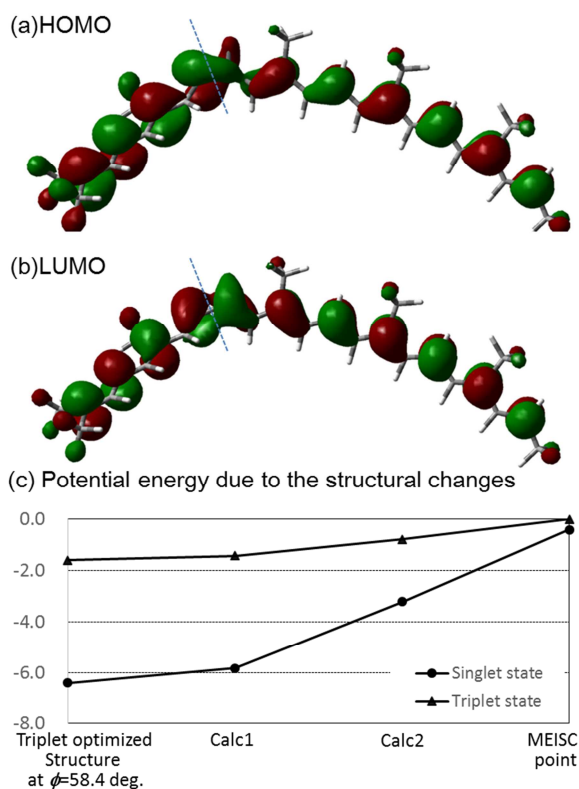
Figure 8 (a) HOMO and (b) LUMO distributions at the MEISC point structure. The twisted C15-C15' bond was shown by dotted lines. (c) Effect of bond lengths on potential energy of the singlet and triplet states. “Calc1” denotes that only the C15-C15' length was changed to that of the MEISC structure while “Calc2” denotes all the conjugated C-C bond lengths were changed.
