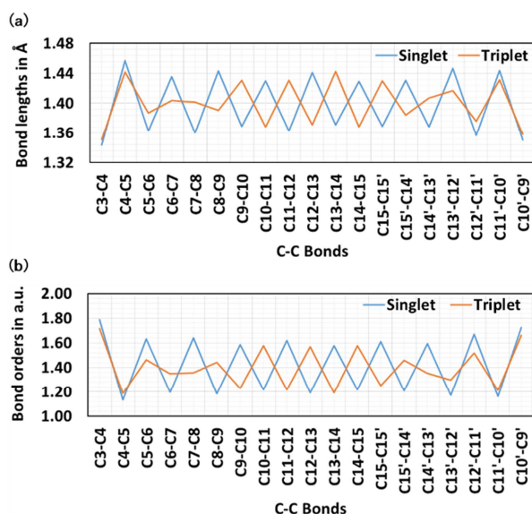
Figure 4. Conjugated (a) bond lengths and (b) bond orders in ground and excited triplet states obtained at B3LYP/6-311G(d) level.
