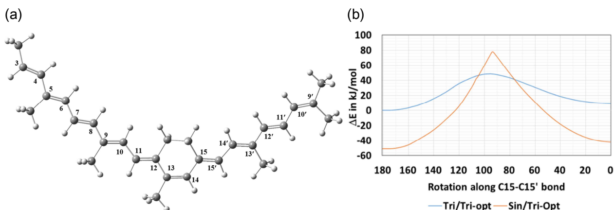
Figure 11. (a) Optimized structure of the locked-13,14- cis -SPO. (b) Singlet-triplet crossing of the locked-13,14- cis -SPO. Tri/Tri-Opt and Sin/Tri-Opt respectively represent the triplet and singlet energies obtained at optimized structures for the triplet state.
