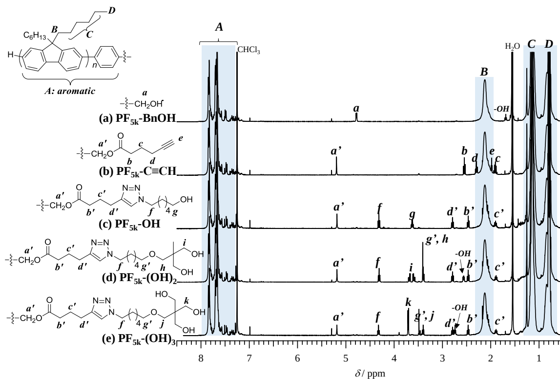
Figure 1. ^1\text{H} NMR spectra of (a) \text{PF}_{5k}\text{-BnOH} ( M_{n,\text{NMR}} = 4800 \text{ g mol}^{-1} , \bar{D} = 1.34 ), (b) \text{PF}_{5k}\text{-C}\equiv\text{CH} ( M_{n,\text{NMR}} = 4900 \text{ g mol}^{-1} , \bar{D} = 1.31 ), (c) \text{PF}_{5k}\text{-OH} ( M_{n,\text{NMR}} = 5000 \text{ g mol}^{-1} , \bar{D} = 1.29 ), (d) \text{PF}_{5k}\text{-(OH)}_2 ( M_{n,\text{NMR}} = 5500 \text{ g mol}^{-1} , \bar{D} = 1.22 ), and (e) \text{PF}_{5k}\text{-(OH)}_3 ( M_{n,\text{NMR}} = 5500 \text{ g mol}^{-1} , \bar{D} = 1.21 ) in \text{CDCl}_3 (400 MHz).
