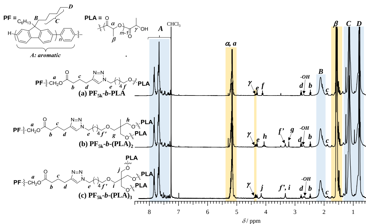
Figure 4. ^1\text{H} NMR spectra of (a) \text{PF}_{5k}\text{-}b\text{-PLA} ( M_{n,\text{NMR}} = 9400 \text{ g mol}^{-1} ; M_{n,\text{SEC}} = 12000 \text{ g mol}^{-1} ; \bar{D} = 1.15 ), (b) \text{PF}_{5k}\text{-}b\text{-(PLA)}_2 ( M_{n,\text{NMR}} = 9800 \text{ g mol}^{-1} ; M_{n,\text{SEC}} = 12200 \text{ g mol}^{-1} ; \bar{D} = 1.17 ), and (c) \text{PF}_{5k}\text{-}b\text{-(PLA)}_3 ( M_{n,\text{NMR}} = 10500 \text{ g mol}^{-1} ; M_{n,\text{SEC}} = 14000 \text{ g mol}^{-1} ; \bar{D} = 1.19 ) in \text{CDCl}_3 (400 MHz).
