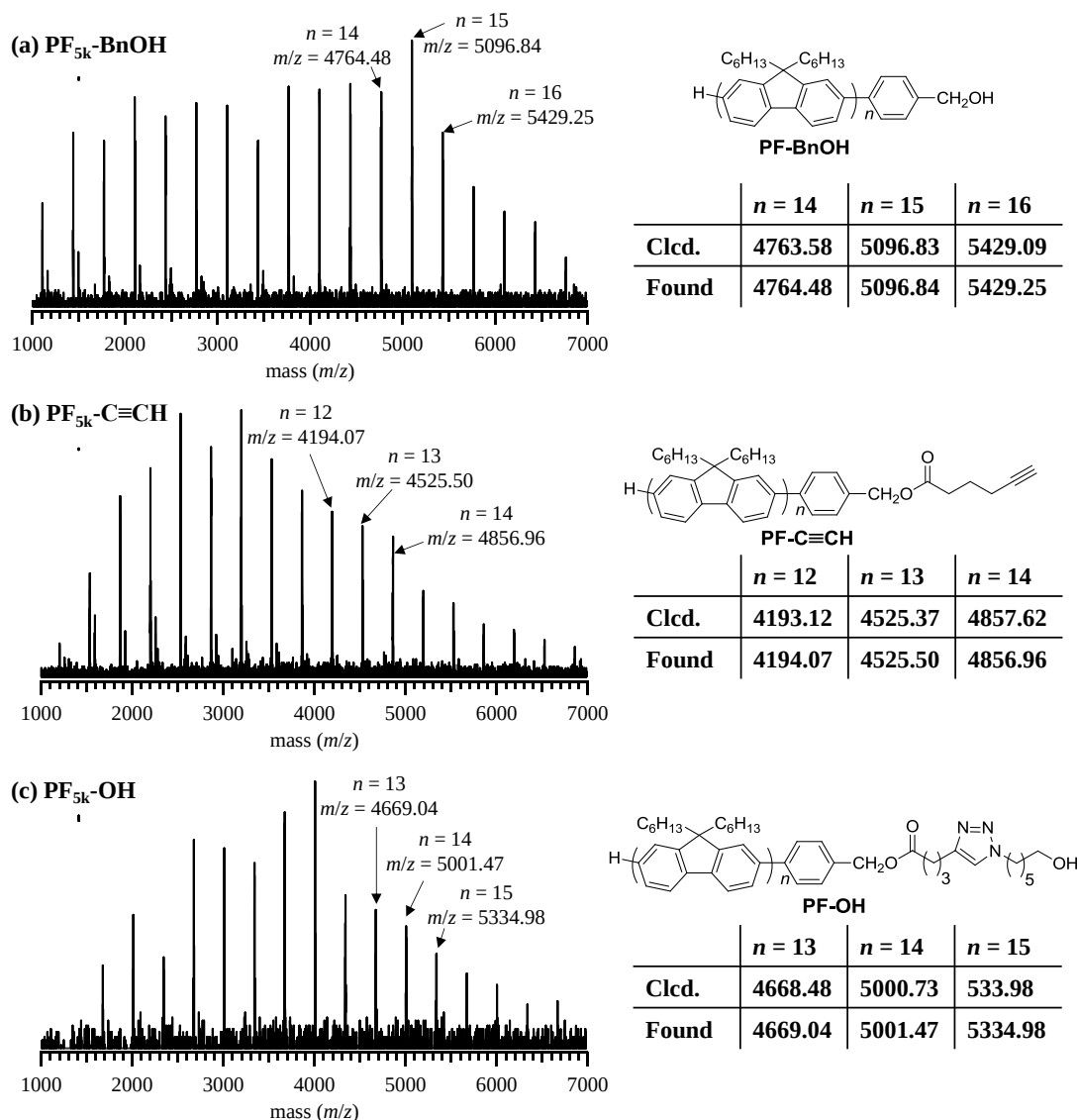
Figure 2. MALDI-TOF MS spectral analysis of (a) PF 5k -BnOH ( M_{n,NMR} = 4800 \text{ g mol}^{-1} , \bar{D} = 1.34 ), (b) PF 5k -C≡CH ( M_{n,NMR} = 4900 \text{ g mol}^{-1} , \bar{D} = 1.31 ), and (c) PF 5k -OH ( M_{n,NMR} = 5000 \text{ g mol}^{-1} , \bar{D} = 1.29 ).
