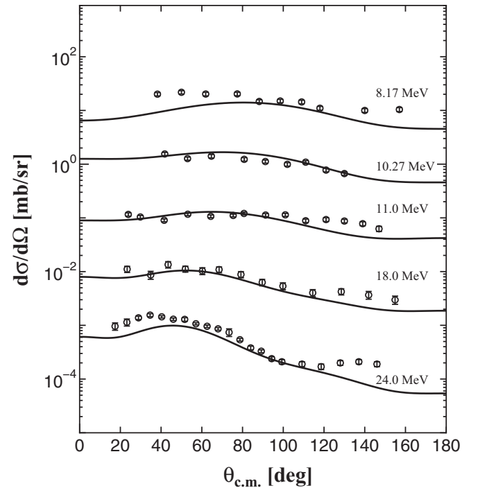
FIG. 11. Angular distributions of the n + {}^7\text{Li} inelastic scattering for the excited 7/2^- state at the excitation energy of 4.65 MeV of {}^7\text{Li} . The solid lines and open circles correspond to the calculated results and experimental data [15,23,27,28], respectively. The data are subsequently shifted downward by a factor of 10^{-1} – 10^{-4} from 10.27 to 24.0 MeV.
