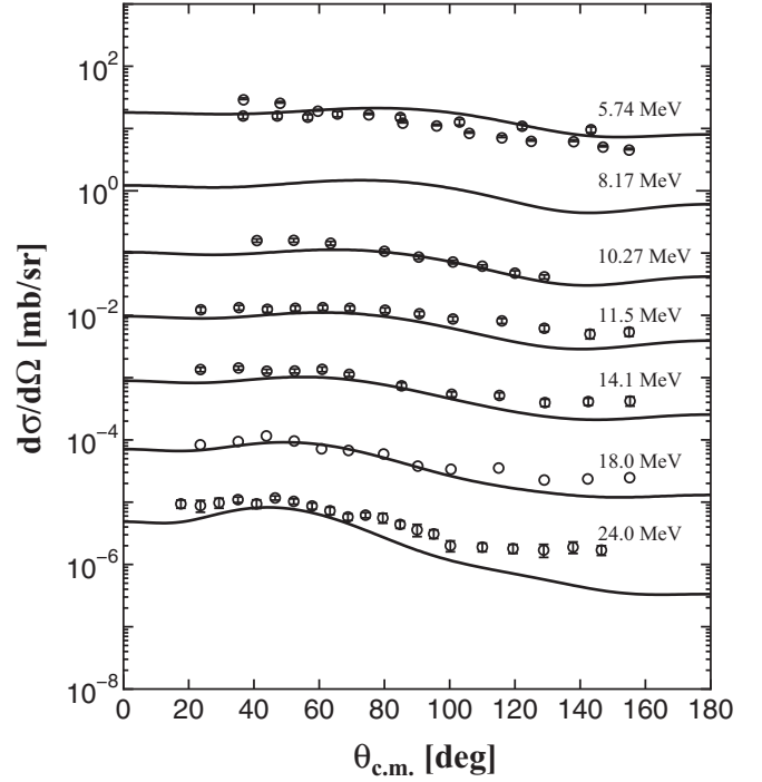
FIG. 6. Angular distributions of the n + {}^6\text{Li} inelastic scattering for the excited 3^+ state at the excitation energy of 2.18 MeV of {}^6\text{Li} . The solid lines and open circles correspond to the calculated results and experimental data [15,23,25,27–29], respectively. The data are subsequently shifted downward by a factor of 10^{-1} – 10^{-6} from 8.17 to 24.0 MeV.
