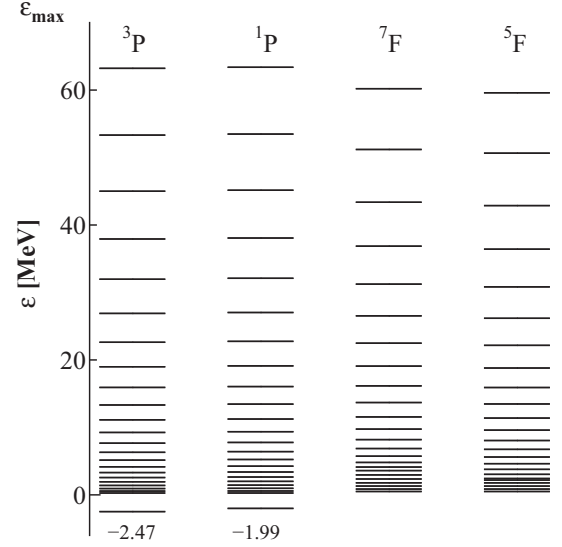
FIG. 2. The discretized eigenstates of {}^7\text{Li} . Each panel indicated as {}^3P , {}^1P , {}^7F , and {}^5F , from left to right sides.
