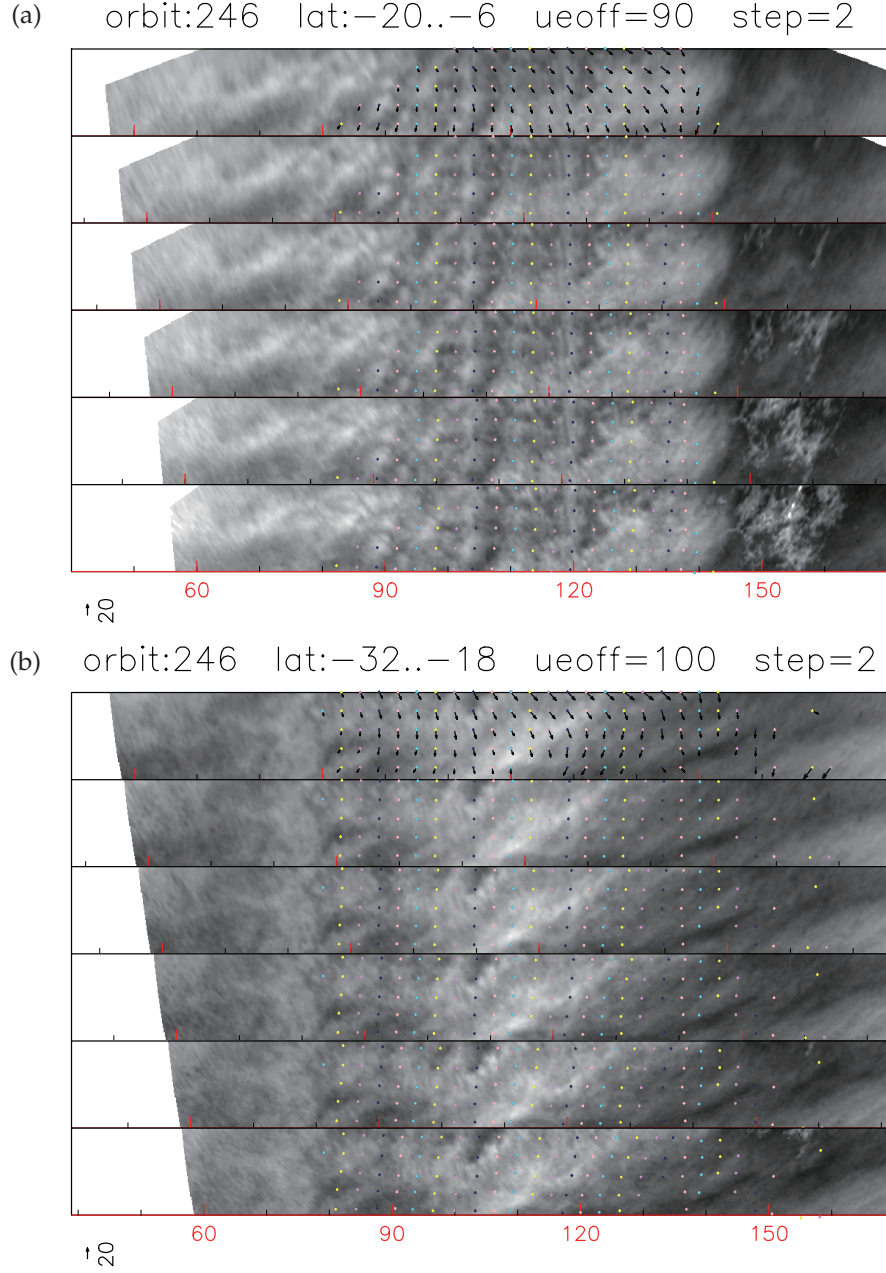
Figure 4.7: CMVs that satisfy \varepsilon < 10 \text{ m s}^{-1} and \chi < 10 \text{ m s}^{-1} (arrows), trajectories corresponding to the CMVs (colored dots), and the preprocessed brightness F (shading) for the orbit 246. The latitudinal ranges covered are (a) 20^\circ\text{S} – 6^\circ\text{S} and (b) 32^\circ\text{S} – 18^\circ\text{S} . Zonal winds corresponding to the solid body rotations that have zonal velocities (a) -90 \text{ m s}^{-1} and (b) -100 \text{ m s}^{-1} at the equator are subtracted from the CMV arrows (unlike in Fig. 3.9 where a uniform zonal wind is subtracted). To show their scales, an arrow whose length corresponds to 20 \text{ m s}^{-1} is shown near the lower-left corner of each panel. The brightness is shown for every 40 min (thus shown are six of the eleven images used to derive the CMVs). To ease visual tracking, images are shifted longitudinally with time (see the red tick marks), which corresponds to the longitudinal shift by the solid body rotations subtracted from CMV arrows. The dots are advected by CMVs constantly with time. Caution: there are small-scale features associated with instrumental error in (a) around the longitude 150^\circ at later times; they do not move in the original images.
