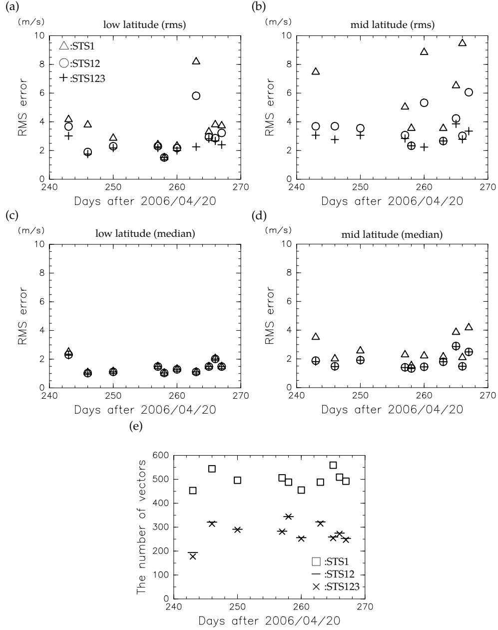
Figure 4.9: The rms (a, b) and median (c, d) of \chi , and the number of vectors (e) obtained from the ten orbit from 243 to 267 by using the STS1, STS12, and STS123 estimations. (a, c) Averaged over 30°S–10°N; (b, d) averaged over 45°S–30°S.
