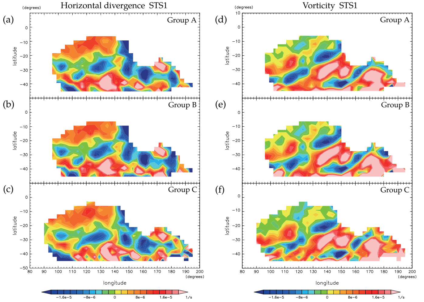
Figure 4.6: As in Fig. 4.5a–c but for horizontal divergence (a–c) and vorticity (d–f) obtained from CMVs screened by the screening 1.
