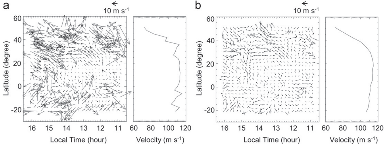
Figure 1.4: (a) Horizontal wind vector field obtained from the maxima of the cross-correlation surface, and the corresponding zonal mean zonal winds. (b) Horizontal wind vector field obtained after selecting a 2nd, 3rd ... peak, having taken into account consistency with the surrounding wind vectors ( Kouyama et al., 2012 ).
