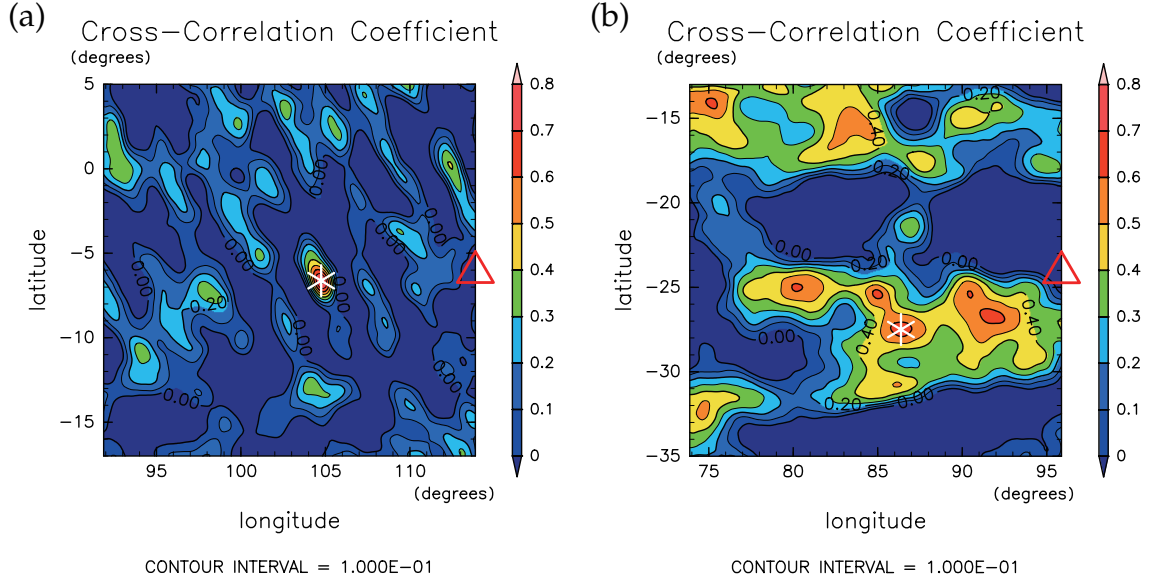
Figure 3.3: The cross-correlation coefficients calculated from two images separated by 200 min in the orbit 246. (a) A typical example where the cross-correlation has a distinguished maximum (denoted by the * mark). The center of the template is at 114°E, 6°S (denoted by the Δ mark). The abscissa and the ordinate shows the longitude and latitude, respectively, of the center of the target regions. (b) As in (a) but for a typical example where the cross-correlation has multiple peaks that are comparable. The center of the template is at 96°E, 24°S. The cross-correlation is maximized when the center of the target is at the location designated by the * mark.
