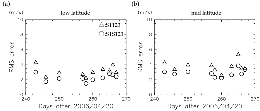
Figure 4.10: The rms of \chi obtained from the ST123 (triangles) and STS123 (circles) results averaged over (a) 30°S–10°N and (b) 45°S–30°S.
