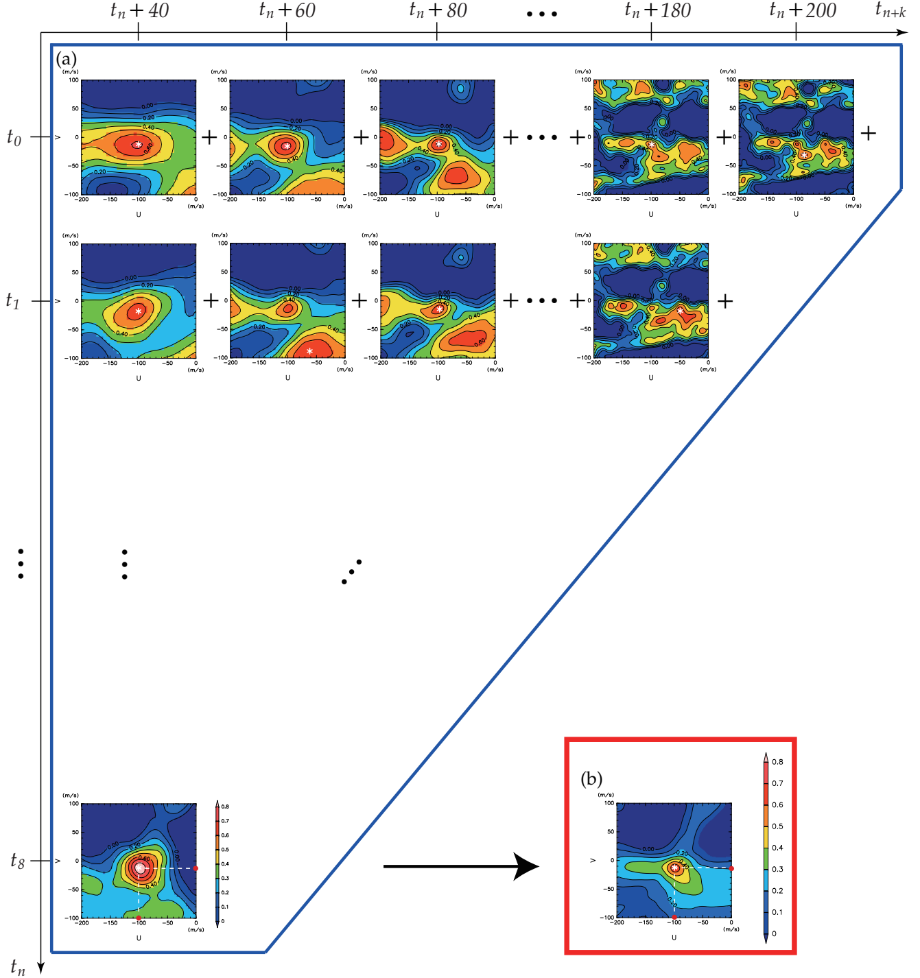
Figure 3.6: (a) Cross-correlation surfaces r_p(\lambda_a, \phi_b, u_{l,b}, v_m) for individual image pairs, and (b) superposed cross-correlation r(\lambda_a, \phi_b, u_{l,b}, v_m) defined by Eq. (3.15). Shown are the results for the orbit 246 and (\lambda_a, \phi_b) = (96^\circ\text{E}, 24^\circ\text{S}) . In (a), the surfaces are aligned with respect to t_n (ordinate) and the time interval t_{n+k} - t_n (abscissa). The * mark designates the maximum. Here, v_{\min} and v_{\max} are set to -100 and 100 \text{ m s}^{-1} , respectively, unlike the actual values ( -70 and 70 \text{ m s}^{-1} ) used to estimate CMVs in this study.
