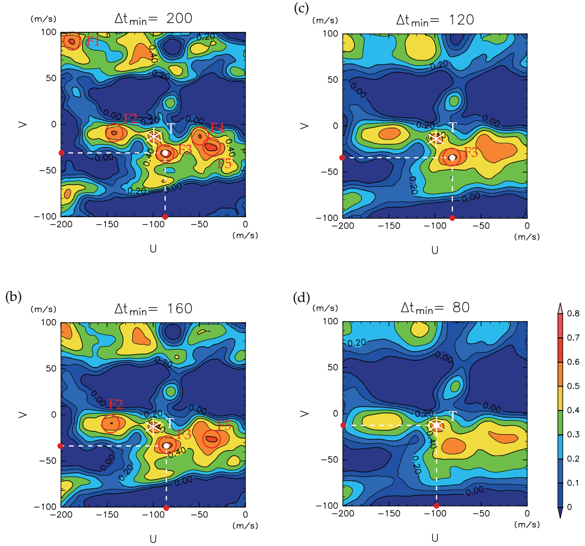
Figure 3.7: Superposed cross-correlation surfaces for various values of \Delta t_{\min} for the same case as in Fig. 3.6: (a) 200 min, (b) 160 min, (c) 120 min, and (d) 80 min. The peak corresponding to the true velocity, which is evident in Fig. 3.6b, is designated by the * mark and named "T", while the false peaks are named F1, F2, \dots . The maximum correlation is denoted by the \bullet mark. Here, v_{\min} and v_{\max} are set to -100 and 100 \text{ m s}^{-1} , respectively, unlike the actual values ( -70 and 70 \text{ m s}^{-1} ) used to estimate CMVs in this study.
