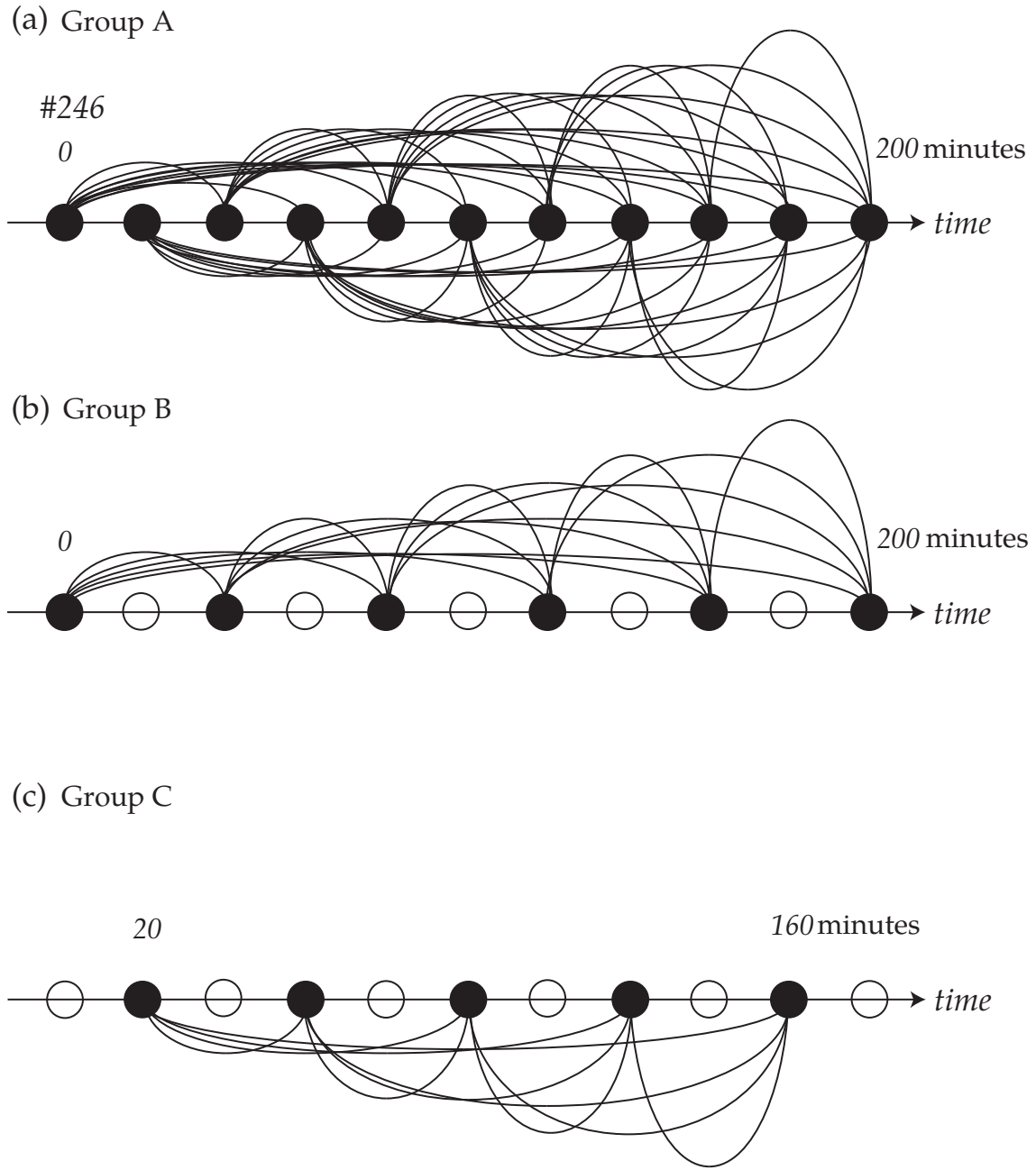
Figure 4.4: Illustration of the observation times (circles) and the pairs to compute cross-correlation (curves) for the group (a) A, (b) B, and (c) C. The number of times, 11, is based on the orbit 246, in which observation is made every 20 min.
