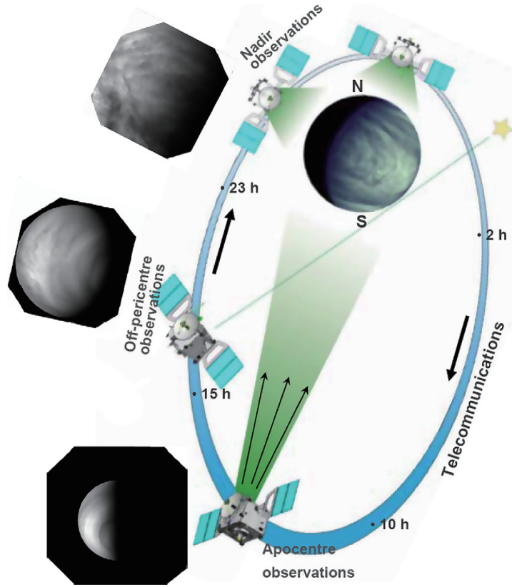
Figure 2.1: Overview of the VEX the orbit and telecommunications ( Titov et al., 2012 ).
