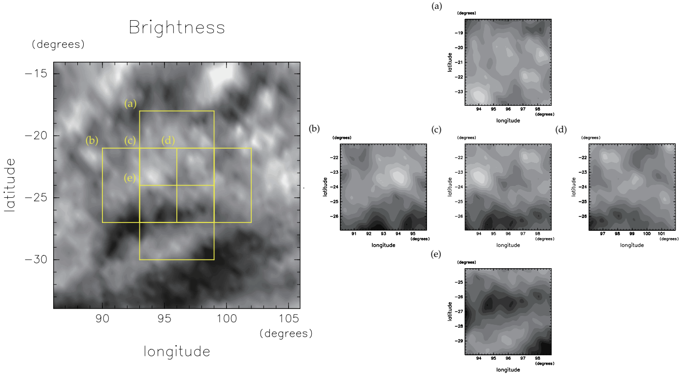
Figure 3.8: Left: configuration of the templates used for the STS estimation using spatial moving average (boxes a–e) overlaid on a preprocessed brightness F . Right: the distribution of F in the five template regions. The cloud tracking velocity is defined at the center of the box c.
