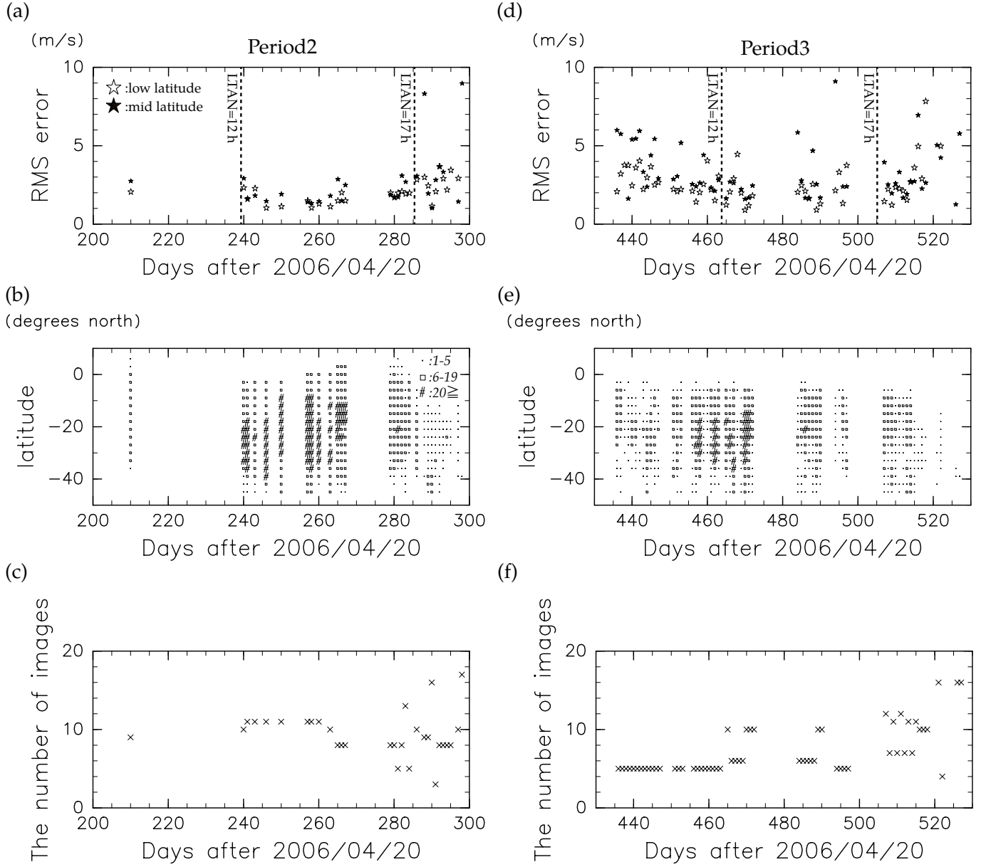
Figure 4.12: (a) The median of \chi (from the STS123 results) averaged over 30^{\circ}\text{S} – 10^{\circ}\text{N} (outlined \star marks) and 45^{\circ} – 30^{\circ}\text{S} (filled \star marks), (b) the number of CMVs for each latitude (dots for 1–5, squares for 6–19, and sharps if greater or equal to 20), and (c) the number of images used, for the period 2. (d)–(f) as in (a)–(c) but for the period 3. Dotted (dashed) lines in (a) and (d) show when LTAN is 12 (17) h.
