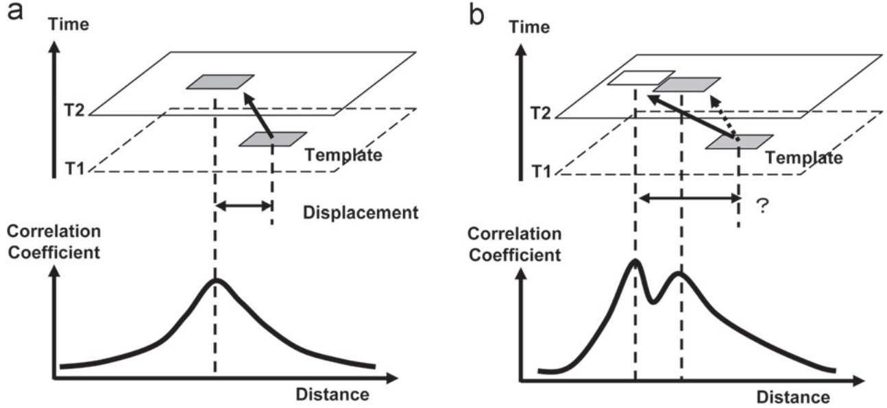
Figure 1.3: (a) Case with a single peak in the cross section of the spatial correlation surface: there is a one-to-one correspondence between the sub-image patterns at times T1 and at T2. (b) Case with multiple peaks in the cross section of the spatial correlation surface: the sub-image patterns at times T1 and T2 do not have a one-to-one correspondence ( Kouyama et al. , 2012).
