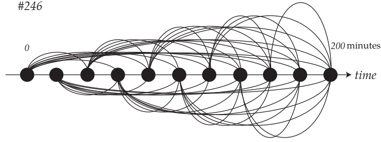
Figure 3.4: Example of the combinations of observation times to compute. Black circles show the observation times, which are at every 20 min in the orbit 246. The arcs show the combinations: on their left (earlier) ends are the times to set templates, and on their right (later) ends are the times to set targets.
