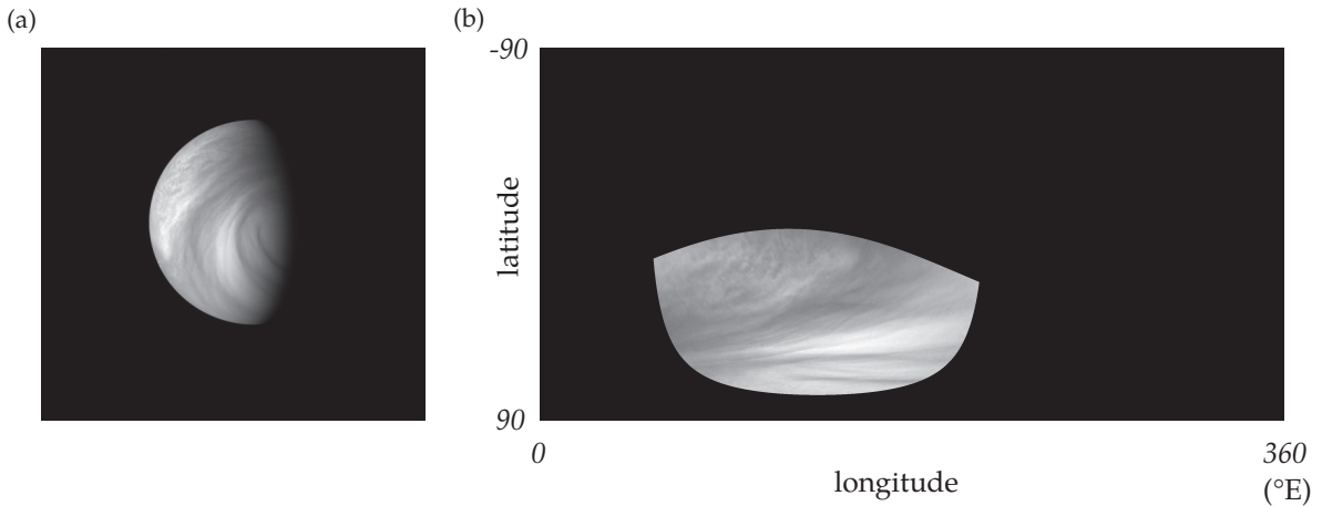
Figure 3.1: Example of the UV brightness data. (a) Original version 2.0 data at 01:00:31 UTC, 23 Dec, 2006 from the orbit 246. (b) As in (a) but for the preprocessed brightness F .
