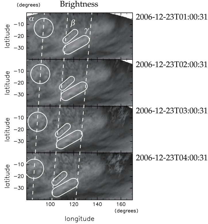
Figure 3.2: The preprocessed brightness F from the orbit 246, starting at 01:00 (as in Fig. 3.1) with one hour time interval. Dashed lines and solid enclosures highlights features that can be readily tracked by visual inspection.
