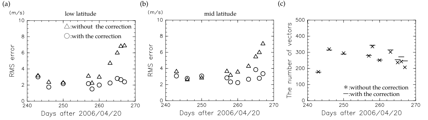
Figure 4.11: The rms (a–b) of \chi and the number of vectors (c) obtained from the STS123 estimation with (“o” or “—”) and without (“ \Delta ” or “*”) the optical and pointing-angle corrections. Averaged over (a) 30°S–10°N, (b) 45°S–30°S.
