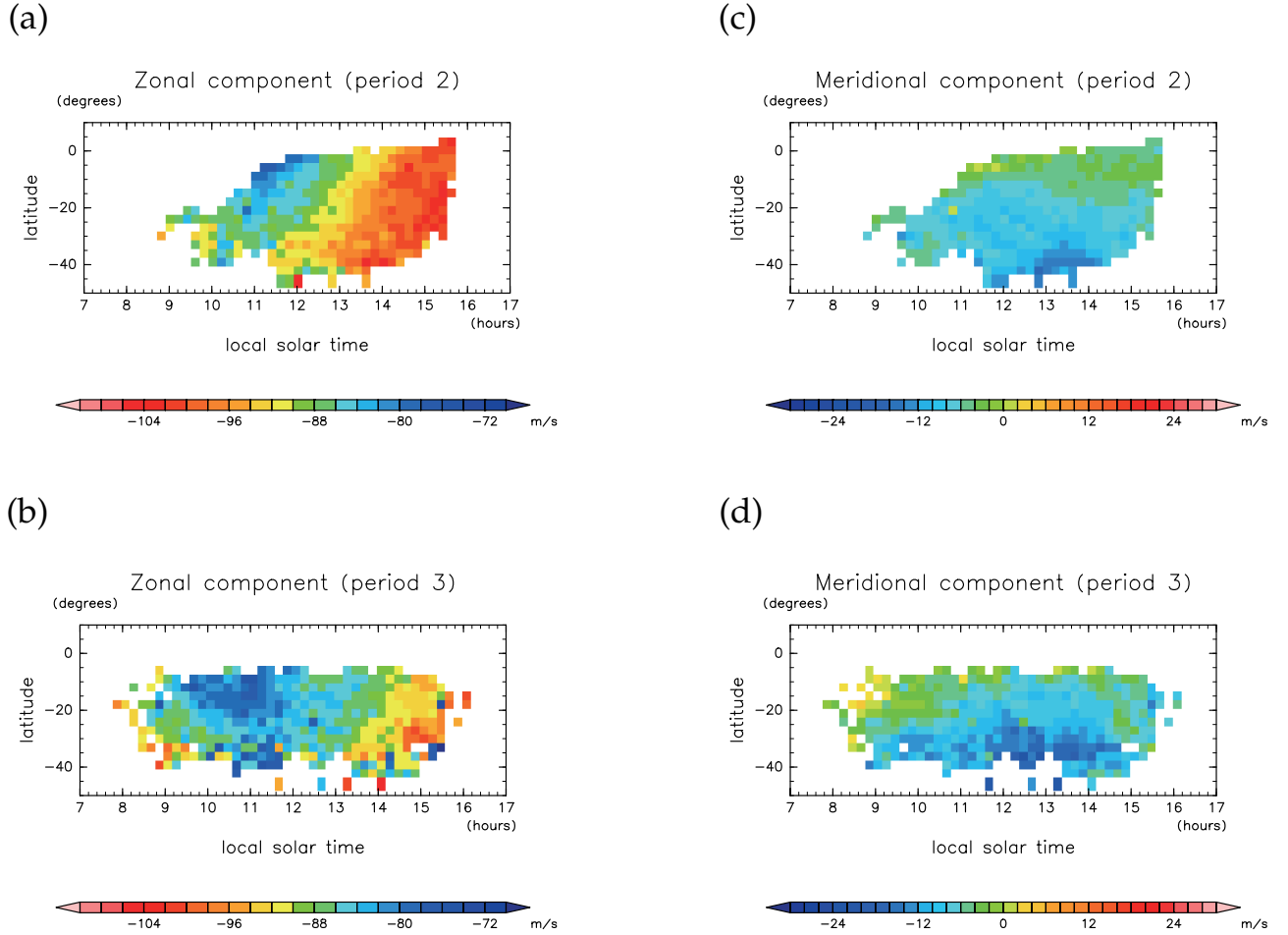
Figure 5.4: Tidal component obtained for the periods 2 (a, c) and 3 (b, d). (a, b) Zonal wind; (c,d) meridional wind. The results are shown where the number of CMVs is greater than or equal to 4.
