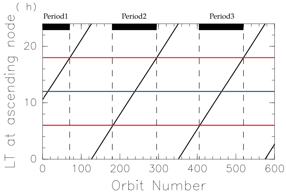
Figure 2.2: The LTAN of the VEX up to the orbit 600 (11, Dec, 2007). The red lines show 6 am and 18 pm, blue line shows the noon.
