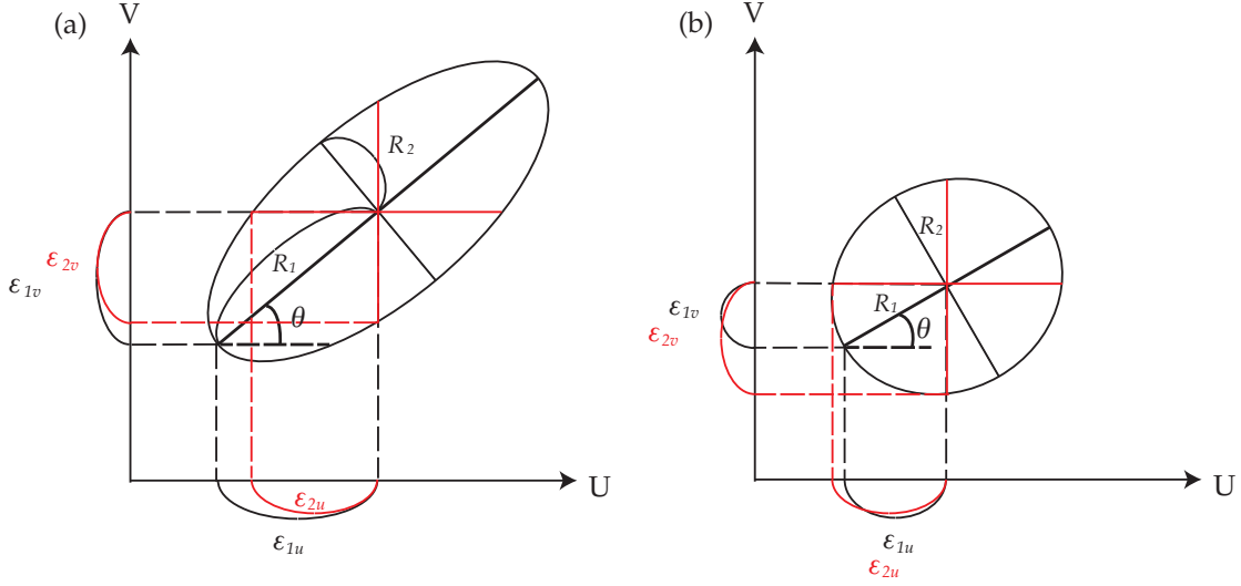
Figure 4.3: Schematic illustration of the precision estimations 1 and 2. (a) When the correlation surface above r = r_{lb} is elongated. (b) When it is relatively isotropic.
