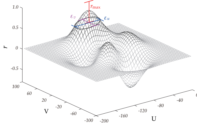
Figure 4.1: Schematic illustration of the CMV precision based on the lower confidence bound of the maximum cross-correlation coefficient r_{\max} . The curved surface represents the cross-correlation surface as a function of velocity. The oval is the cross section between the surface and the r = r_{\text{lb}} plane.
