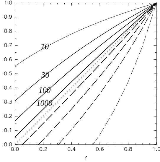
Figure 4.2: The 90% upper (solid lines) and lower (dashed lines) confidence bounds of cross-correlation coefficient r for some effective degrees of freedom (10, 30, 100, and 1000 as indicated in the figure). The dotted line is the diagonal line to indicate r itself.
