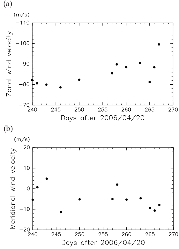
Figure 5.3: Mean (a) zonal and (b) meridional winds for the twelve orbits in the period 2 obtained by averaging CMVs between 20°S and the equator. The abscissa is the orbit numbers, which are the days after April 20, 2006.
