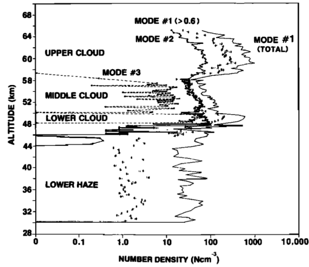
Figure 1.1: Vertical profile of density number for cloud droplets ( Knollenberg and Hunten, 1980 ).
