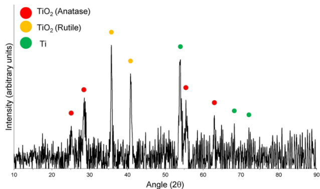
Figure 6(c) XRD spectrum of \text{TiO}_2 nanoballs.
