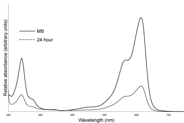
Figure 7(c) Photoabsorbance results for MB decomposition in presence of \text{TiO}_2 nanoballs
