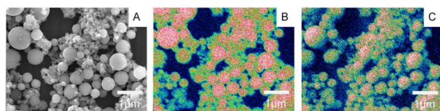
Figure 5(c) SEM-EDS map of TiO 2 nanoballs showing (A) greyscale, (B) Ti K, (C) O K.
