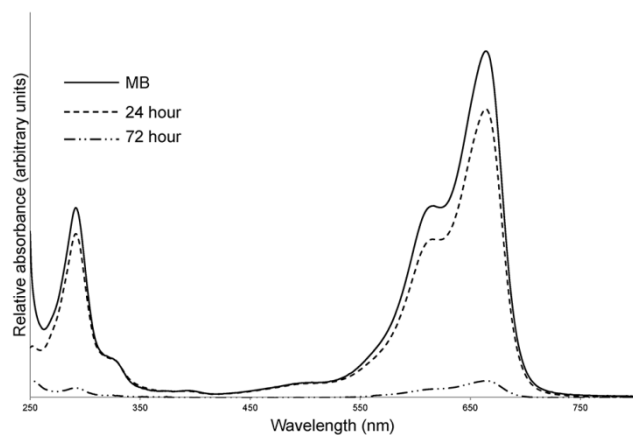
Figure 7(a) Photoabsorbance results for MB decomposition in presence of SUS nanoballs.
