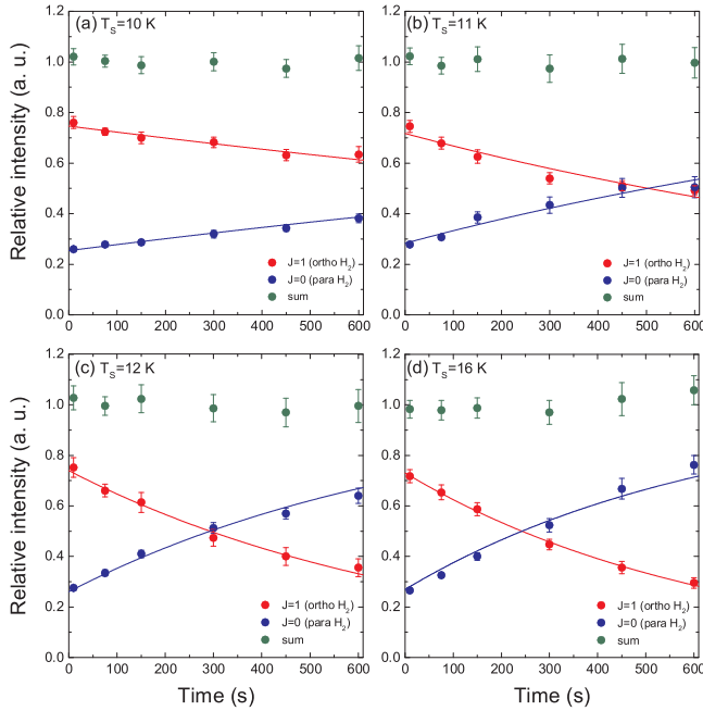
FIG. 2. The time evolution of the photodesorbed \text{H}_2 intensities for J = 0 (blue), 1 (red), and their sum (green). Intensities were derived from the integrated photodesorbed \text{H}_2 signals. The surface-temperature dependence of \text{H}_2 is shown for (a) 10, (b) 11, (c) 12, and (d) 16 K. The origin of the x axis corresponds to the opening of the pulsed valve of the molecular beam source. The error bars represent the confidence reliabilities for 6 to 9 measurements. Solid lines are results of single-exponential fittings.
