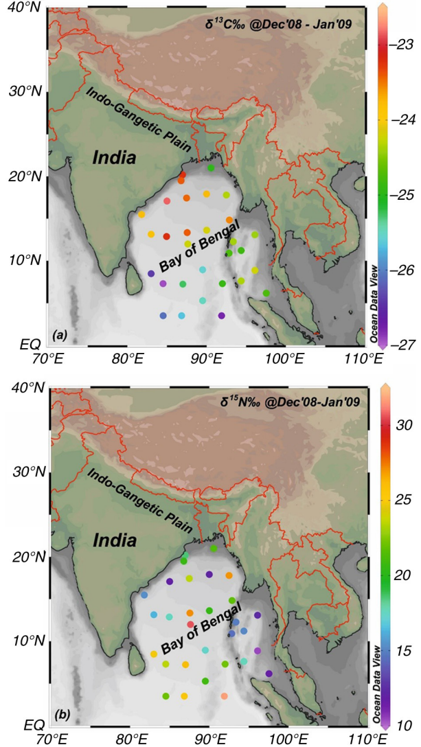
Fig. 3. Spatial distributions of (a) stable carbon ( \delta^{13}\text{C}_{\text{TC}} ) and (b) nitrogen ( \delta^{15}\text{N}_{\text{TN}} ) isotopic composition of fine mode ( \text{PM}_{2.5} ) aerosols collected from the marine atmospheric boundary layer of the Bay of Bengal during a winter cruise (27 December 2008 to 28 January 2009).
