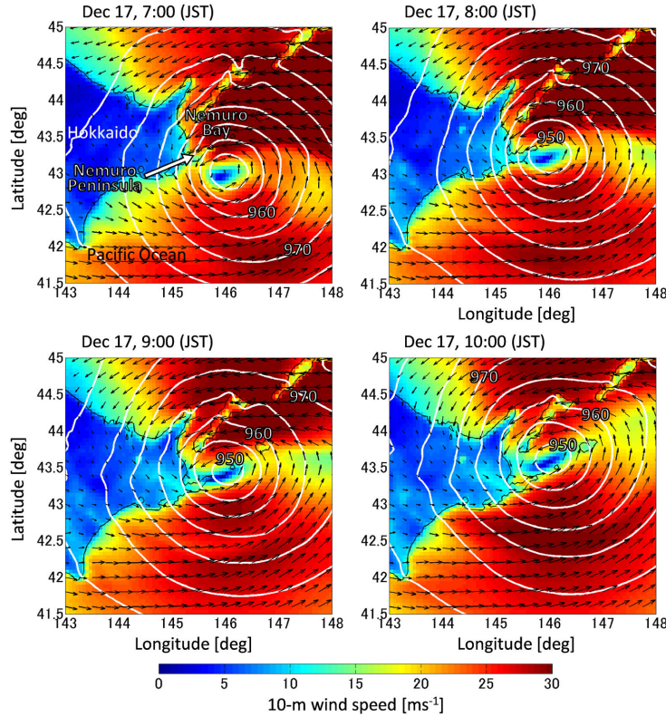
Fig. 6. Distribution of the air pressure and wind velocity obtained in the present meteorological simulation. Color and arrows indicate wind speed at 10 m above the surface, isobars represent the pressure at sea level.
