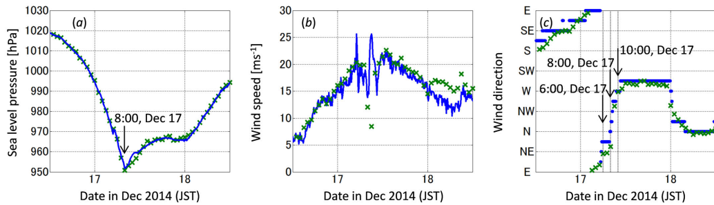
Fig. 5. Comparison between the forecast results by JMA-MSM (green) and observed data by AMeDAS (blue) for the (a) sea level pressure, (b) wind speed and (c) wind direction at the Nemuro AMeDAS station.
