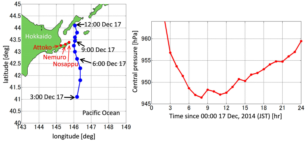
Fig. 4. The computed trajectory (left) and central pressure (right) of the extratropical cyclone, provided by JMA. The locations of the AMeDAS stations in the Nemuro Peninsula are indicated.
