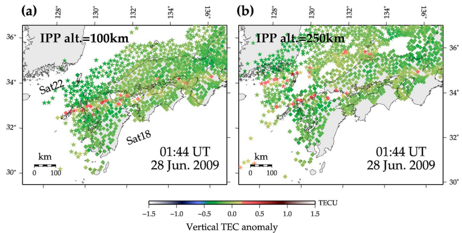
Figure 2. Altitude constraint by vertical TEC anomaly maps derived from two different satellites. Sub-ionospheric points (SIPs) of Satellite 18 and Satellite 22 are represented by diamonds and stars, respectively. SIPs are projected by assuming the IPP altitude at (a) 100 km ( E region height) and (b) 250 km ( F region height). Looking at the ENE-WSW frontal structure, two images coincide in Figure 2a, while gaps emerge in Figure 2b. This ensures that the frontal structure exists at the altitude of E region of the ionosphere.
