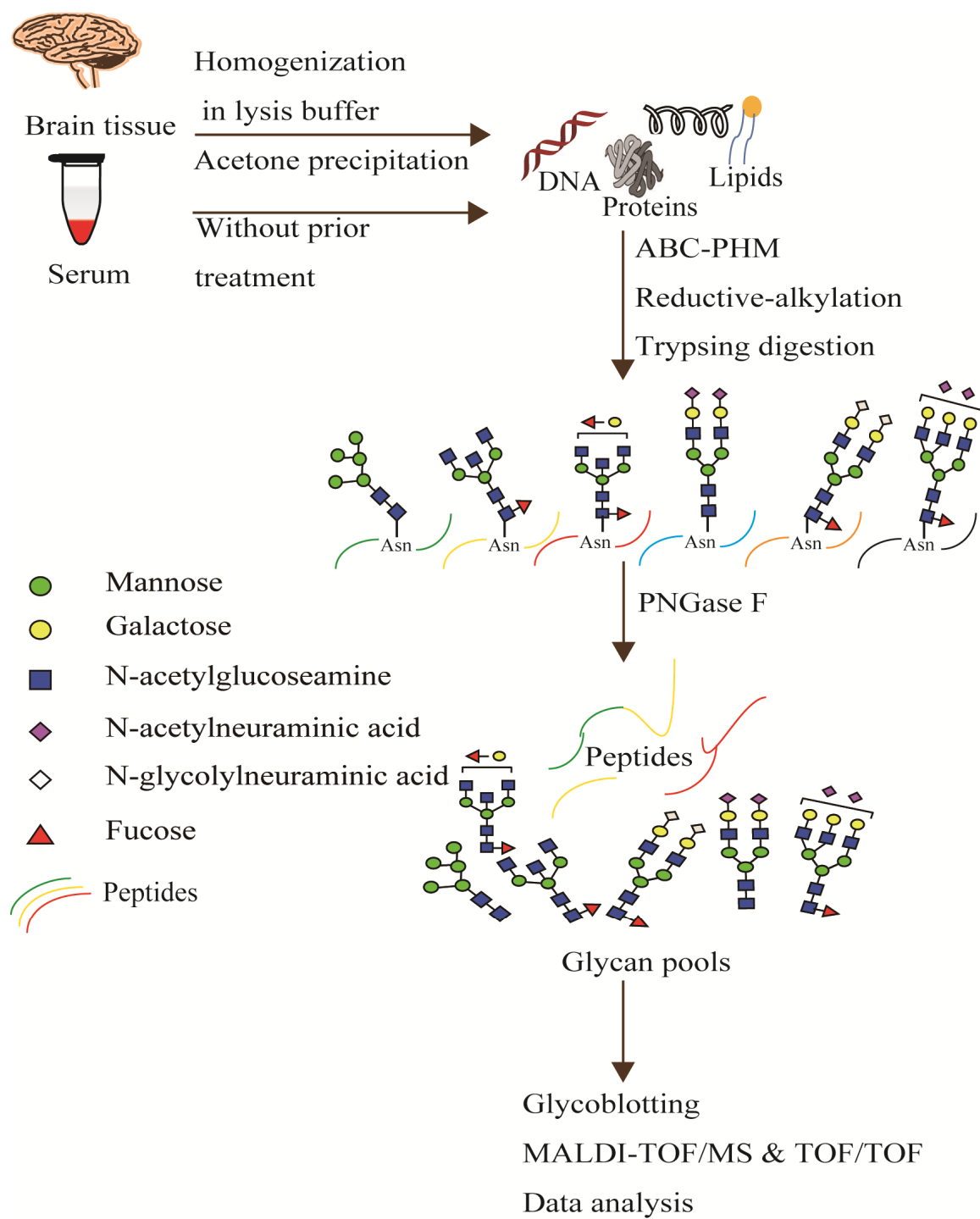
Figure 2.2. Schematic representation of N -glycomics.
