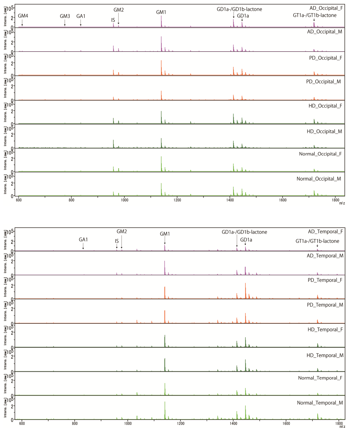
Figure 4. 5. Representative MALDI-TOF MS spectra of human brain tissue GSL-omics.
