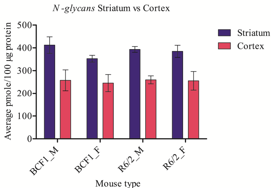
Figure 2.14. Comparison of N -glycans in striatum and cortex (R6/2, HD transgenic mice; BCF1, wild type mice; M, male; and F, female).
