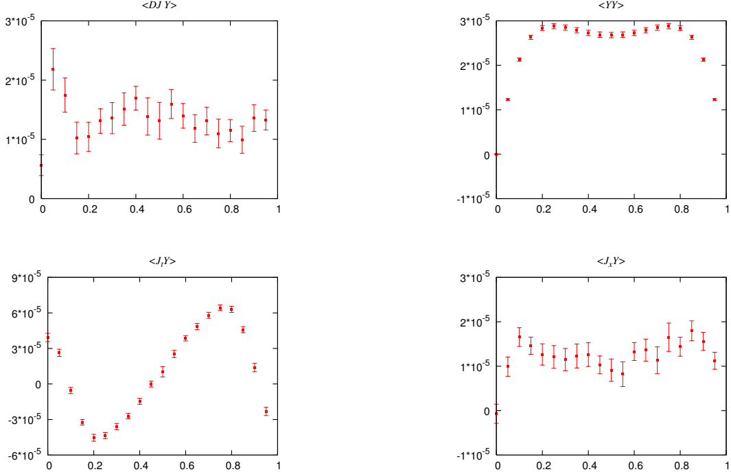
Figure 13: Correlation functions used in our study of the SWTI. The corresponding parameters are N_t = 20 , m^2/\lambda = 0.5 . All the correlators are presented as a function of t/N_t at fixed x = N_x/2 for \alpha = \beta = 1 . The other correlators for \alpha = \beta = 2, \dots, 16 behave in the same way.
