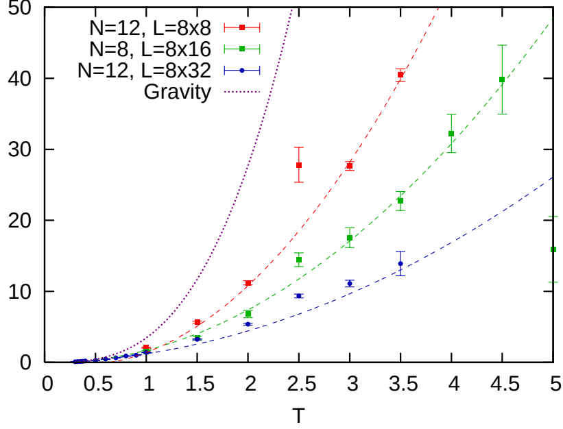
Figure 19: Normalized "energy" (E - PL)/(N^2 L) . The line named gravity indicate the expected curve obtained from black p-brane model. The data named Ib correspond to N = 8 , N_t = 8 , N_x = 16 , Ila correspond to N = 12 , N_t = 8 , N_x = 8 and Iic N = 12 , N_t = 8 , N_x = 32 .
