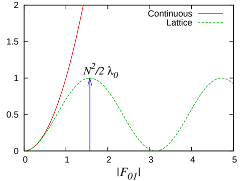
Figure 4: Action of the gauge field as a function of the magnitude of the gauge field ( |F_{01}| = \sqrt{1/N \text{tr} F_{01}^2} ). The lattice action is consistent with the continuous one when the fields are small, but shows other minima. A "potential" wall with a height of N^2/2\lambda_0 suppress the transition between the minima.
