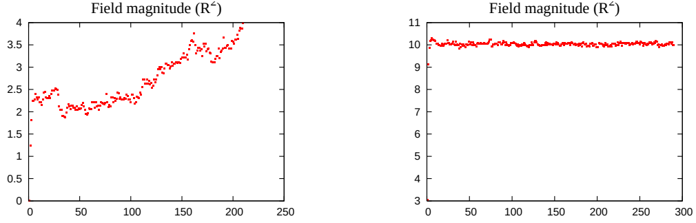
Figure 5: Size of the scalar fields R^2 = \text{tr}(X_i^2) as a function of the trajectory. The gauge group is N = 12 in both case. On the left, we have a smaller lattice N_t = 8 , N_x = 8 at T = 0.8 . On the right, the parameters are N_t = 8 , N_x = 16 at T = 0.3 . The simulation on the left have a flat direction problem.
