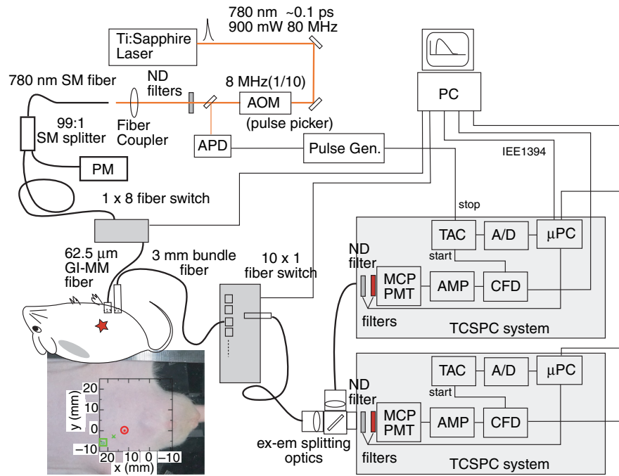
Fig. 2 Experimental setup for in vivo measurements. The inset picture shows the approximated positions of the injection (red circle) and detection (green box) points and the scales on the abdominal region. The output at 780 nm from a mode-locked Ti:Sapphire laser was used as an excitation source for ICG and the fluorescence and excitation light were detected by a bundled fiber. The TPSFs were obtained by TCSPC systems. A similar system was used in the phantom measurements.
