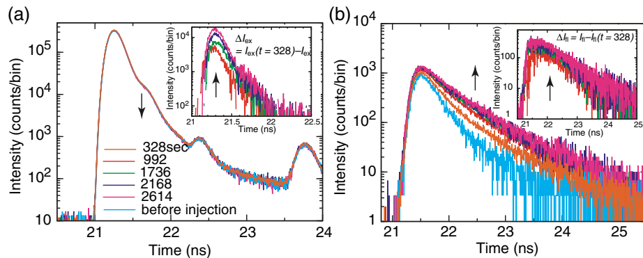
Fig. 5 (a) Excitation and (b) fluorescence TPSFs and the TPSF changes from the reference profile (inset) with time after the ICG injection. The same colors indicate TPSFs or change of TPSF at the same time point in (a) and (b). The arrows in the figures indicate the time flow. The excitation and fluorescence TPSFs are decreasing and increasing with the time, respectively.
