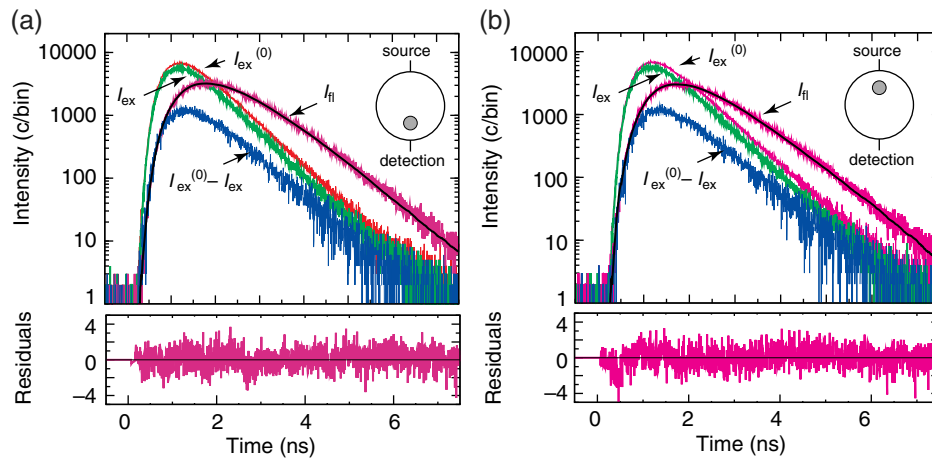
Fig. 3 TPSFs with 3-cm cylinder phantom measurements. The source-detection plane was the middle of cylinder. The geometry of the source-detection fibers are illustrated in the insets. The target with 6 mm in diameter was highlighted. Each TPSF is indicated by the arrows. I_{ex}^{(0)} and I_{ex} are the excitation TPSF without and with the target, respectively, and I_{fl} is the fluorescence TPSF. The solid black lines superimposed on I_{fl} show the best fits to the fluorescence TPSF using the difference of excitation TPSFs. The bottom figures show the residuals of the best fits.
