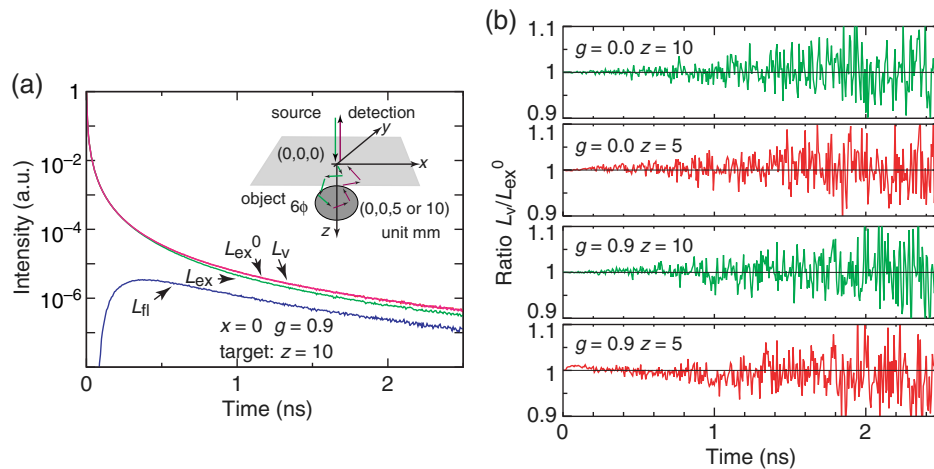
Fig. 1 (a) TPSFs of excitation light with and without the fluorescence target L_{ex} and L_{ex}^0 , fluorescence L_{fl} , and calculated by the Monte Carlo simulation and the sum TPSF of fluorescence and excitation with the target L_v . (b) The difference, calculated by the ratio of L_{ex}^0 and L_v . The geometry of the simulation is illustrated in the inset. The sphere fluorescence target with 6 mm diameter was set at the origin with different depths 5 and 10 mm. The source and detector were placed at the origin.
