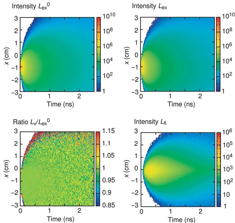
Fig. 7 Pseudocolor images of the excitation TPSF with and without the target, L_{\text{ex}} and L_{\text{ex}}^0 , the fluorescence L_f and the ratio of L_v = L_{\text{ex}} + L_f to L_{\text{ex}}^0 , which were calculated by the MC simulation. The simulation parameters were the same as the previous simulation except the photon injection point at (-1 \text{ cm}, 0 \text{ cm}, 0 \text{ cm}) .
