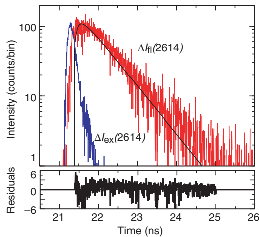
Fig. 6 A single-exponential fitting to the differential TPSF profiles of fluorescence at 2614 s. The fluorescence and excitation profiles are shown by red and blue lines, respectively. The fitting curve is shown by black line. The bottom figure shows the residuals of the fitting. The intensity scale was calibrated to that of the TPSF profile at 2614 s.
