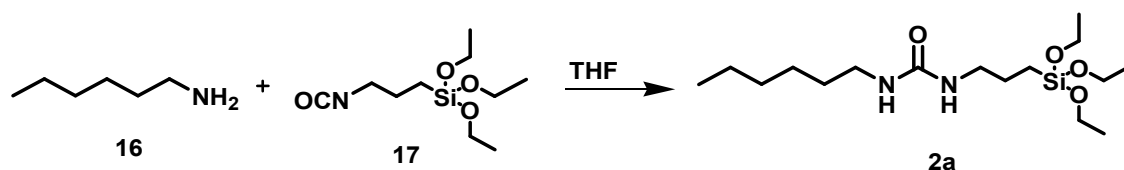
Scheme 3 Synthetic scheme of compound 2a.
