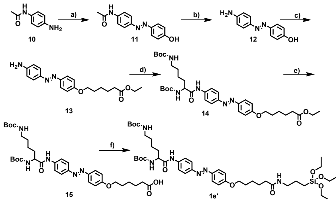
Scheme 2 a) HCl, H 2 O, NaNO 2 , NaOH, PhOH, 0–2 °C. b) 10% NaOH, Reflux 2h. c) Br-(CH 2 ) 5 -COOEt, K 2 CO 3 , (CH 3 ) 2 CO, 50–60 °C. d) Boc-Lys-(Boc)-OH, DCHA, DCC, HOBt, DMF. e) Dioxane, 1M aq. KOH. f) OCN-(CH 2 ) 3 -Si-(OEt) 3 , THF.
