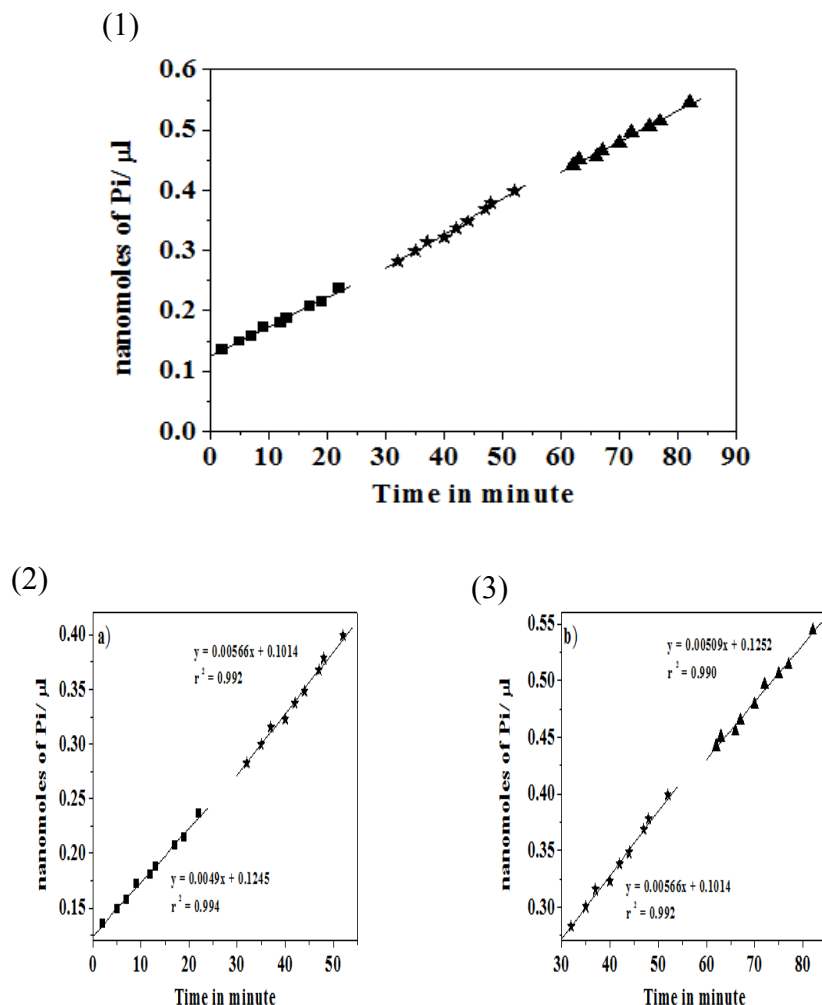
Fig. 5 Time dependent inorganic phosphate releases from hydrolysis of ATP by kinesin at different environments of azobenzene functionalized surface of 1a before irradiation [(1) squares], after 366 nm irradiation [(1) stars] and after visible light irradiation [(1) triangles]. Enlarged figure of phosphate release before and after 366 nm irradiation (2) and after 366 nm and >500 nm irradiation (3).
