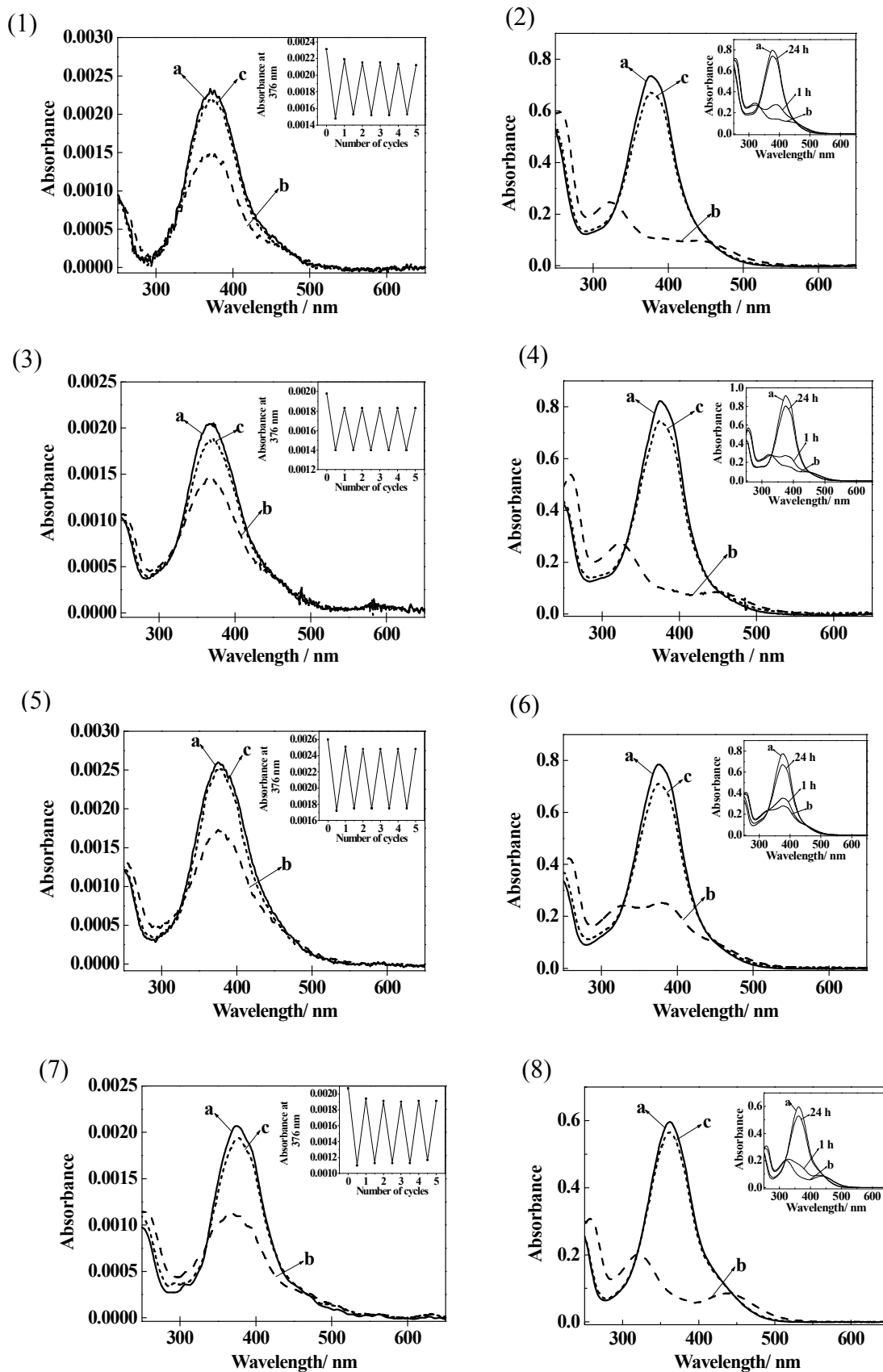
Fig. 1 Absorption spectral changes of 10% of 1b-e and 90% of 2a or 2b in quartz surface after deprotection of tert -Boc group [left (1), (3), (5), (7)] and that of 1b'-d' in acetonitrile and 1e' in DCM before deprotection of tert -Boc group [right (2), (4), (6), (8)]. (a) Before irradiation. (b) photostationary state
