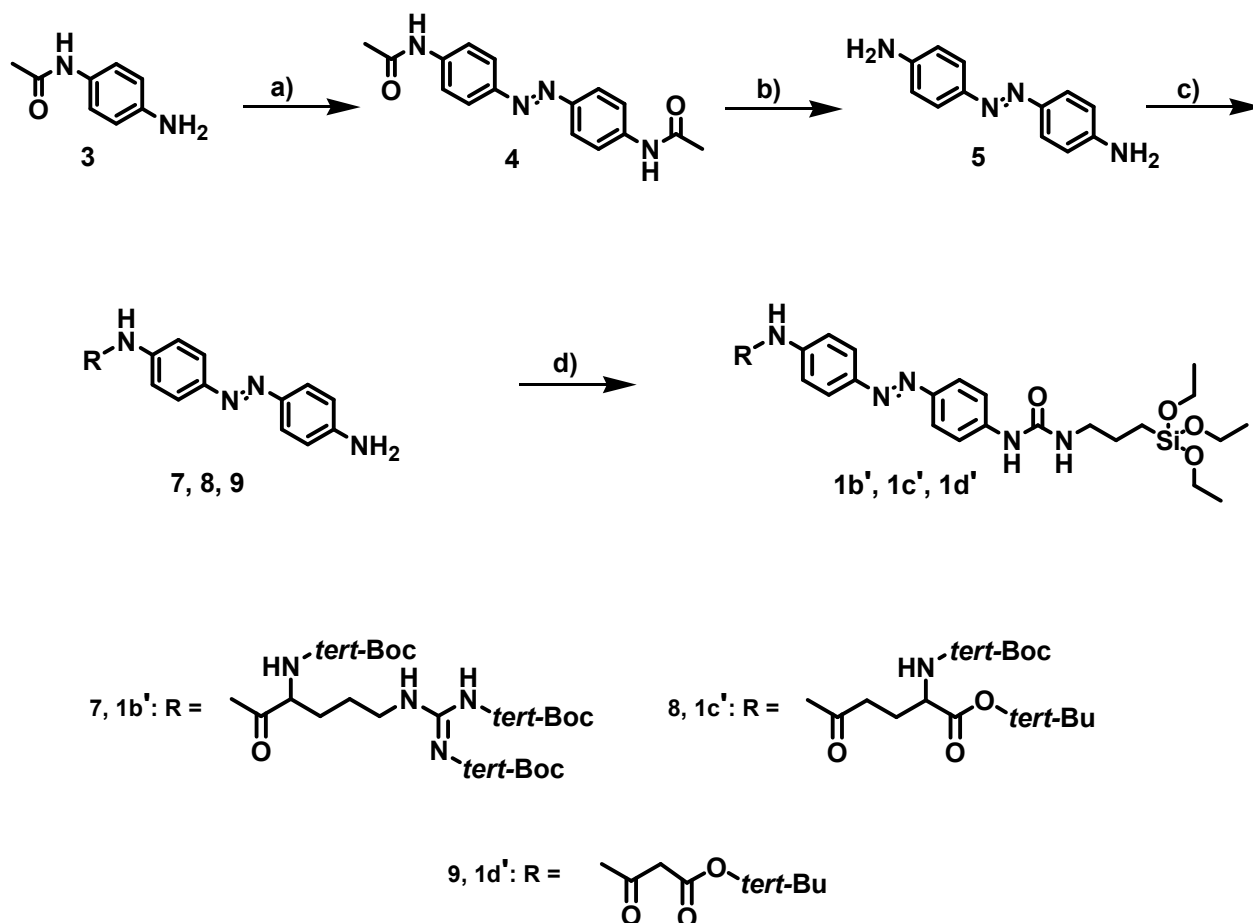
Scheme 1 a) NaBO 3 , H 3 BO 3 , HOAc, HCl, MeOH, 60 °C. b) NaOH. c) For 7 , 1b' = Boc-Arg-(Boc) 2 -OH, for 8 , 1c' = Boc-Glu-(OtBu)-OH and for 9 , 1d' = Mono-tert-butyl malonate, DCC, HOBT, DMF. d) OCN-(CH 2 ) 3 -Si(OEt) 3 , THF.
