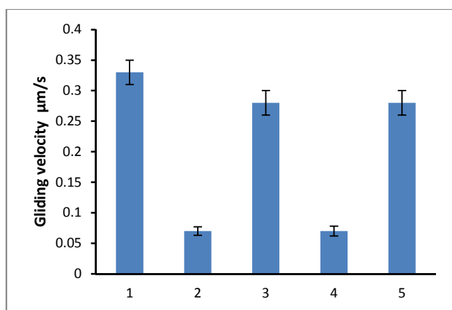
Fig.4 Repeatable changes in the gliding velocity of microtubules in the presence of AzoTP (3 mM) by the alternative UV and visible light irradiations. 1) Before irradiation. 2) After UV (366nm) irradiation for 10 s. 3) After subsequent irradiation at 436 nm for 30 s. 4) After subsequent UV irradiation for 10 s. 5) After subsequent irradiation at 436 nm for 30 s. Error bars represent standard deviations for 10 microtubules.
