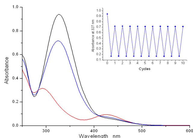
Fig.2 UV-vis absorption spectra of AzoTP ( 5.85 \times 10^{-5} M) in water. (Black line) Before irradiation. (Red line) Photostationary state (PSS) at 366 nm. (Blue line) PSS at 436 nm. Inset: Absorbance changes at 327 nm after the alternative irradiation at 366 nm and 436 nm upto 10 cycles.
