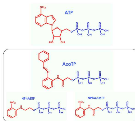
Fig.1 Structures of non-nucleoside triphosphates, AzoTP, NPhAETP and NPhAdMTP in comparison with adenosine triphosphate (ATP).
