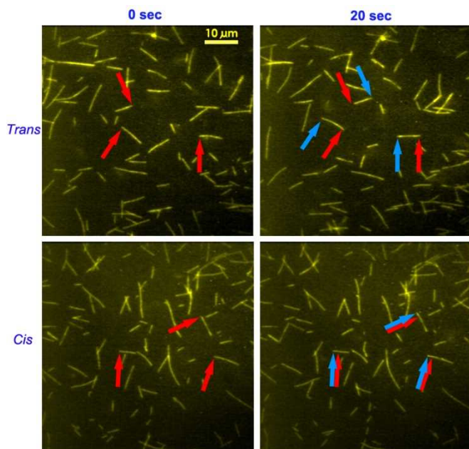
Fig.3 Fluorescence images of the gliding microtubules driven by AzoTP (3 mM) on the kinesin-adsorbed glass surface. (Top) Non-irradiated state at 0 s (left) and 20 s (right), and (bottom) 366 nm irradiated state at 0 s and 20 s in the flow cell. Red arrows indicate the leading points of microtubules at 0 sec and blue arrows indicate the leading points of the same microtubules at 20 sec.
