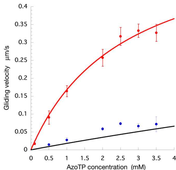
Fig.5 Concentration dependence curves of AzoTP on the gliding velocities of microtubules. Red circles are corresponding to observed gliding velocity for non-irradiated state. Red line represents the fitting curve by Michaelis-Menten equation ( V_{\max} = 0.61 \mu\text{m/s} and K_m = 2.6 \text{ mM} ). Blue circles are the observed gliding velocity for cis -rich states after 366 nm light irradiation. Black line is a theoretical curve derived from the red line for 8% of trans AzoTP. Error bars indicate standard deviations for 10 microtubules.
