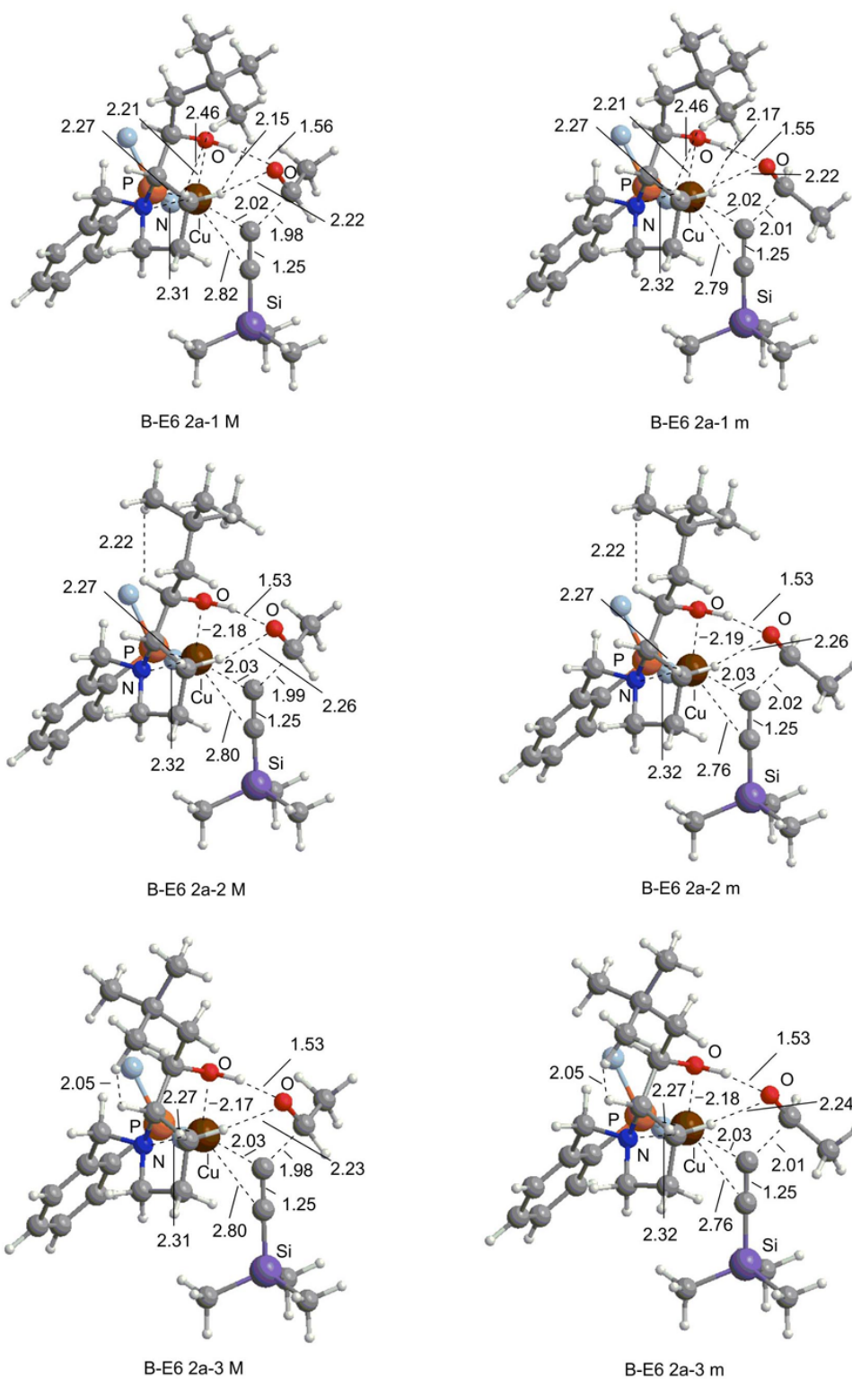
Figure 16. Structures of six-centered TSs of B-E6 conformer for Model-2a (B3LYP/BI). Phenyl groups are shown as right-blue balls for clarity. Atomic distances are shown in Å.
