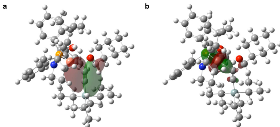
Figure 11. Two representative localized MOs of the six-centered TS B-E6 M for Model-1a (B3LYP/BI).
