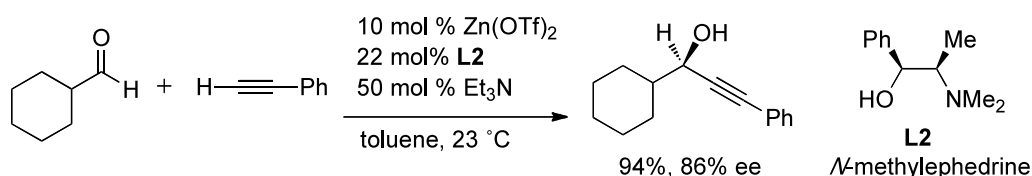
Scheme 11. Zn-catalyzed alkynylation.
