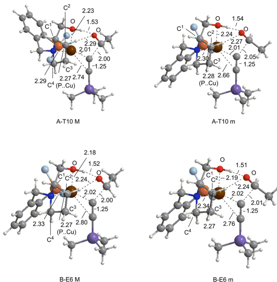
Figure 10. Structures of four most stable six-centered TSs (Model-1a) with A-T10 and B-E6 conformation (B3LYP/BI). Phenyl groups are shown as right-blue balls for clarity. Cu, P, N, Si atoms are shown in brown, orange, blue, and purple, respectively. Atomic distances are shown in Å. The sign “1” after the sign for conformation (e.g. B-E6) means Model-1.
