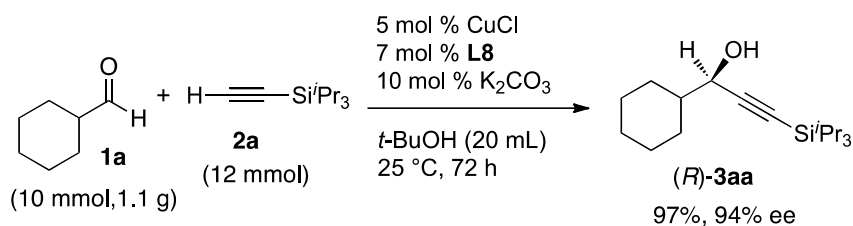
Scheme 2. A gram-scale reaction of 1a and 2a under the glovebox-free conditions.
