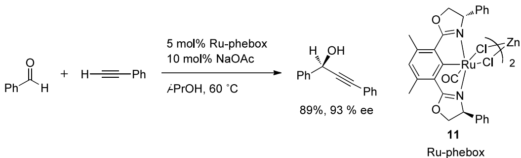
Scheme 15. Asymmetric alkynylation catalyzed by chiral Ru-phebox complex.
