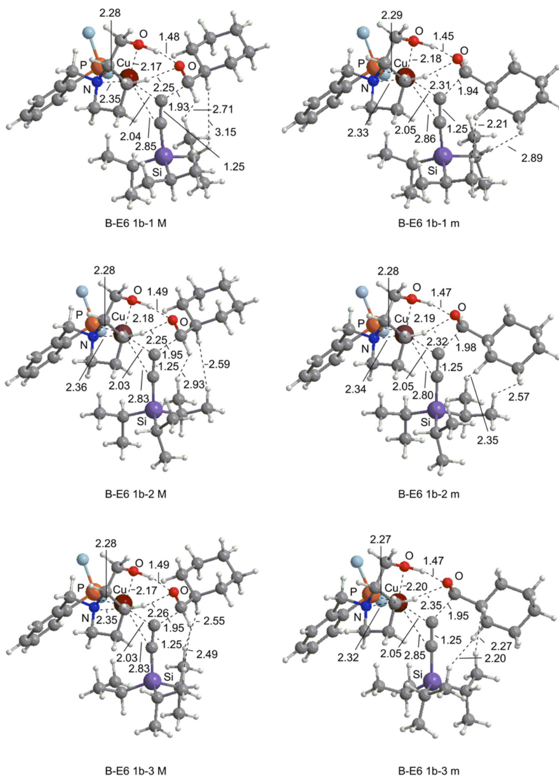
Figure 15. Structures of six-centered TSs for Model-1b with B-E6 conformation (B3LYP/B0). Phenyl groups are shown as right-blue balls for clarity. Cu, P, N, Si atoms are shown in brown, orange, blue, and purple, respectively. Atomic distances are shown in Å.
