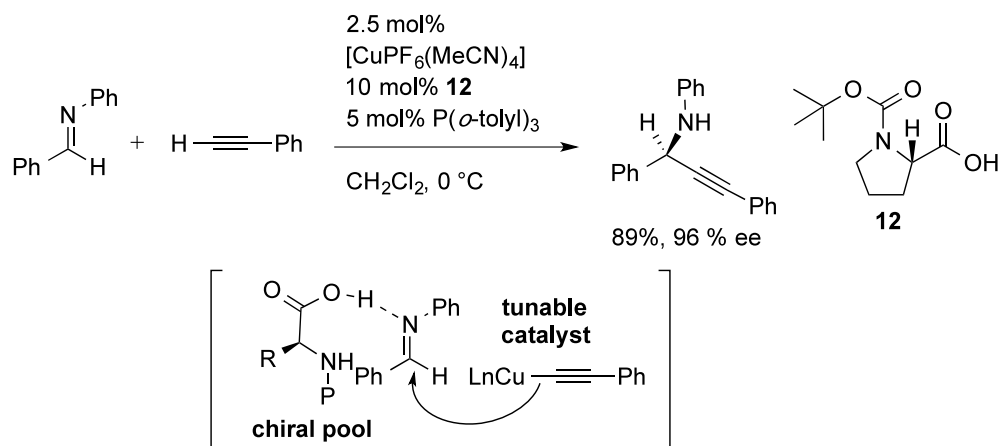
Scheme 17. Asymmetric alkynylations of imines by cooperative hydrogen bonding and Cu catalyst.
