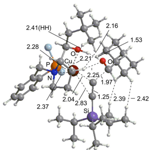
B-E6 2b-1-2-3 M
