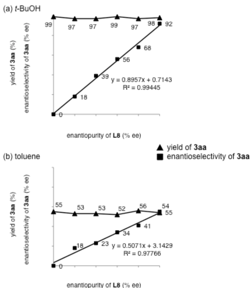
Figure 3. Linear correlation between enantiomeric purity of L8 and enantioselectivity of the reaction between 1a and 2a catalyzed by Cu(O- t -Bu)/ L8 system (10 mol %) at 25°C for 48 h (a) with t -BuOH or (b) with toluene as a solvent.
