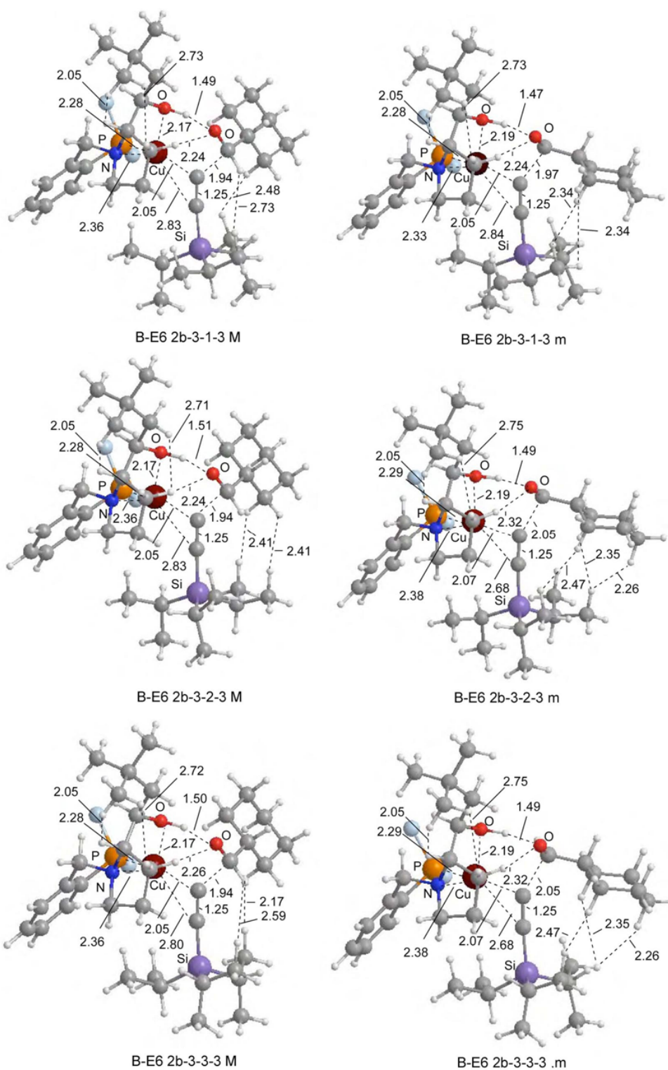
Figure 17. (Part 3) Structures of six-centered TSs for Model-2b with B-E6 2b-x-y-3 conformations (B3LYP/BI). Phenyl groups are shown as right-blue balls for clarity. Cu, P, N, Si atoms are shown in brown, orange, blue, and purple, respectively. Atomic distances are shown in Å.
