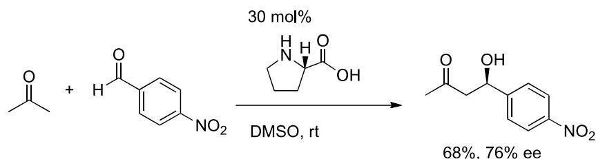
Scheme 7. Proline-catalyzed enantioselective aldol reaction.
