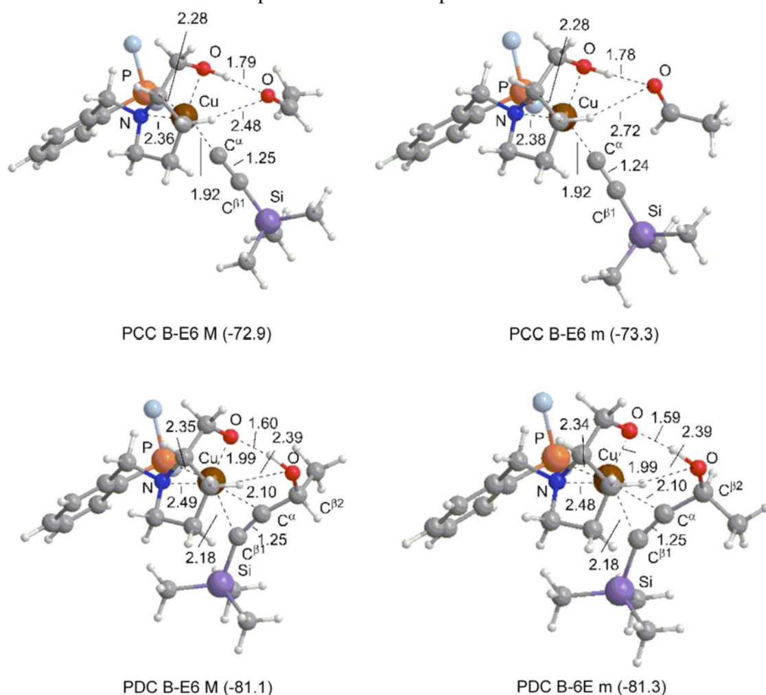
Figure 12. Structures of B-E6 conformers of precursor and product complexes for Model-1a (B3LYP/BI). The Gibbs energies in kJ/mol are relative to TS B-E6 M. Phenyl groups are shown as right-blue balls for clarity. Atomic distances are shown in Å.
