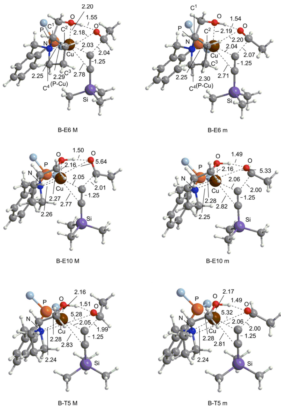
Figure 9. D structures of six-centered TSs for Model-1a optimized at the B3LYP/B0 level. Phenyl groups are shown as light-blue balls for clarity. Atomic distances are shown in Å.
