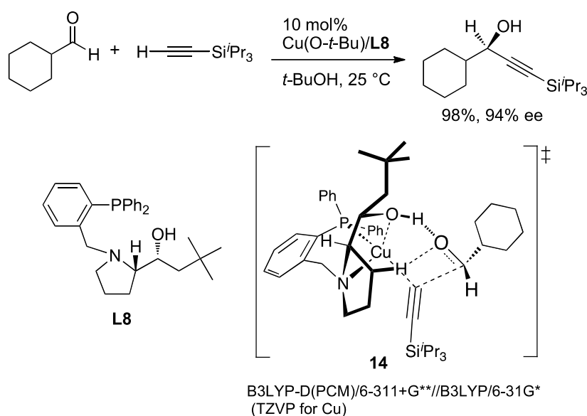
Scheme 20. Cu-hydroxy amino phosphine complex catalyzed enantioselective direct alkynylation of aldehydes with terminal alkynes.
