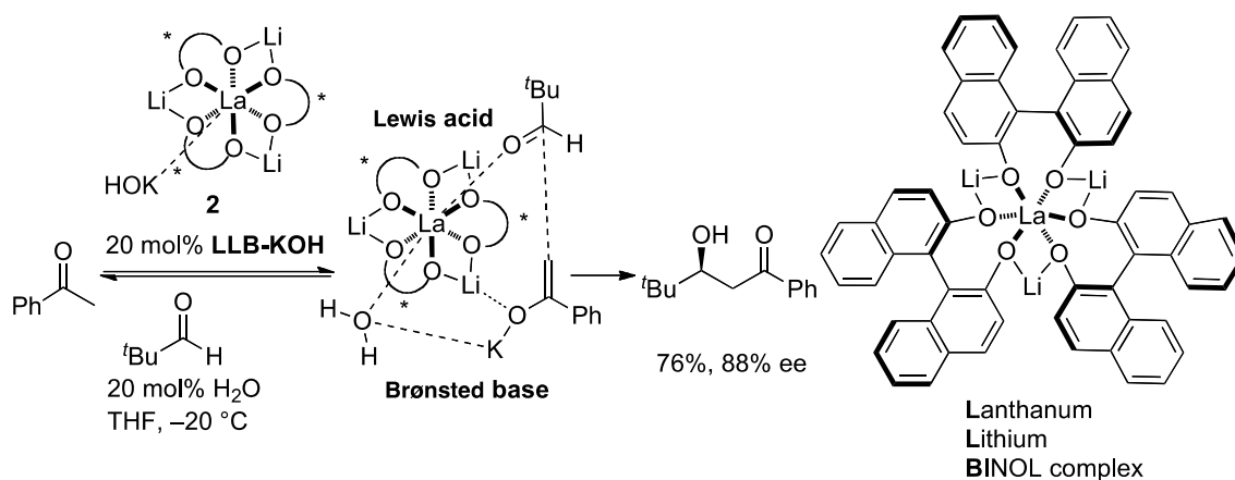
Scheme 3. Catalytic direct asymmetric aldol reaction promoted by LLB complex.
