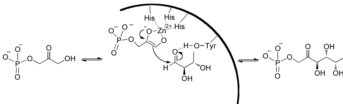
Scheme 1. Model of class II aldolase-promoted enantioselective aldol reaction.
