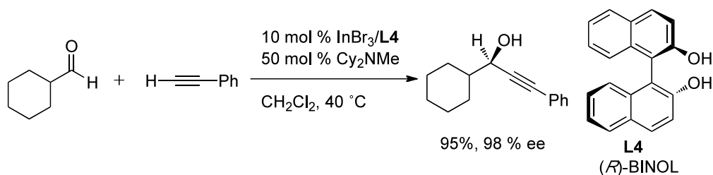
Scheme 13. Asymmetric alkynylation of aldehyde catalyzed by an In/BINOL complex.
