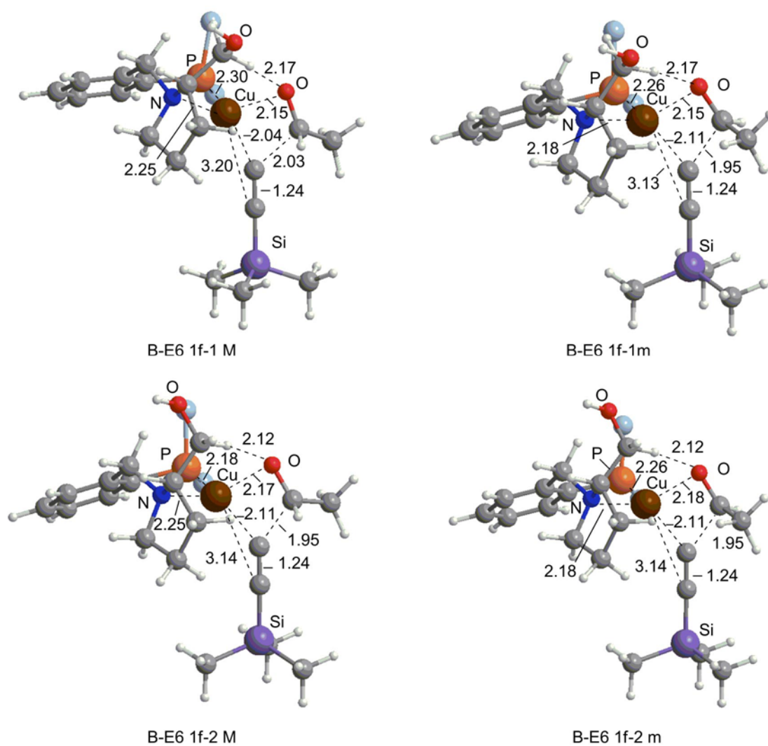
Figure 14. Structures of four-centered TSs of B-E6 conformer for Model-1f (B3LYP/B0). Phenyl groups are shown as right-blue balls for clarity. Atomic distances are shown in Å.
