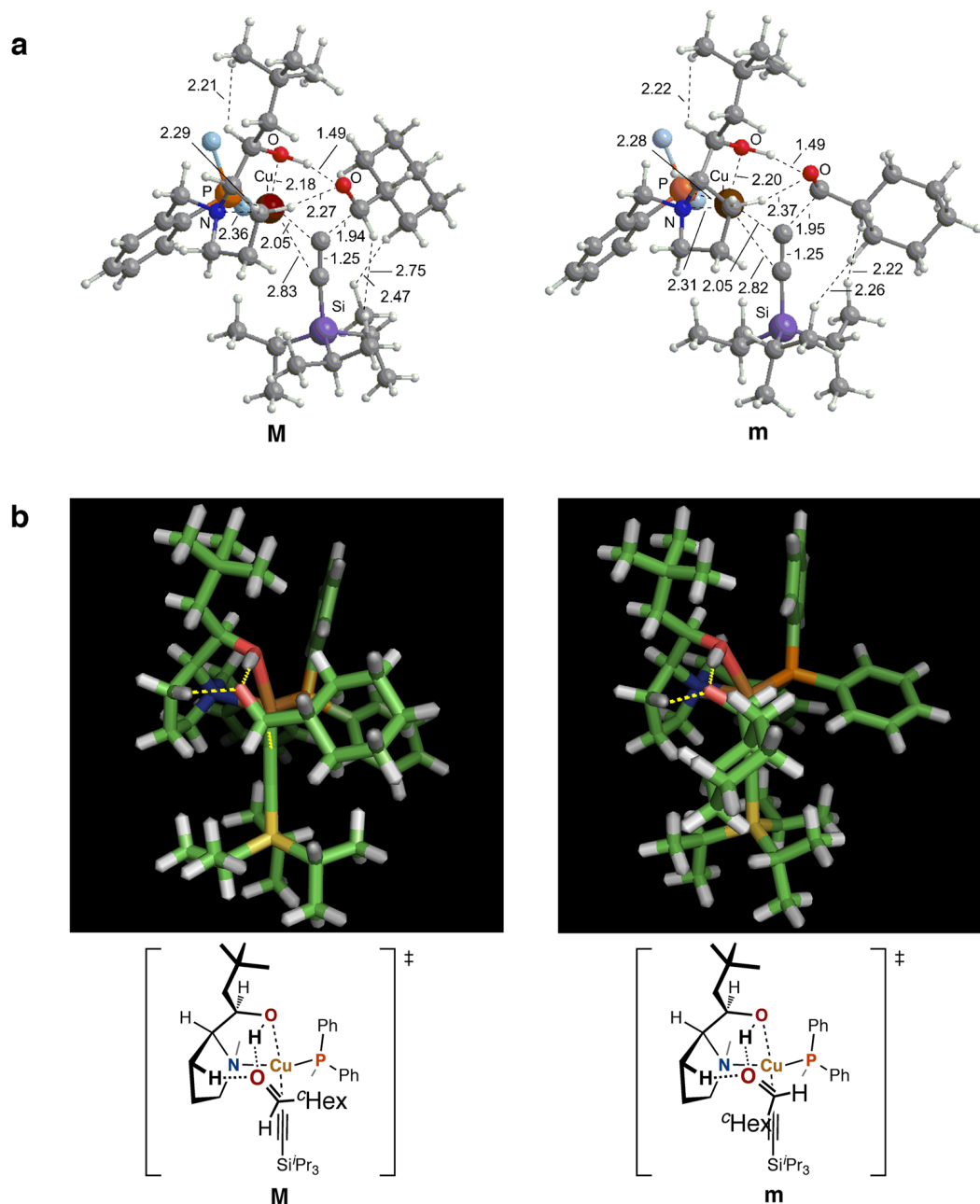
Figure 6. The most stable structures of M (major) and m (minor) transition states for Model-2b [ L8 , c -HexCHO ( 1a ), -C \equiv CSi- i -Pr 3 ( 2a-H )]. a) Side views. Phenyl groups are shown as light-blue balls for clarity. b) Views (from the front) from the plane of the aldehyde along the developing C–C bond.
