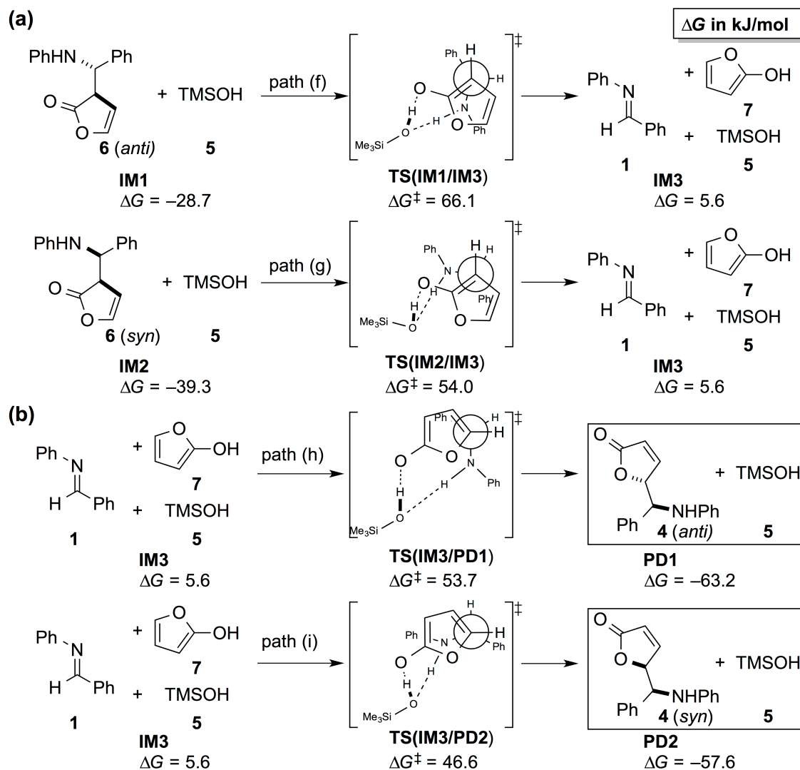
Figure 4. Four pathways obtained by the AFIR search. PD, IM, and TS stand for product (separately optimized two molecules), intermediate (separately optimized two or three molecules), and transition state, respectively. Gibbs free energy \Delta G (298.15 K, 1 atm) based on M06-2X calculations (see text) relative to RT (separately optimized three reactant molecules) is presented in kJ/mol.
