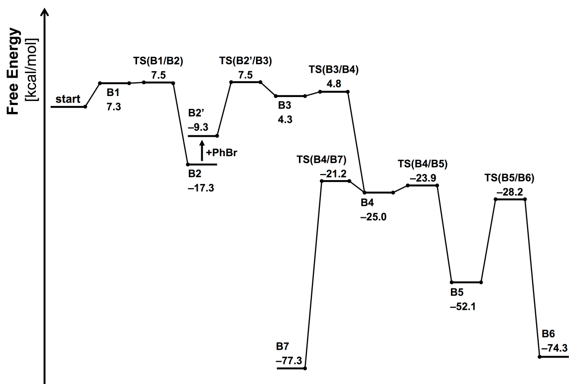
Figure S2-2. Reaction Pathways Leading to the B/Si Products for 3b
