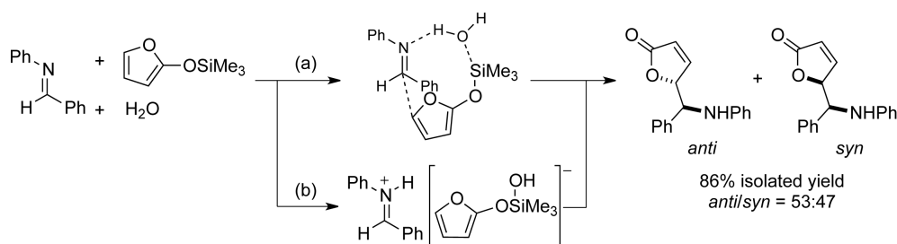
Scheme 1. Palusible Reaction Pathways
