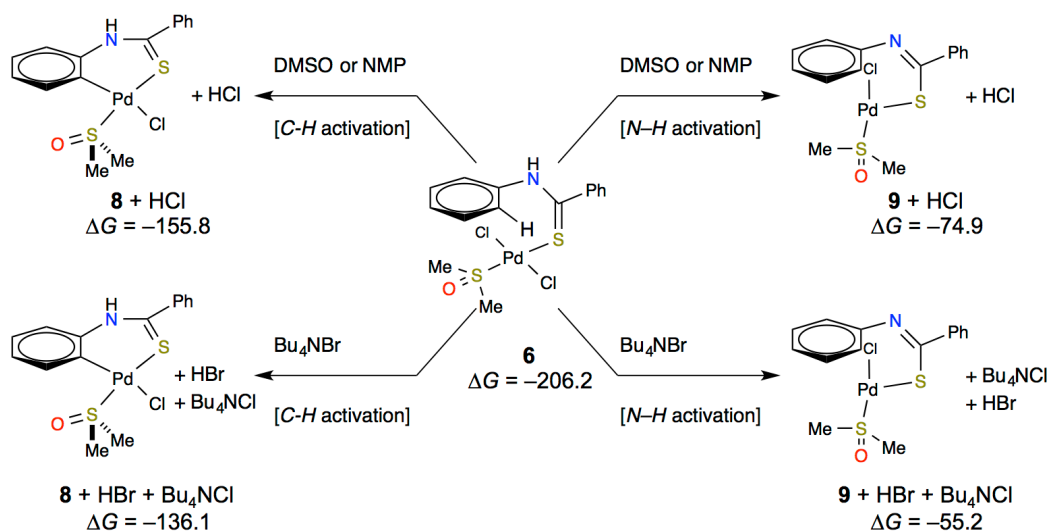
Figure 2. Thermodynamic Stability of C–H or N–H Activated Intermediates. Free Energies ( \Delta G ) Relative to the Reactants (i.e., 1 , 2 , 3 , 5 and 7 ) in kJ/mol.
