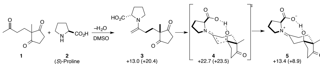
Scheme 1. The proposed rate-limiting step in Hajos-Parrish reaction. Gas-phase energy values based on B3LYP/6-31+G(d,p)//B3LYP/6-31G(d) calculations relative to the reactant (i.e. 1 and 2 ) are shown in kcal/mol. Values in parentheses include solvation energies based on HF/6-31+G(d,p) in DMSO (PCM model & UAKS radii)//B3LYP/6-31G(d) calculations.
