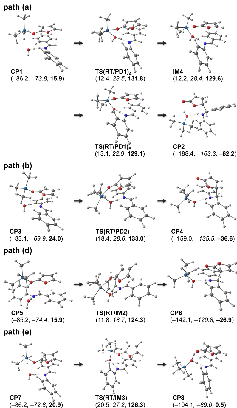
Figure S1-1. Optimized complex (CP) and transition state (TS) structures for the reaction 1 + 2 + 3 , at the M06-2X level (see main text for basis sets)
