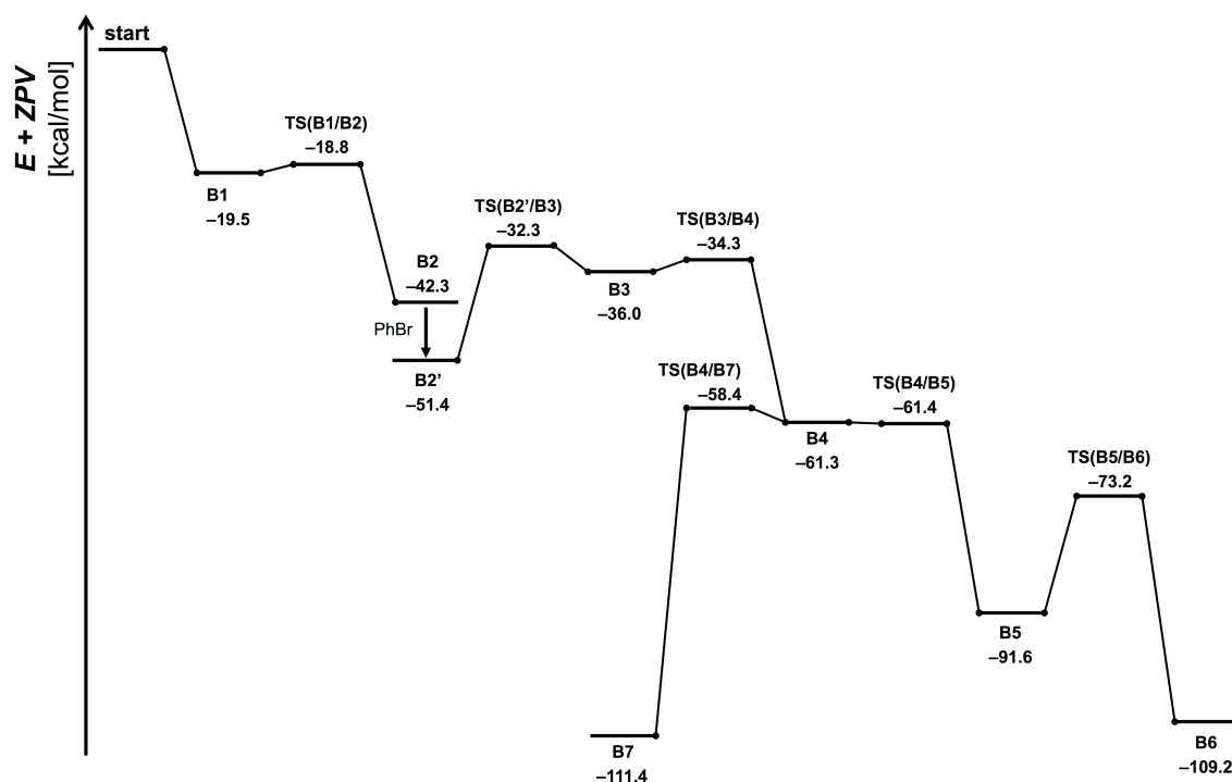
Figure S3-2. Reaction Pathways Leading to the B/Si Products for 3b
