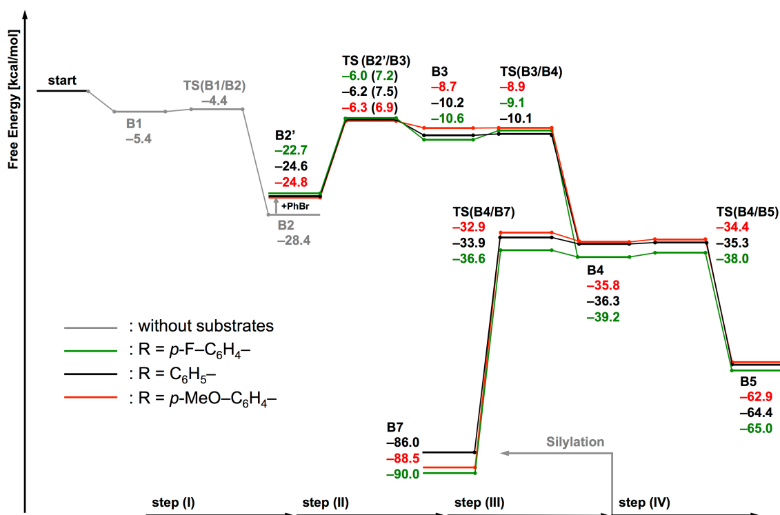
Figure S5-4. Reaction Pathways Leading to the B/Si Products with Different Substrates R–Br ( R = p\text{-FC}_6\text{H}_4 and p\text{-MeOC}_6\text{H}_4 )
