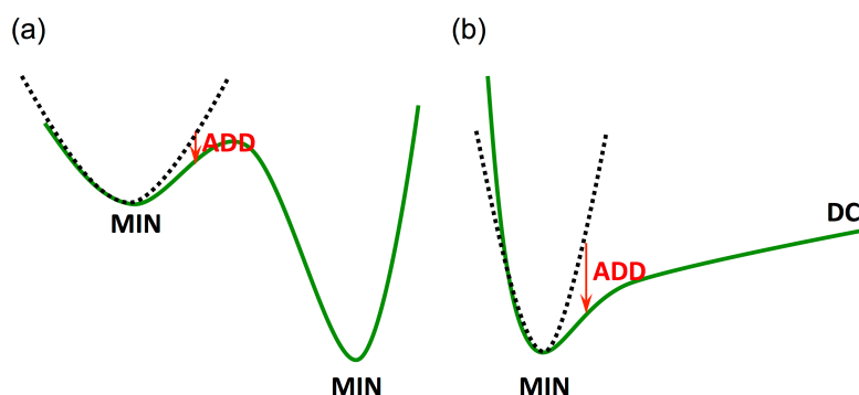
Figure 1. Anharmonic downward distortion from harmonic potential at equilibrium structure (MIN): (a) model potential corresponding to bond rearrangement; (b) model potential connecting to dissociation channel (DC)
