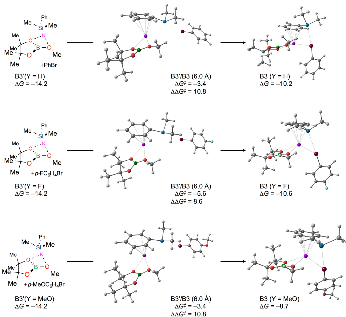
Figure S6-3. Free Energies at a Point along Coordination Coordinates of p -Y- C_6H_4 -Br (Y = H, F, and MeO) to B3
