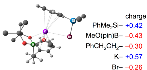
Figure S7. Ball-and-stick Representation of the Charge Distribution in the Intermediates Formed from A2' to A5 and B2' to B5
