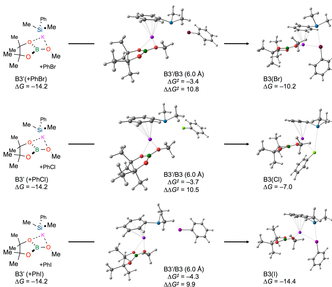
Figure S6-2. Free Energies at a Point along Coordination Coordinates of Ph-X (X = Br, Cl, and I) to B3
