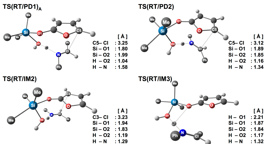
Figure 2. Ball-and-stick illustrations of optimized TS structures for the first step (see Figure 1 for corresponding schematic representations). Important bond distances (in Å) are also shown. Methyl and phenyl groups are simplified and represented by one carbon atom for clarity.
