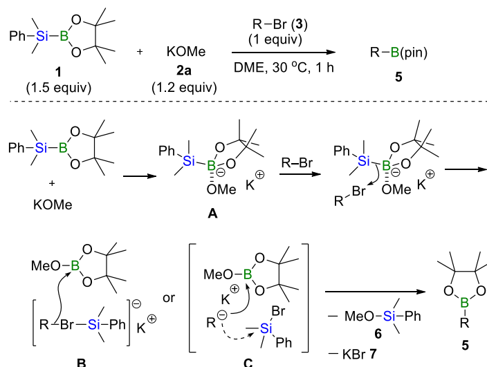
Scheme 1. Proposed Reaction Mechanism of Formal Boryl Substitution of Organic Bromine Compounds ( R = \text{Aryl or Alkyl} ) with Silylborane and Alkoxy Base
