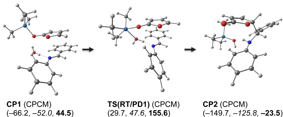
Figure S3. Optimized complex (CP) and transition state (TS) structures for the concerted path to the 4 ( anti ) in C-PCM-water solvent, at the M06-2X level (see main text for basis sets)
