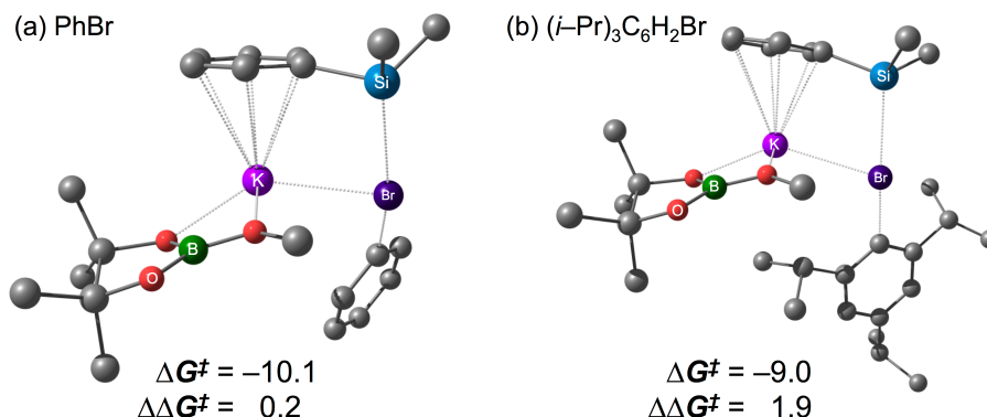
Figure 4. TS Structures, Free Energies ( \Delta G^\ddagger ) Relative to the Reactants ( 1 , 2a and 3b/3c ), and Activation Free Energies ( \Delta\Delta G^\ddagger ) for the Halogenophilic Attack Reaction Steps. Free energy values (303.15 K, 1.0 atm) based on M06-L/6-311+G(2d,p) calculations are given in kcal/mol.
