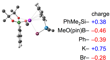
Figure S7. Ball-and-stick Representation of the Charge Distribution in the Intermediates Formed from A2' to A5 and B2' to B5
