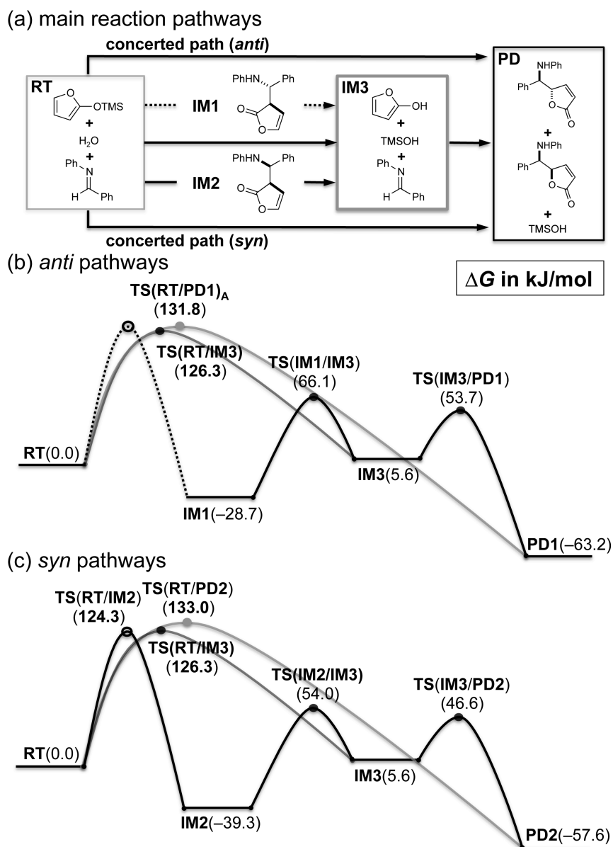
Figure 6. The full reaction mechanism of the present vinyllogous Mannich-type reaction. Panel (a) presents main pathways in this reaction. Panels (b) and (c) represent free energy profiles leading to the anti - and syn -products, respectively.
