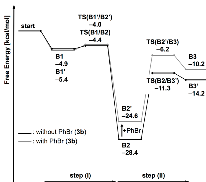
Figure S4-2 Reaction Pathways Leading to the Silyl Potassium Intermediate with and without PhBr ( 3b )
