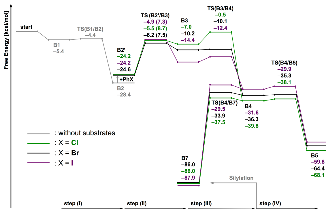
Figure S5-2. Reaction Pathways Leading to the B/Si Products with Different Substrates Ph-X (X = Cl and I)
