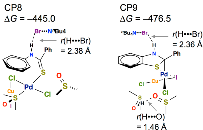
Figure 5. The Most Stable Structures of Intermediate in CP8 (=CP4 \cdots\mathbf{15} ) and CP9 (=CP7 \cdots\mathbf{15} ) system. Free Energies ( \Delta G ) Relative to the Reactants (i.e., \mathbf{1} , \mathbf{2} , \mathbf{3} , \mathbf{5} , \mathbf{10} and \mathbf{15} ). Free energy values based on B3LYP+D3/6-31G(d,p) & SDD calculations have been given in kJ/mol.
