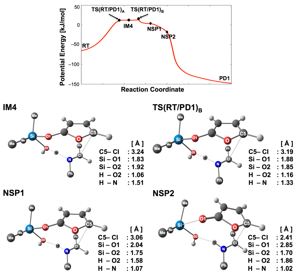
Figure 3. Potential energy (relative to RT) and structural changes along the IRC of path (a). See Figure 2 for the structure of \text{TS(RT/PD1)}_{\text{A}} .
