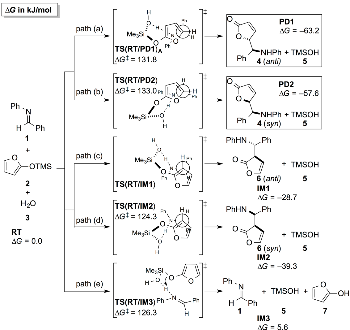
Figure 1. Five pathways obtained by the AFIR search. RT, PD, IM, and TS stand for reactant (separately optimized three molecules), product (separately optimized two molecules), intermediate (separately optimized two or three molecules), and transition state, respectively. Gibbs free energy \Delta G (298.15 K, 1 atm) based on M06-2X calculations (see text) relative to RT is presented in kJ/mol. \text{TS(RT/IM1)} , initially obtained at a low computational level, was not located at the final M06-2X calculation due to very flat potential energy surface in the TS region (see text).
