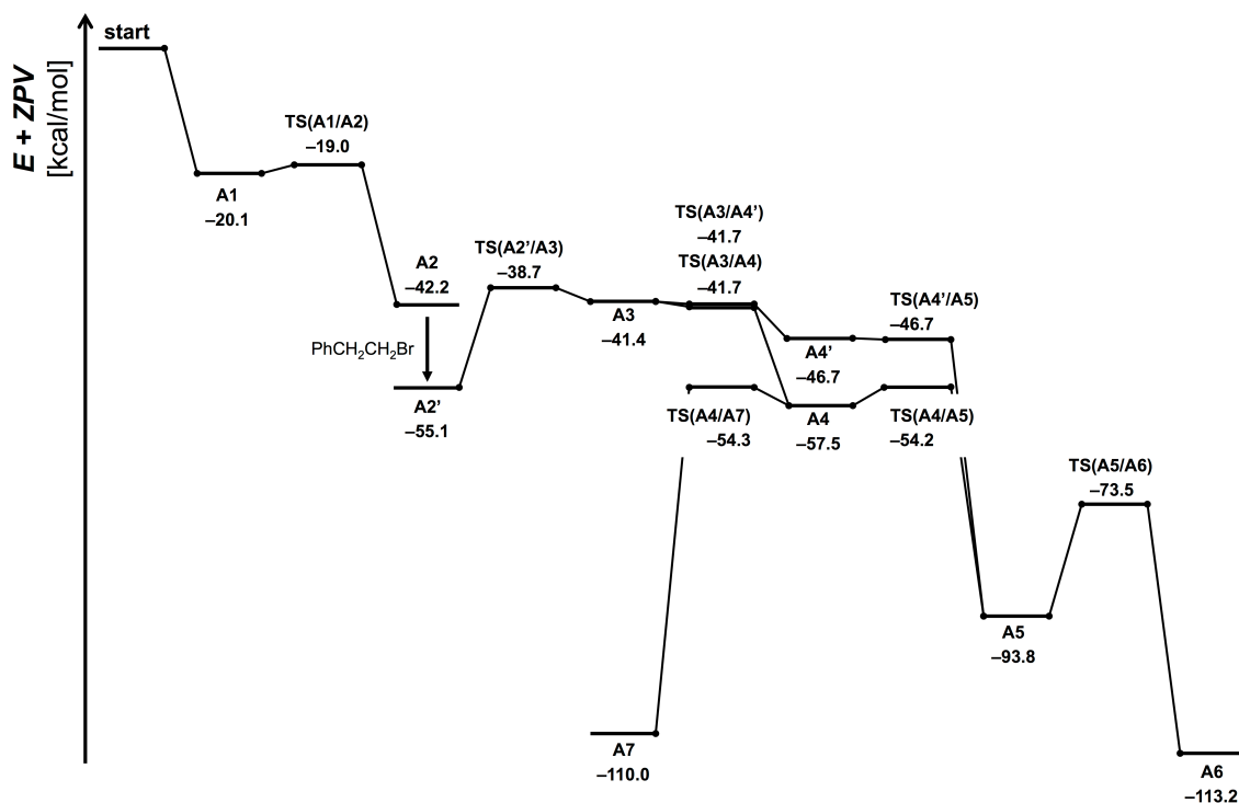
Figure S3-1. Reaction Pathways Leading to the B/Si Products for 3a
