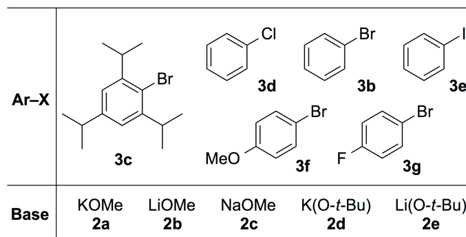
Scheme 4. Aryl Halides and Bases Used in Discussions on the Reactivity of the BBS Method
