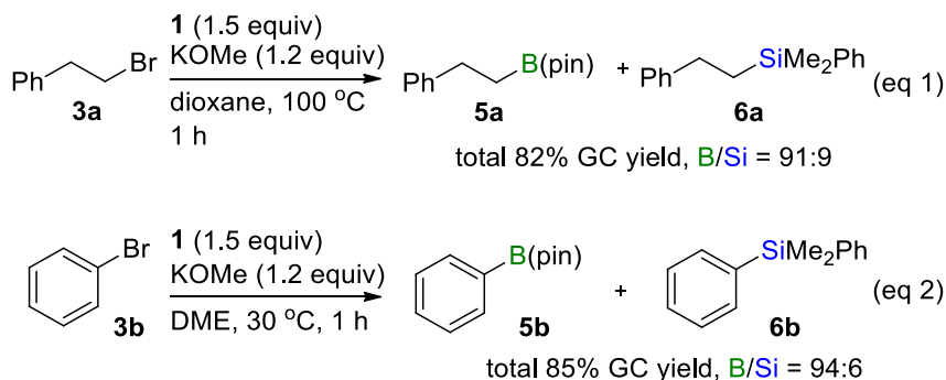
Scheme 2. Boron Substitution Reactions of Compounds 3a and 3b Using the BBS Method
