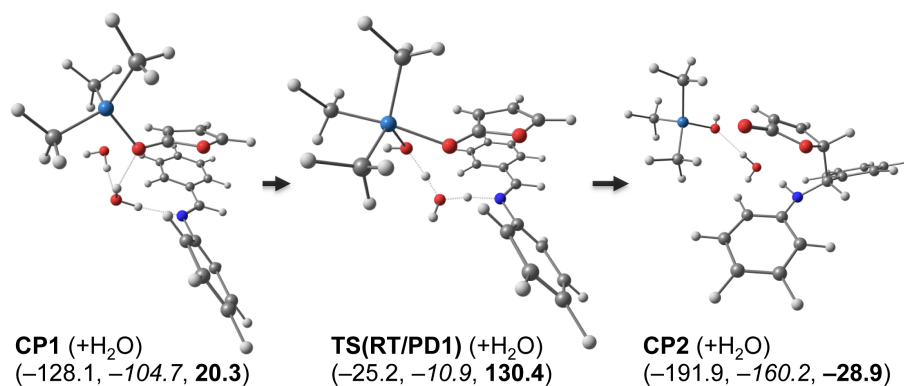
Figure S4. Optimized complex (CP) and transition state (TS) structures for the concerted path to the 4 ( anti ) with a single water catalyst, at the M06-2X level (see main text for basis sets)
