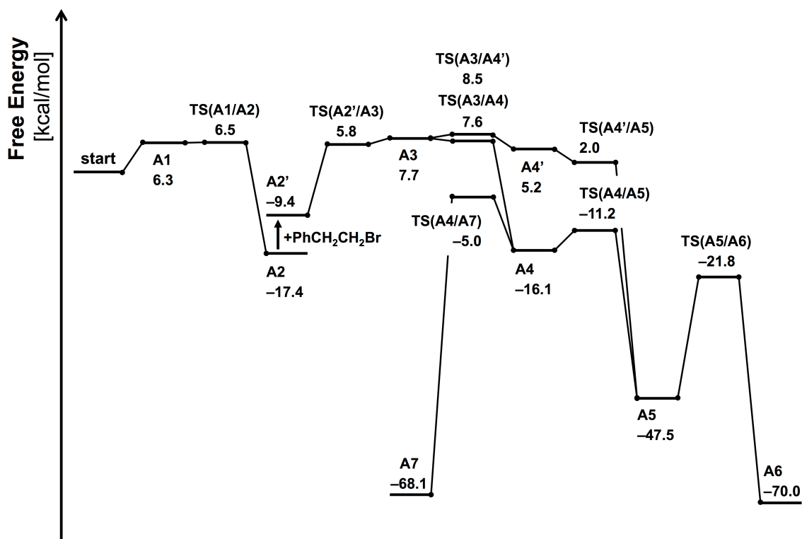
Figure S2-1. Reaction Pathways Leading to the B/Si Products for 3a
