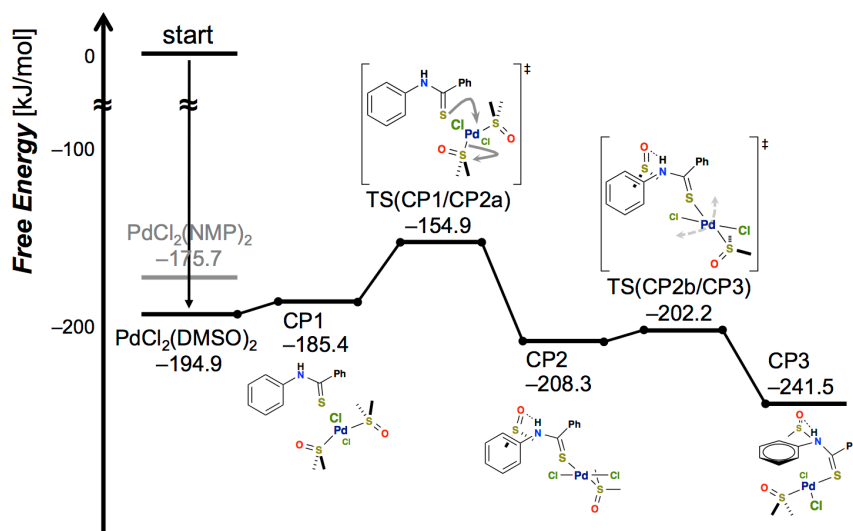
Figure 1. Reaction Pathways Leading to the Reactive Intermediate. The use of “start” corresponds to the reactant (i.e., 1 , 2 , 3 and 5 , which were separately optimized), CP n to an intermediate complex (local minimum), and TS(CP n /CP m ) to the transition state connecting CP n and CP m . Gibbs free energy values (298.15 K, 1.0 atm) based on B3LYP+D3/6-31G(d,p) & SDD calculations relative to the “start” position are shown in kJ/mol. Schematic representations of the optimized structures corresponding to CP n or TS(CP n /CP m ) are shown in the current reaction.
