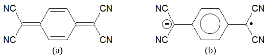
Figure 1.2.5. The structure of TCNQ; (a) the neutral state of TCNQ, (b) the TCNQ anion radical..
