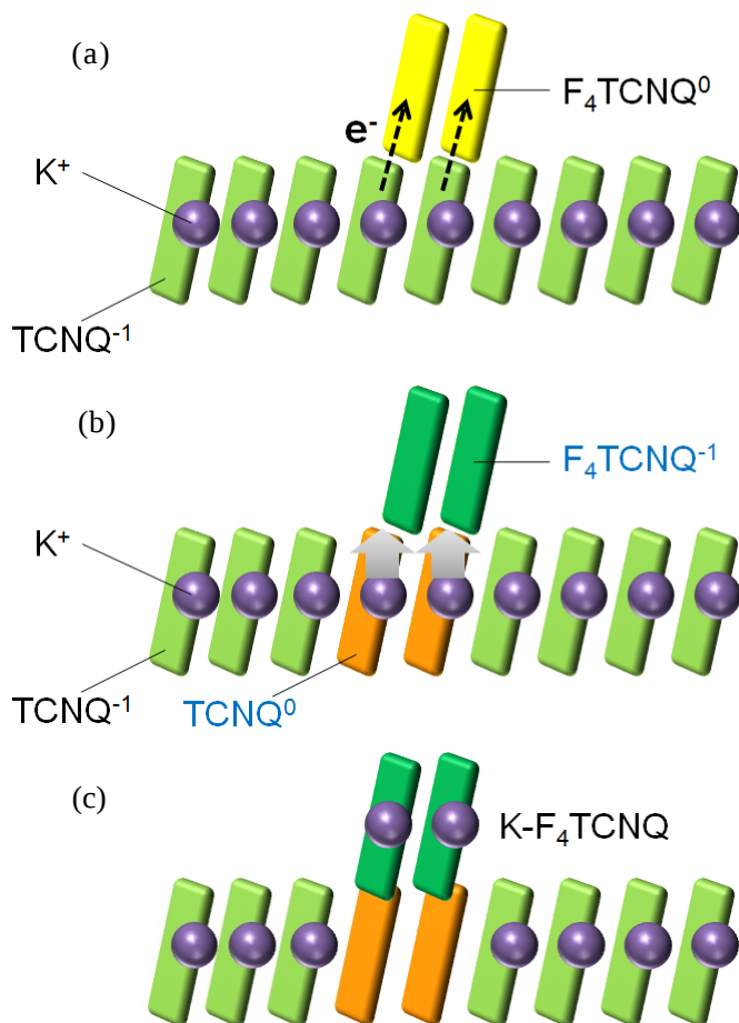
Figure 3.3.5. The mechanism of the hole-doping for K-TCNQ. (a) The hole-doping by F 4 TCNQ for TCNQ -1 . (b) As a result of hole-doping, TCNQ 0 and F 4 TCNQ -1 are generated. (c) K + is extracted to the surface, leading to the formation of K-F 4 TCNQ.
