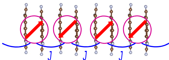
Scheme 2.9. Antiferromagnetic 1-D chain (Bonner-Fisher type) spin model. The red arrows are S = 1/2 spin in the dimeric unit, and all the blue solid curves represent the same scale of exchange interaction ( J ).
