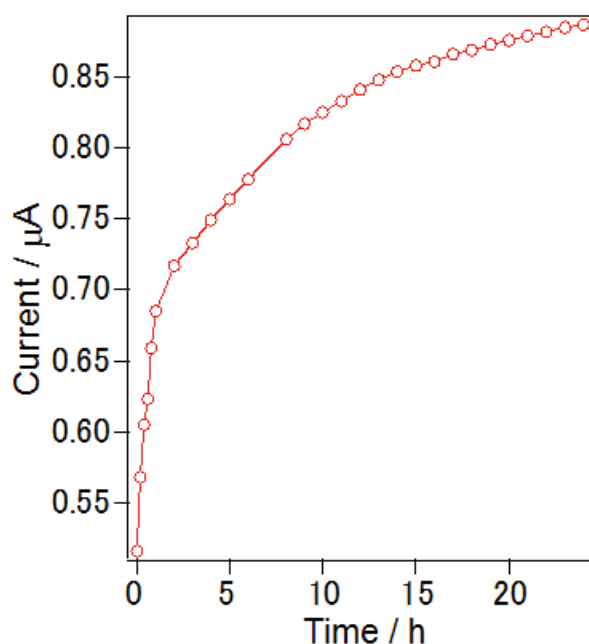
Figure 3.3.2. The time dependence of the current of the K-TCNQ surface after the \text{F}_4\text{TCNQ} contact.
