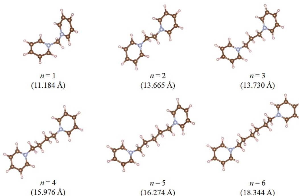
Scheme 2.3. The size of the cations of the optimized structure based on the Gaussian Revision C. 01 MP2/6-31G calculation in the isolated state.
