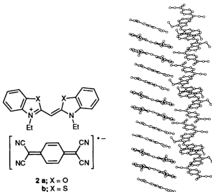
Figure1.3.5. The structural model of the 4,5,4',5'-Dibenzo-3,3'-diethyloxacyanine-TCNQ [19]. The cation component is \pi -conjugated and planar. Thus it can interact with another cation on one side and can also interact with TCNQ anion on the other side, leading to the formation of TCNQ anion dimer and DDAA type stack.
