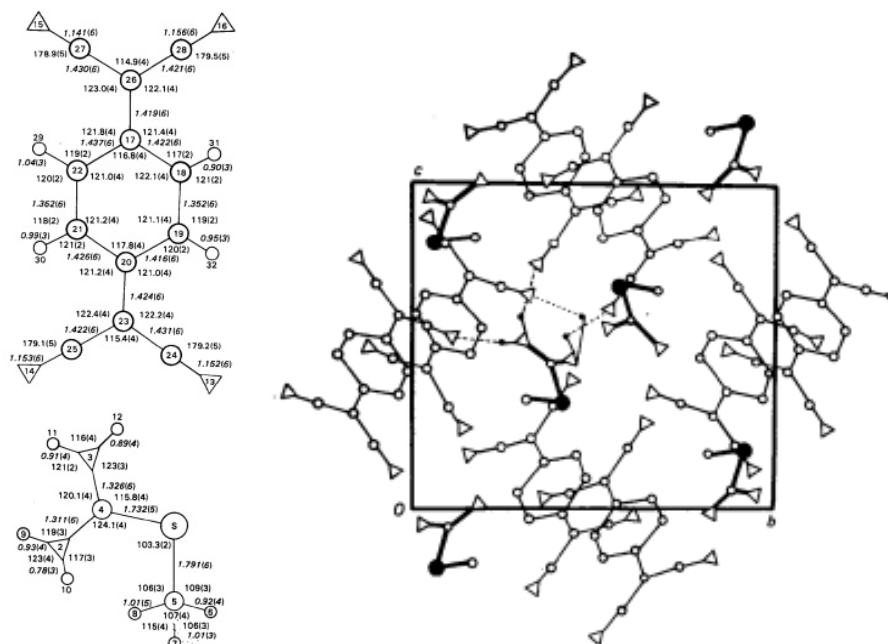
Figure 1.3.7. The structural model of S-Methylthiuronium-TCNQ [24]. The N atom in the TCNQ anion is connected with the H atom in the \text{NH}_2 group included in the cation component. Probably this hydrogen bond network is prior to the \pi - \pi interaction between the TCNQ anions, resulting in the independently located TCNQ anion dimer.
