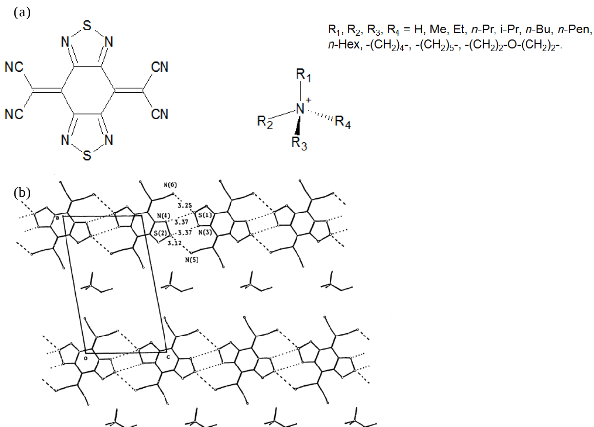
Figure 1.3.9. (a) The structure of BTDA-TCNQ and the ammonium cations. (b) The structural model of the BTDA-TCNQ salt with ethyltrimethylammonium cation [27]. The stoichiometry (cation : BTDA-TCNQ) is 1:1. Each S atom in the thiadiazole ring interacts with two N atoms of the adjacent BTDA anion, resulting in the formation of 2-D network (described as “ribbon-network” in the article).
