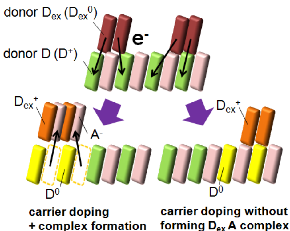
Figure 3.1.6. The electron-doping process for an ionic charge transfer complex.
