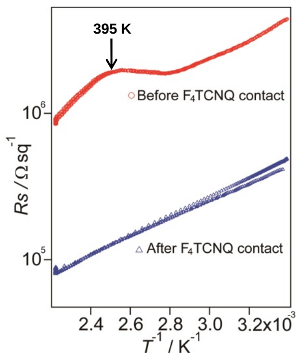
Figure 3.3.8. The sheet resistance of the K-TCNQ surface before and after the F_4\text{TCNQ} contact.
