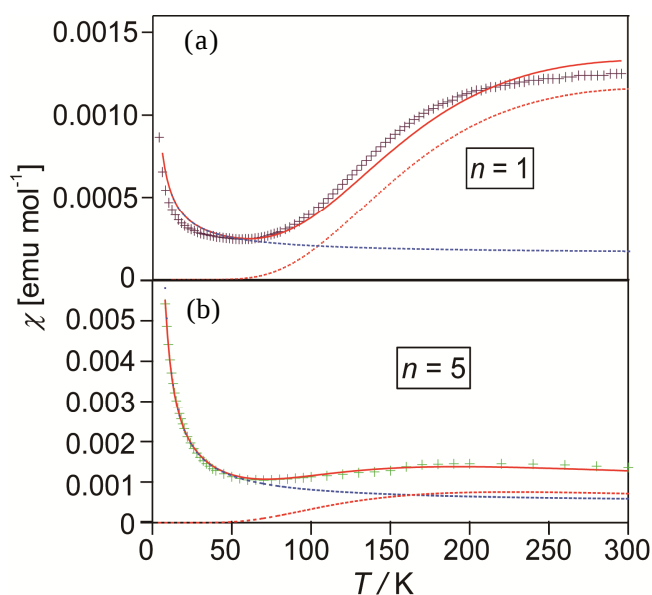
Figure 2.3.14. Magnetic susceptibility of (a) (C1BPy)(TCNQ) 4 and (b) (C5BPy)(TCNQ) 4 . The crosses are the observed values, the red dotted lines are the thermally activated components, the blue dotted lines are the Curie components, and the solid red lines are the best fit of the summation of the thermally activated and Curie components.
