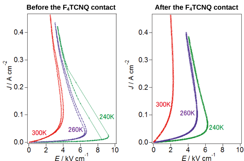
Figure 3.3.10. The negative differential resistance characteristics of the K-TCNQ surface before and after the F 4 TCNQ contact.
