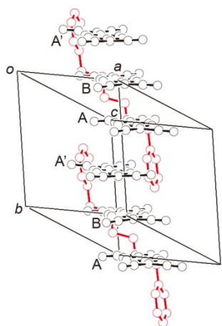
Figure 2.3.5. Perspective view of the unit cell for (\text{C6BPy})(\text{TCNQ})_3 .
