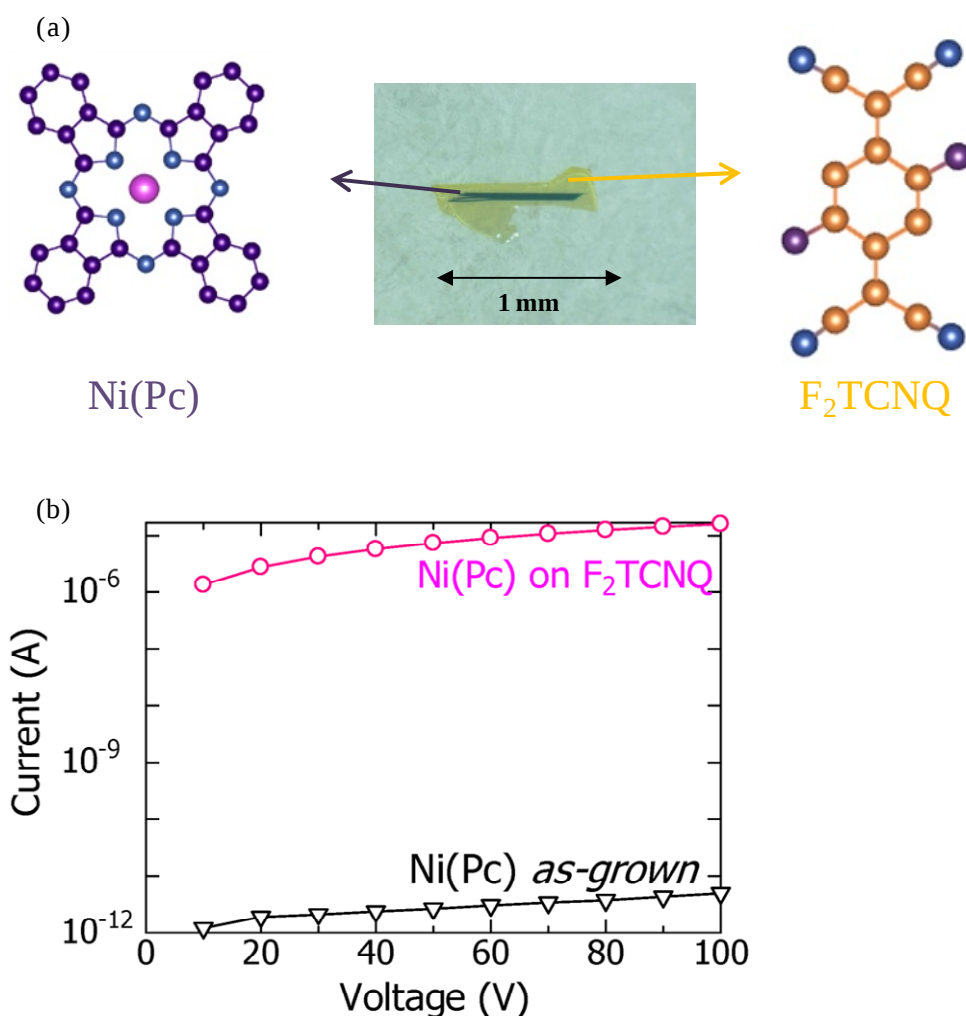
Figure 3.1.3. (a) The contact of NiPc and F 2 TCNQ single crystal. (b) The current increase at the interface of the two crystals.
