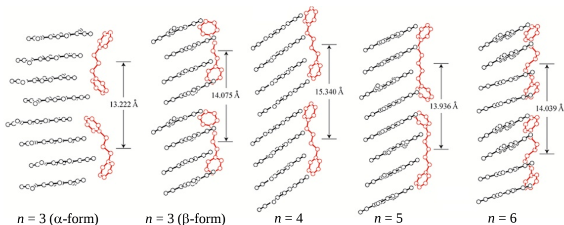
Figure 2.3.2. Effective dication lengths in the 1:4 salts for n = 3, 4, 5 , and 6 .
