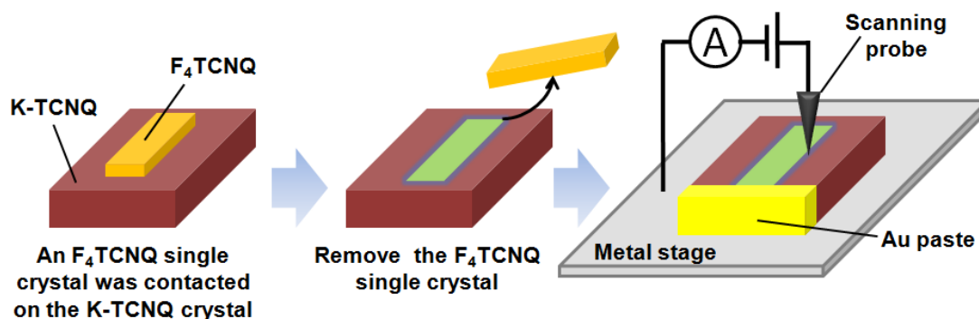
Figure 3.3.6. The fabrication of the boundary between K-TCNQ and K-F 4 TCNQ, and the method to measure the current around the boundary.
