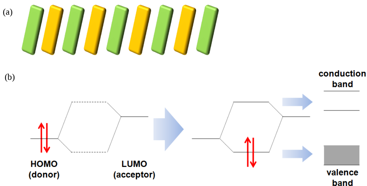
Figure 1.3.1. (a) The model of the mixed-stack structure. Different colors describe different kinds of molecules (donors or acceptors). (b) The energy state of the mixed-stack structure. The left side is before the complex formation, the right side is after the complex formation.
