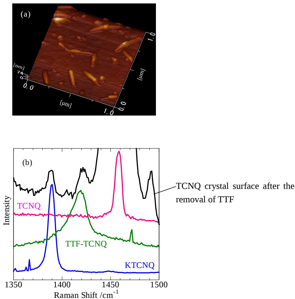
Figure 3.1.2. The AFM image (a) and the Raman scattering spectra (b) of the TCNQ crystal surface after the removal of the TTF powder.
