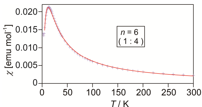
Figure 2.3.13. Magnetic susceptibility of (C6BPy)(TCNQ) 4 . The crosses are the observed values, and the solid lines are the best results of fitting.
