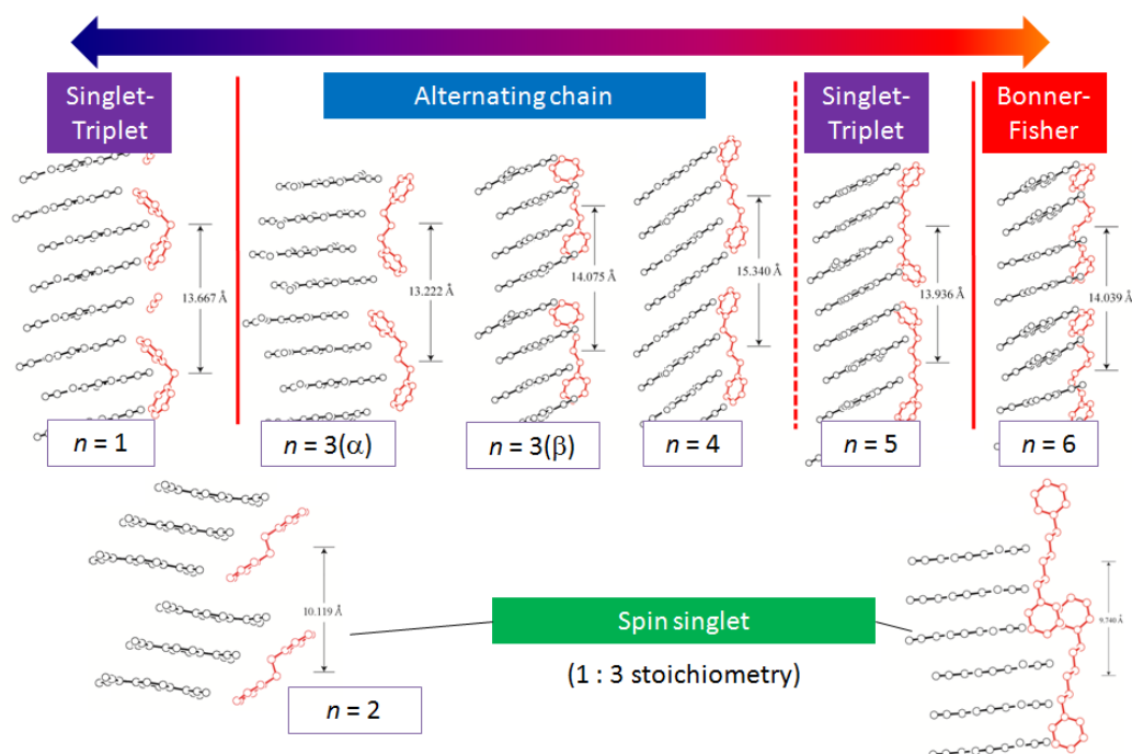
Figure 2.3.15. Correlations between the variations in the magnetic behavior and the size of the dication.
