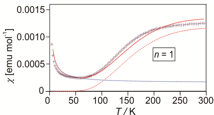
Figure 2.3.8. Magnetic susceptibility of (C1BPy)(TCNQ) 4 CH 3 CN. The crosses are the observed values, and the solid lines are the best results of fitting.
