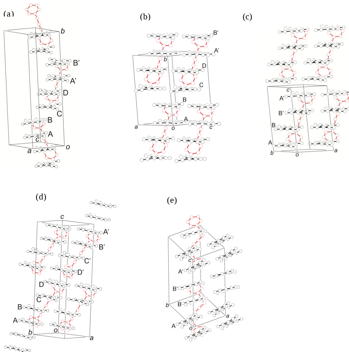
Figure 2.3.1. Perspective view of the unit cell for (a) \alpha -(C3BPy)(TCNQ) 4 (the structure is the same as that reported in ref. [26]), (b) \beta -(C3BPy)(TCNQ) 4 , (c) (C4BPy)(TCNQ) 4 (the structure is the same as that reported in ref. [27]), (d) (C5BPy)(TCNQ) 4 , and (e) (C6BPy)(TCNQ) 4 .
