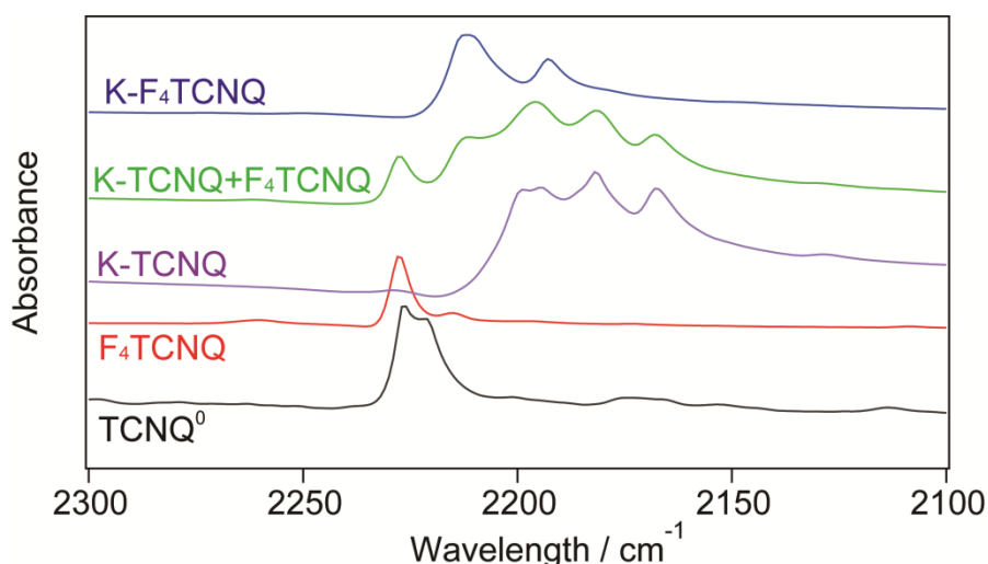
Figure 3.3.3. The IR spectra of TCNQ 0 , F 4 TCNQ 0 , K-TCNQ, the mixture of the K-TCNQ and F 4 TCNQ, and K-F 4 TCNQ.
