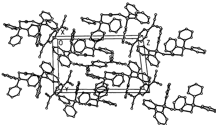
Figure 1.3.3. Packing diagram for [\text{Au}(\text{CH}_2\text{PPh}_3)_2](\text{TCNQ}) [15]. The cation component has bis(triphenylphosphine) structure, and is much larger than TCNQ, leading to the mixed-stack (DADA) structure.
