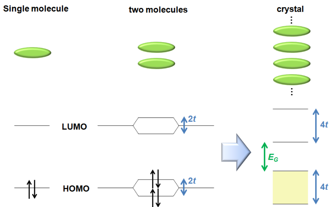
Figure 1.2.2. The energy band diagram of organic crystal.
