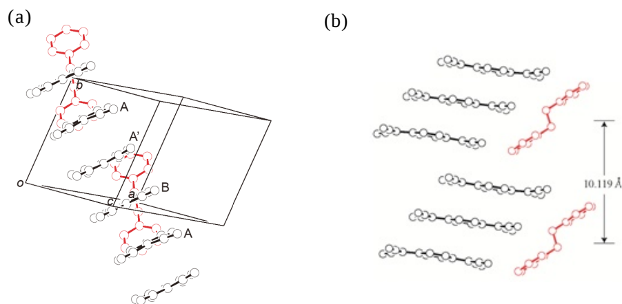
Figure 2.3.4. (a) Perspective view of the unit cell for (C2BPy)(TCNQ) 3 and (b) its side view.
