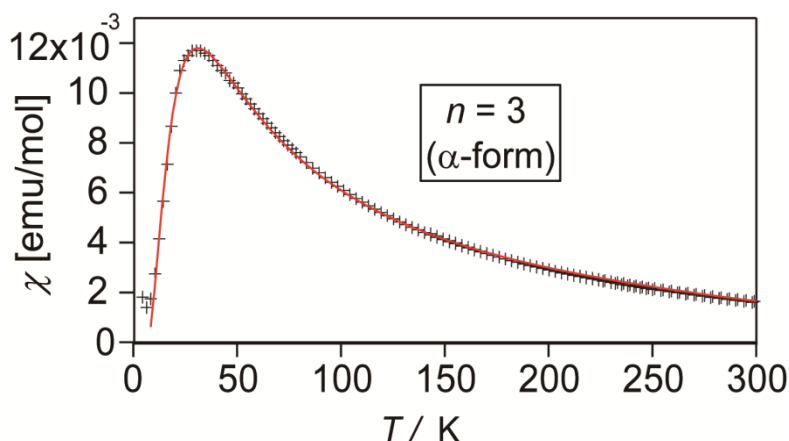
Figure 2.3.9. Magnetic susceptibility of \alpha -(C3BPY)(TCNQ) 4 . The crosses are the observed values, and the solid lines are the best results of fitting.
