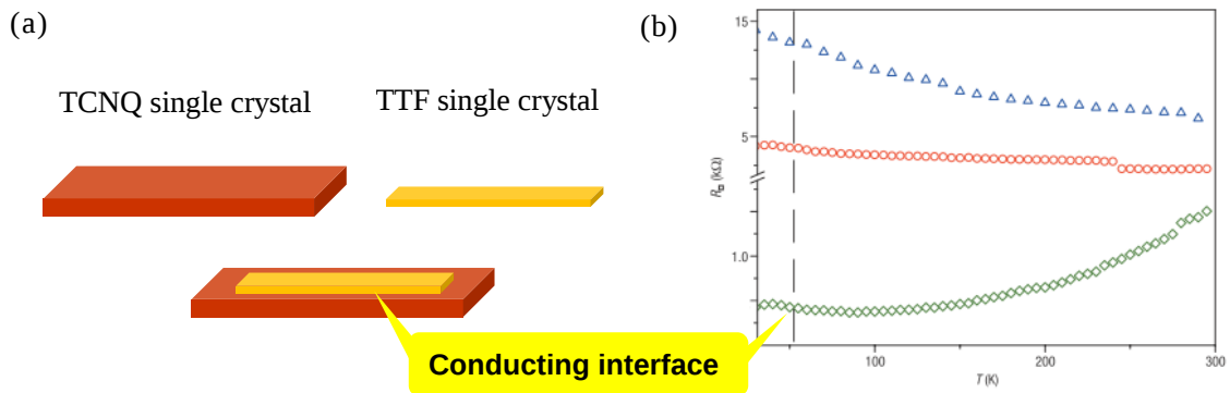
Figure 3.1.1. (a) The initial contact doping with TTF and TCNQ single crystal. (b) The result of the sheet resistance measurement at the interface of the two single crystals.
