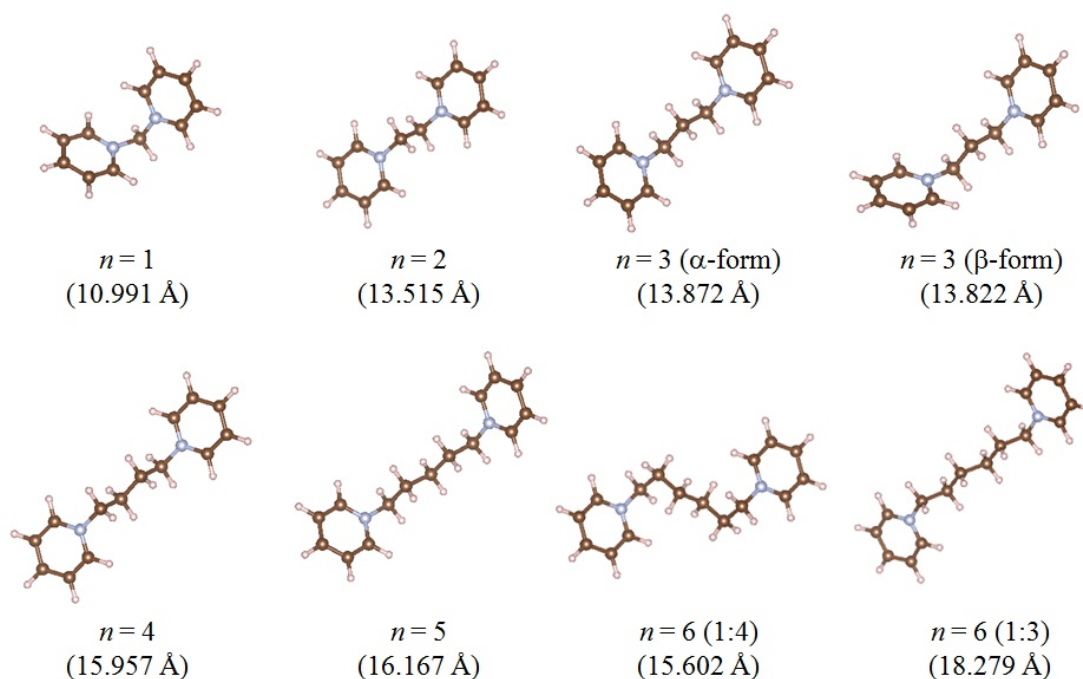
Scheme 2.4. The size of the cations in the TCNQ anion radical crystals.
