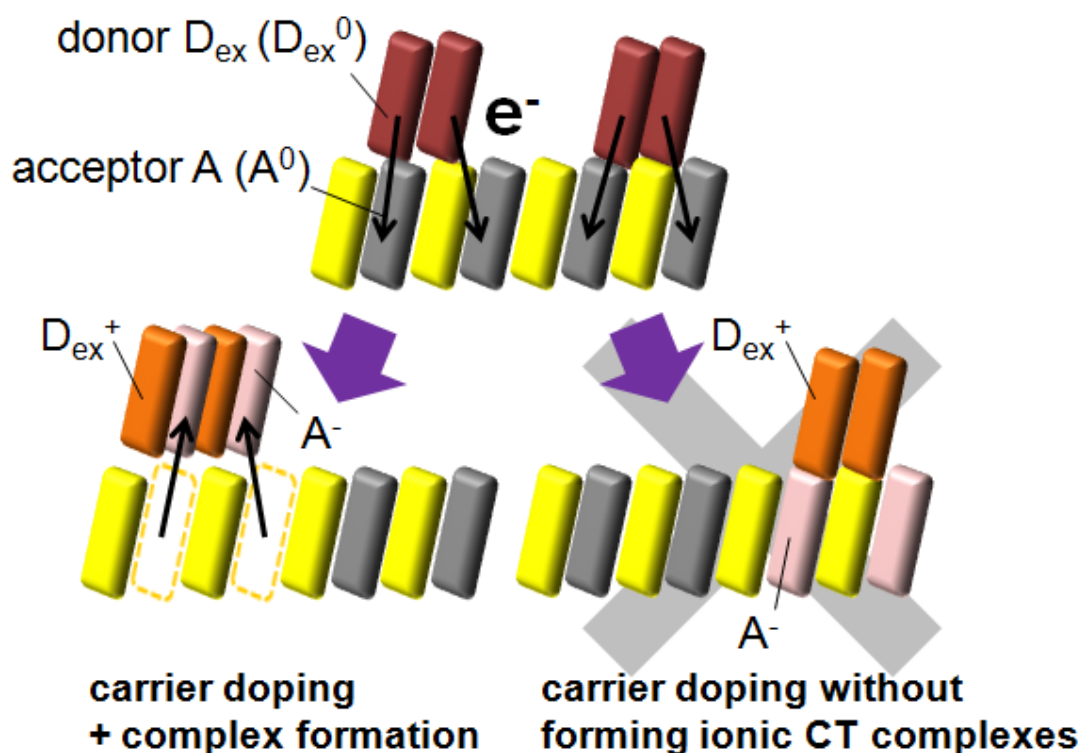
Figure 3.1.5. The electron-doping process for charge transfer complexes with a neutral ground state.
