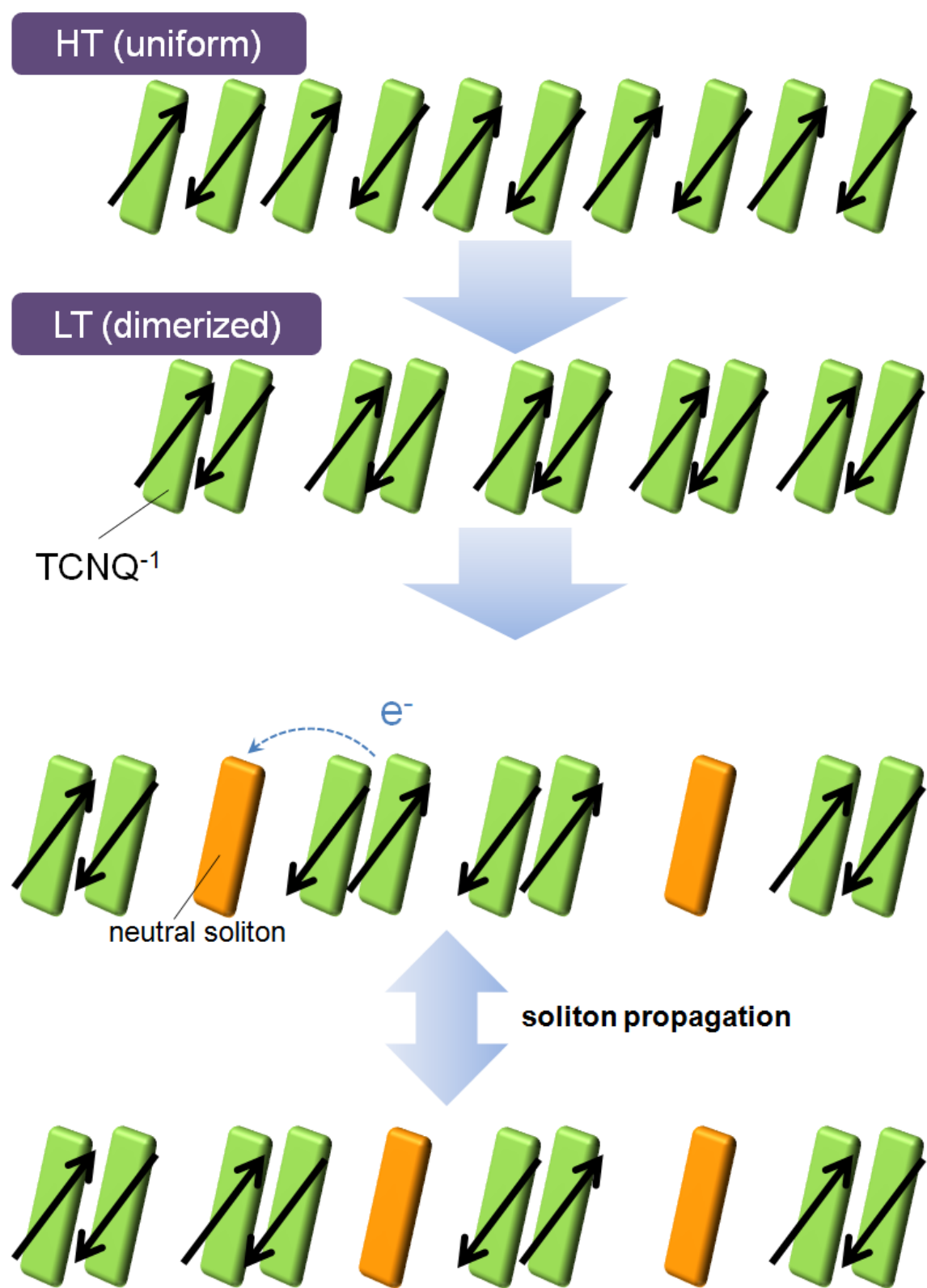
Figure 3.3.9. The effects of the hole-doping for the TCNQ column in K-TCNQ.
