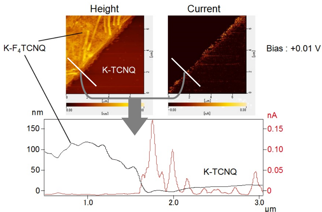
Figure 3.3.7. The AFM images of the height and the current across the boundary between K-F 4 TCNQ and K-TCNQ (described as a white line in the current image).
