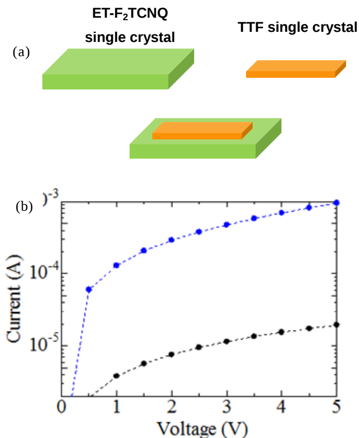
Figure 3.1.4. (a) The contact of ET-F 2 TCNQ and TTF single crystal. (b) The current increase at the interface of the two crystals.
