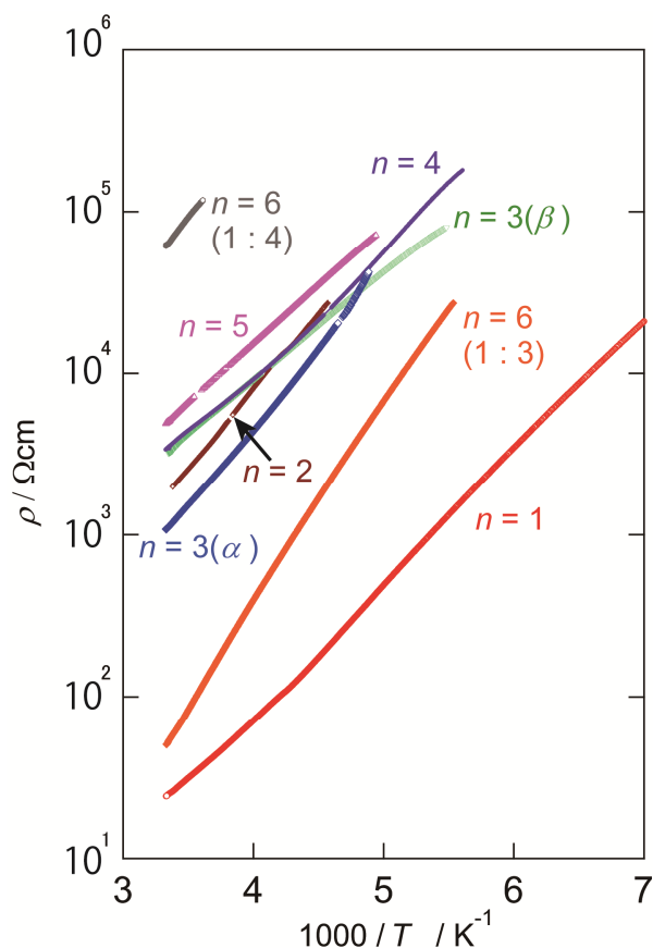
Figure 2.3.6. Temperature dependence of the single-crystal resistivity for the C_n BPy TCNQ salts.
