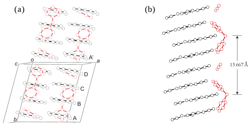
Figure 2.3.3. (a) Perspective view of the unit cell for (\text{C1BPy})(\text{TCNQ})_4 \cdot \text{CH}_3\text{CN} . (b) Effective dication length in (\text{C1BPy})(\text{TCNQ})_4 \cdot \text{CH}_3\text{CN} .
