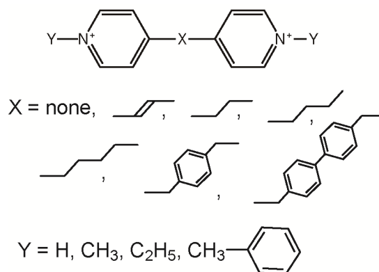
Scheme 2.2 Dications used in the Ashwell's studies.
