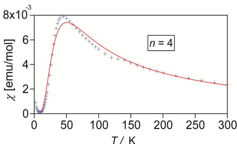
Figure 2.3.11. Magnetic susceptibility of (C4BPy)(TCNQ) 4 . The crosses are the observed values, and the solid lines are the best results of fitting.
