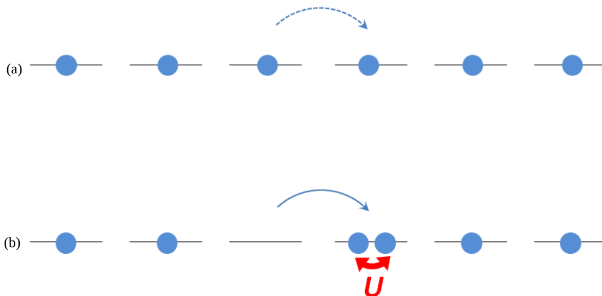
Figure 1.2.3. The model of the on-site Coulomb repulsion in an array of neutral radicals. The blue filled circles describe the electrons, and each horizontal line means the singly occupied molecular orbital (SOMO) of the single neutral radical. (a) The state before the electron transfer, and (b) the state after the electron transfer. The on-site Coulomb repulsion ( U ) operates between the two electrons occupied in the same molecular orbital, which requires extra energy for electron transfer.
