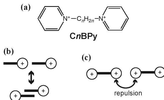
Scheme 2.1. (a) The structure of the target dication(s). (b) The possible model of an interdigitation by using the N -alkyl-pyridinium monocation. (c) The model of coulomb repulsion caused by having the two pyridinium rings close together.
