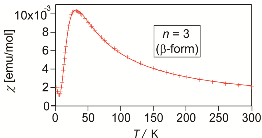
Figure 2.3.10. Magnetic susceptibility of \beta -(C3BPy)(TCNQ) 4 . The crosses are the observed values, and the solid lines are the best results of fitting.
