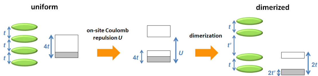
Scheme 2.5. The band structural model of the 1/4-filled TCNQ column.
