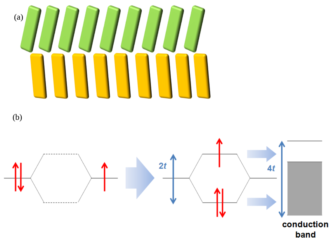
Figure 1.3.2. (a) The model of the segregated-stack structure. Different colors describe different kinds of molecules (donors or acceptors). (b) describes the energy state of the segregated-stack structure with the degree of charge transfer being 1/2. The left side is before the complex formation, the right side is after the complex formation.
