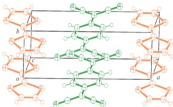
Figure 1.2.6. The crystal structure of TTF-TCNQ.
