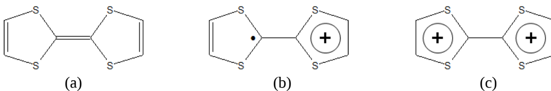
Figure 1.2.4. The structure of TTF. (a) The neutral charge state of TTF, (b) the TTF cation radical, (c) the dicationic state of TTF.
