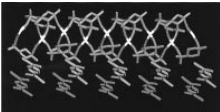
Figure 1.3.4. The structural model of the TCNQ salt of a cation polymer \{[M(dmb)_2]^+\}_n , M = Ag and dmb = 1,8 -diisocyano- p -menthane [17]. The cation component is 1-D chain polymer. The crystal structure seems to be dominated by the arrangement of the cation polymer. As a result, TCNQ anion cannot form segregated columns, but dimerized instead. Each TCNQ dimer is completely independent of others.
