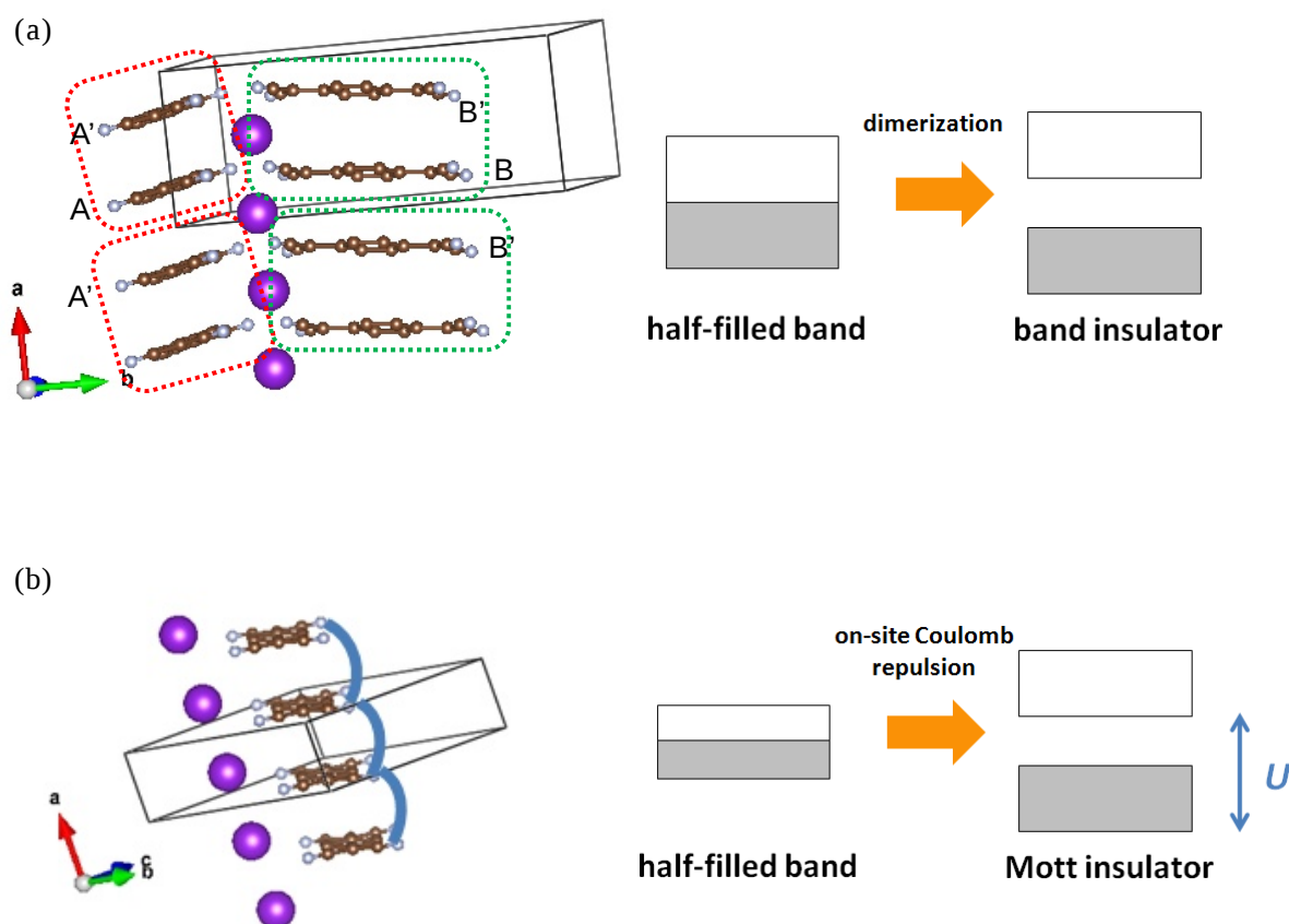
Figure 3.1.7. The crystal structure of K-TCNQ for (a) LT phase and (b) HT phase. For (a), the red and green dotted square describe two independent TCNQ columns. For (b), the blue wavy line means the TCNQ stack is uniform.
