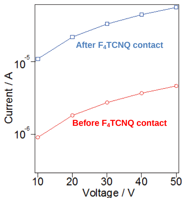
Figure 3.3.1. The current measurement of the K-TCNQ surface before and after the F 4 TCNQ powder contact.
