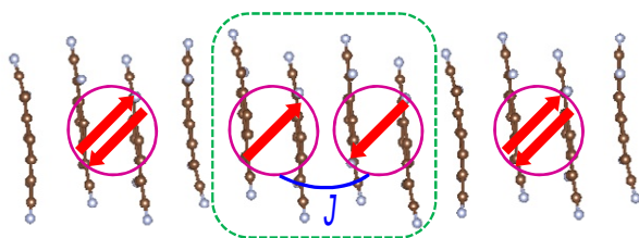
Scheme 2.8. Singlet-triplet type spin model for n = 5 . The green dashed line surrounds a pair of the TCNQ dimers that contribute to the singlet-triplet type paramagnetism.
