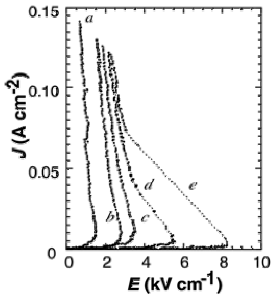
Figure 3.1.8. The negative differential resistance characteristics of K-TCNQ at different temperatures (curve a, 300 K; curve b, 280 K; curve c, 230 K; curve d, 180 K; curve e, 180 K).
