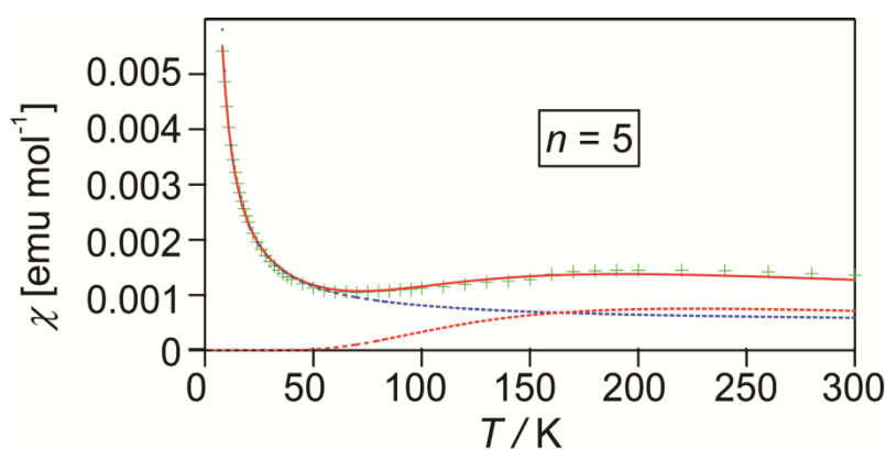
Figure 2.3.12. Magnetic susceptibility of (C5BPy)(TCNQ) 4 . The crosses are the observed values, and the solid lines are the best results of fitting.
