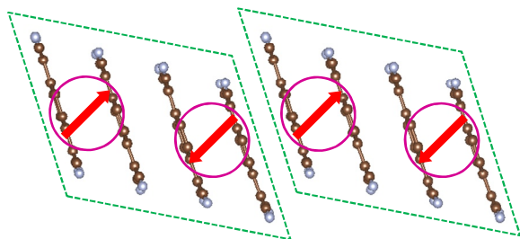
Scheme 2.6. Singlet-triplet type spin model for n = 1 . Each green parallelogram surrounds the configurational repeating unit of the TCNQ column, in which the spins form a singlet pair.
