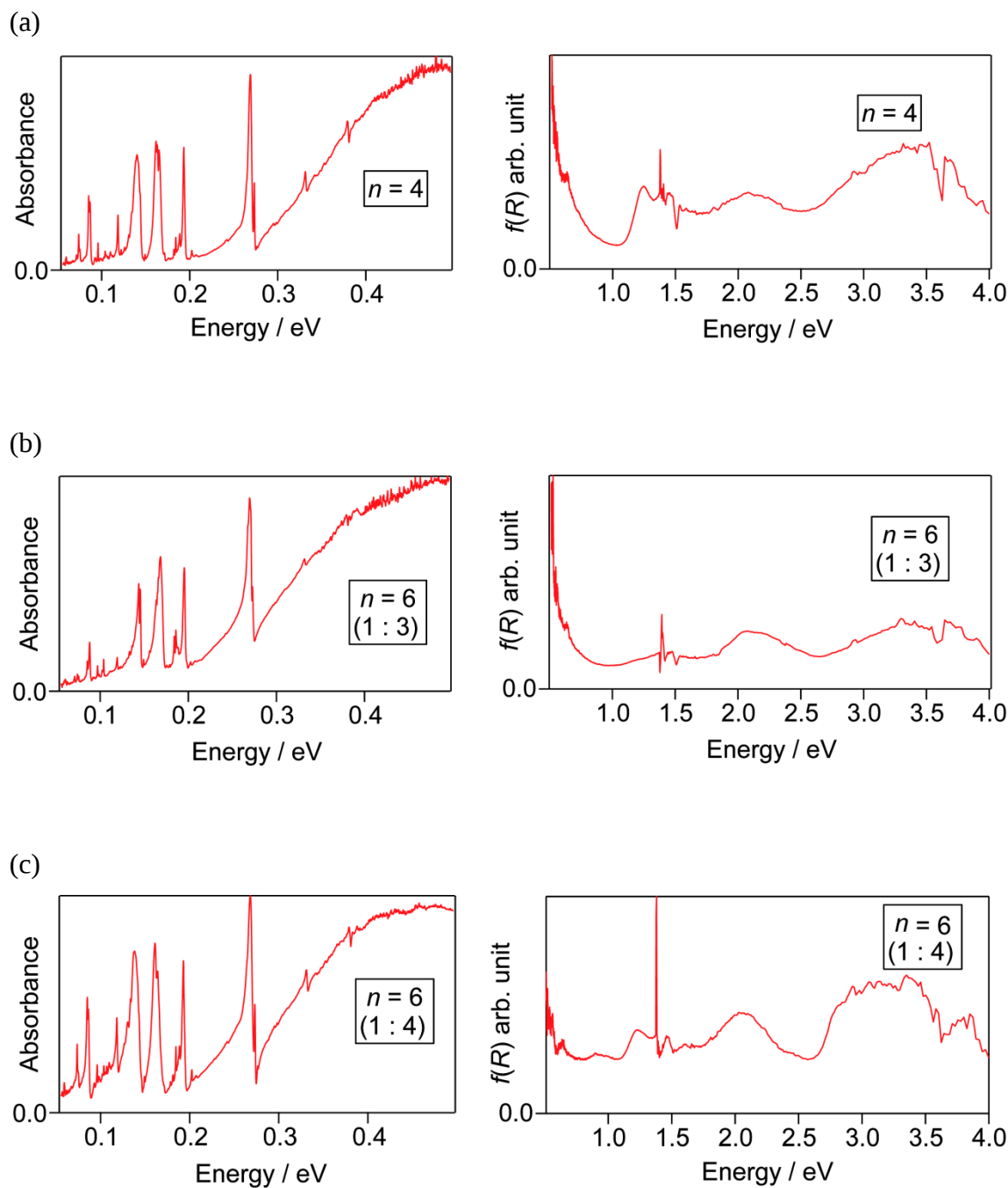
Figure 2.3.7. Optical spectra of (a) (C_4BPy)(TCNQ)_4 , (b) (C_6BPy)(TCNQ)_3 , and (c) (C_6BPy)(TCNQ)_4 . For each compound, the left-side panel indicates the IR spectrum, and the right-side panel indicates the diffuse reflectance spectrum (nearIR-vis-UV region) converted to the Kubelka-Munk function, f(R) , corresponding to the absorption. Optical spectra of other (C_nBPy)(TCNQ)_x salts are practically the same as those shown above.
