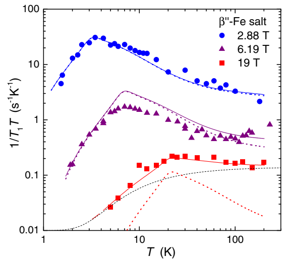
FIG. 5. Temperature dependence of 1/T_1T in three different fields. 1/T_1T is strongly suppressed in high magnetic fields. The solid lines are the result of our model calculation. The temperature and field dependence can be explained by our model. The dotted and dashed lines represent the Fe-spin contribution and the underlying \pi contribution, respectively.
