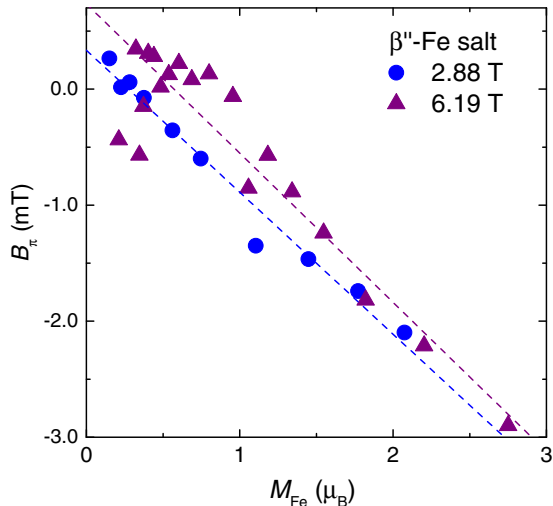
FIG. 4. The hyperfine field from \pi electrons B_\pi plotted as a function of the magnetization of Fe spins M_{\text{Fe}} . The negative slope indicates the negative exchange interaction as expressed by Eq. (5).
