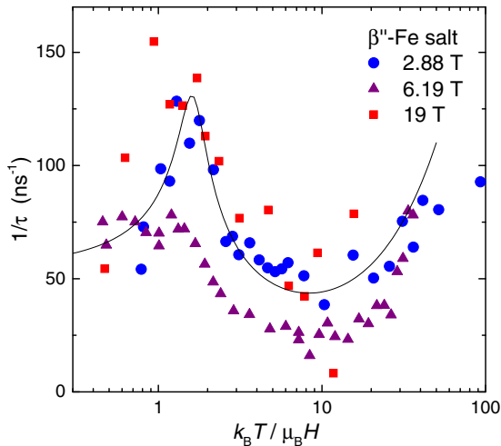
FIG. 6. Temperature dependence of Fe spin-spin correlation rate 1/\tau derived from 1/T_1 T measured at the ^{13}\text{C} site. The horizontal axis is the temperature normalized by the magnetic field t = k_B T / \mu_B H . The solid line is the fit to the data by Eq. (8).
