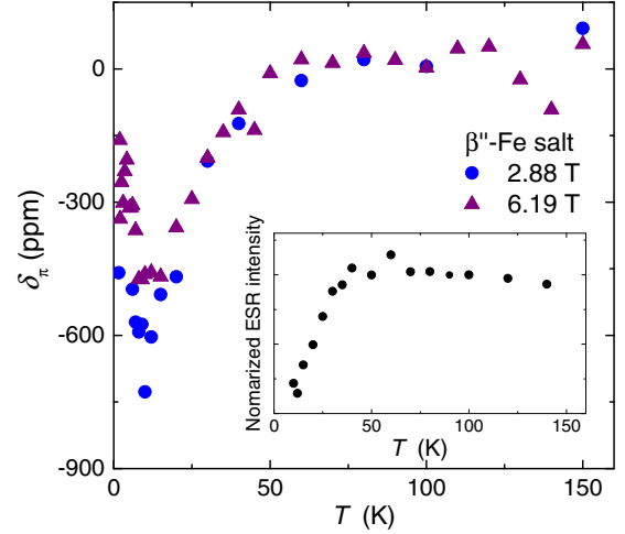
FIG. 3. Temperature dependence of the NMR shift by \pi spins \delta_{\pi} . The decrease in \delta_{\pi} observed below 50 K is explained by the negative exchange interaction between Fe and \pi spins. The inset shows the temperature dependence of ESR intensity. The decrease in ESR intensity was observed also below 50 K. This consistent behavior evidences the validity of our analysis to extract \delta_{\pi} .
