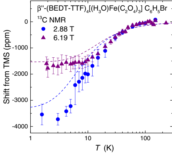
FIG. 2. Temperature dependence of the NMR shift at magnetic fields of 6.19 T and 2.88 T. Dashed lines represent the simulated temperature dependence originating from free Fe spins.
