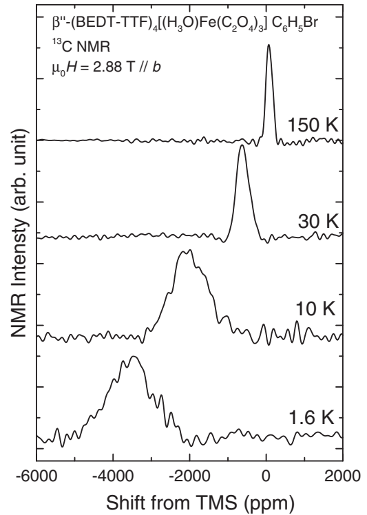
FIG. 1. Temperature dependence of 13 C NMR spectra in magnetic fields of 2.88 T applied along the b axis. A large shift and broadening were observed at low temperatures because of the large magnetization of Fe spins.
