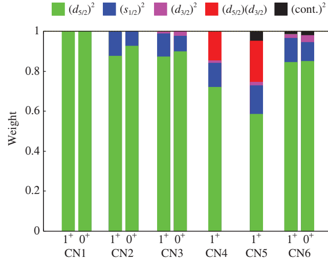
Fig. 6. Model-space dependence of the composition of the 1^+ - and 0^+ -state wave functions. “(cont.) 2 ” shows the components of higher partial waves above the sd -shell.
