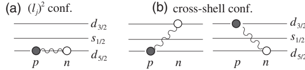
Fig. 4. A schematic figure for (a) (l_j)^2 -type ((d_{5/2})^2) and (b) “cross-shell” [(d_{5/2} \otimes d_{3/2})] configurations of valence nucleons.
