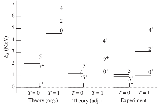
Fig. 2. Calculated and experimental [38] excitation energies of ^{18}\text{F} measured from the 1_1^+ ( T = 0 ) state. In the theoretical calculations, “(org.)” shows the calculation with the original strength of the Minnesota potential, and “(adj.)” means the calculation with an adjusted strength. For the strength parameters, please see the text.
