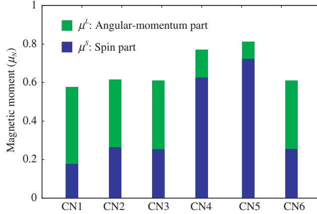
Fig. 7. Model-space dependence of magnetic moment for ^{18}\text{F}(1^+) .
