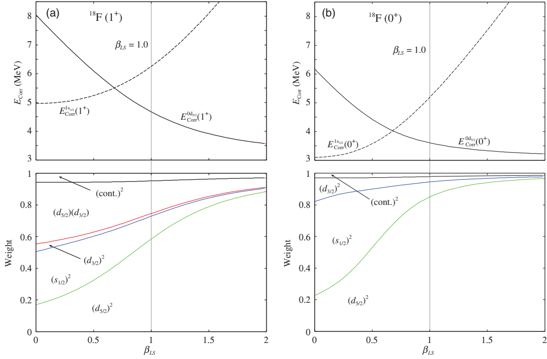
Fig. 8. Upper panels: \beta_{LS} dependence on the correlation energy for ^{18}\text{F}(1^+) and ^{18}\text{F}(0^+) . Lower panels: the weights of the wave function for the 1^+ and 0^+ states are shown.
