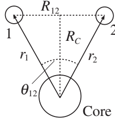
Fig. 1. Definitions of the coordinates in COSM ( \mathbf{r}_1 and \mathbf{r}_2 ) and other quantities, R_{12} , R_C , and \theta_{12} .
