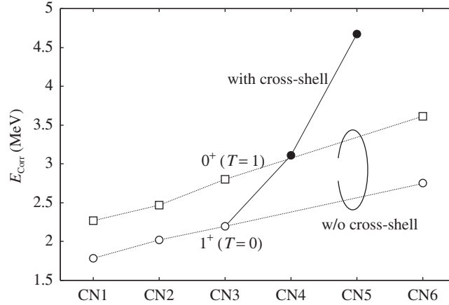
Fig. 5. Model-space dependence of the correlation energies for the 1^+ ( T=0 ) and 0^+ ( T=1 ) states of ^{18}\text{F} . Open circles and squares correspond to the calculations using only the (l_j)^2 -type configurations. The solid circles are for calculations using the cross-shell configurations. The lines are drawn to guide the eyes.
