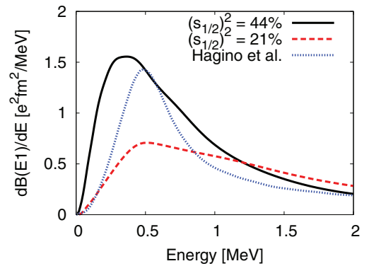
FIG. 4. (Color online) Comparison between the E1 strength distribution with different (s_{1/2})^2 components. The black (solid) line represents the present result used in Fig. 3. The red (gray) dashed line is the result of using the ground-state wave function with (s_{1/2})^2 = 21\% . The blue (gray) dotted line is the result taken from Ref. [26].
