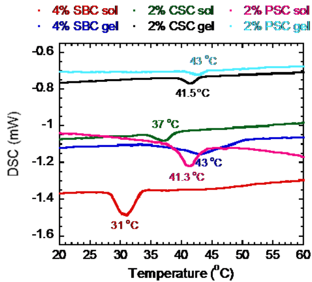
Figure 9 DSC curves of SBC, CSC and PSC (both solution and hydrogel) heated at 1°C/min.
