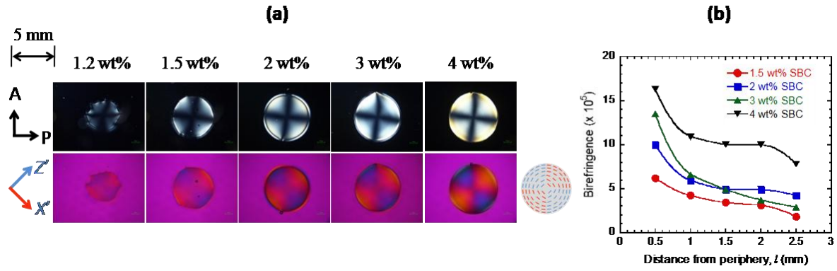
Figure 4 (a) POM images (crossed polarizer both in absence and presence of tint plate) of SBC hydrogels (1 hour gelation) prepared at 25°C having concentration ranges from 1.2 wt% to 4 wt%. Illustration of orientation structure of SBC identified by POM is shown on the right side of POM images. A: analyzer, P: polarizer, X' and Z': fast and slow axes of the tint plate, respectively. All the POM images are in same scale as shown in the top left part. (b) The birefringence variation of SBC hydrogel (2 hours gelation), with the distance from periphery to center ( l ) of the hydrogel.
