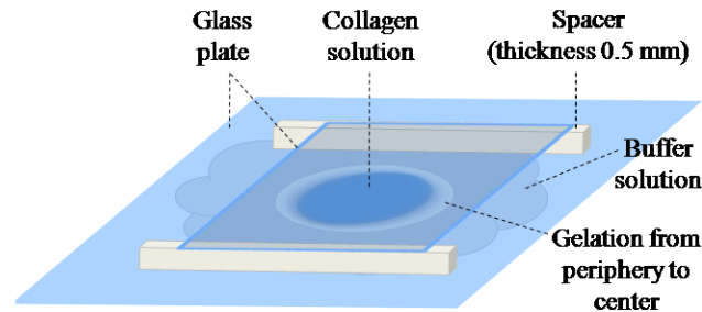
Figure 1 Set up for the diffusion induced gelation process of collagen solution. The diameter of the disc-shaped collagen solution was about 6 mm.
