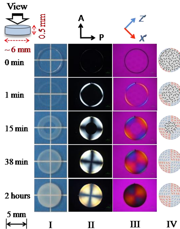
Figure 2 (I) Photographic images of 4 wt% SBC hydrogel at different gelation time. (II, III) POM images under crossed polarizer in absence (II) and presence (III) of color sensitized 530 nm tint plate. All the images are in same scale as shown in the bottom left part. (IV) Illustrations of orientation structure of SBC identified by POM. A: analyzer, P: polarizer. X' and Z': fast and slow axes of tint plate, respectively.
