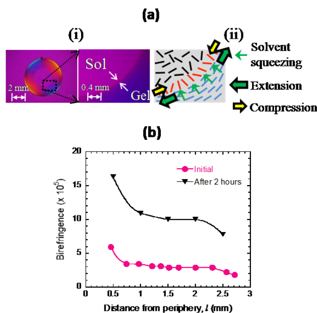
Figure 3 (a) POM image (i) of the diffusion/gelation front region under magnified lens and the corresponding schematic representation (ii) of orientation structure of SBC identified by POM. (b) The birefringence of 4 wt% SBC gel at the position right behind the advancing gelation front which corresponds to the initially formed structure (denoted as initial in the Figure) and after 2 hours gelation vs. distance from periphery to center, l .
