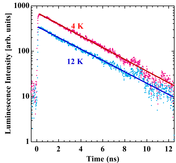
FIG. 3. Time decay of luminescence peak intensity measured at the wavelength of 1570 nm (790 meV) with the bandwidth of 20 nm (10.1 meV). The average excitation power is 0.8 \mu\text{W} (pulse peak power is 2.1 mW). The solid lines are the fitting curves obtained with a single exponential function.
