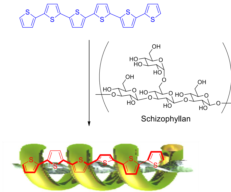
Figure 1.9 Chirality-induced host for achiral guest
