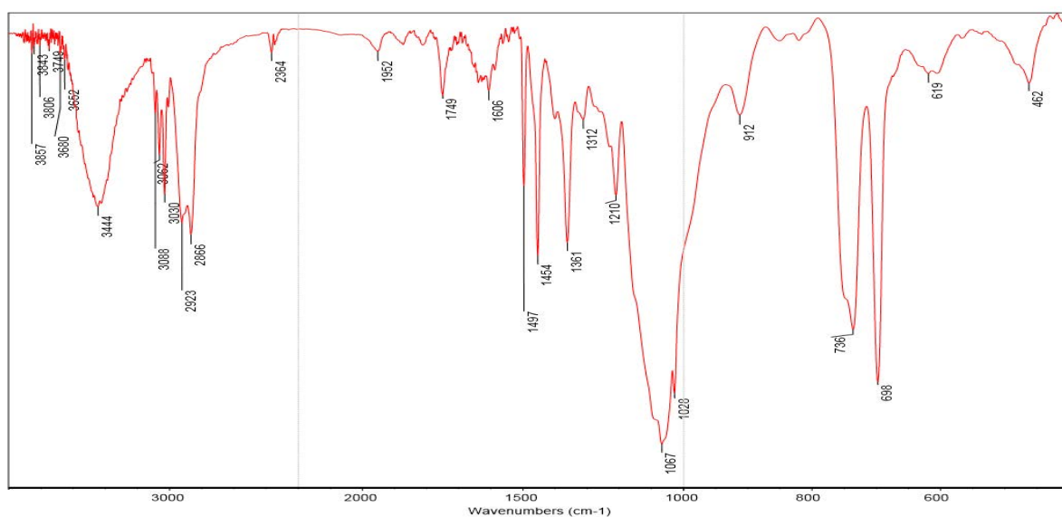
Figure 3.17 IR spectrum (KBr) of polymer obtained by the reaction using 5 mol% of TfOH at room temperature (Table 3.1, entry 5).
