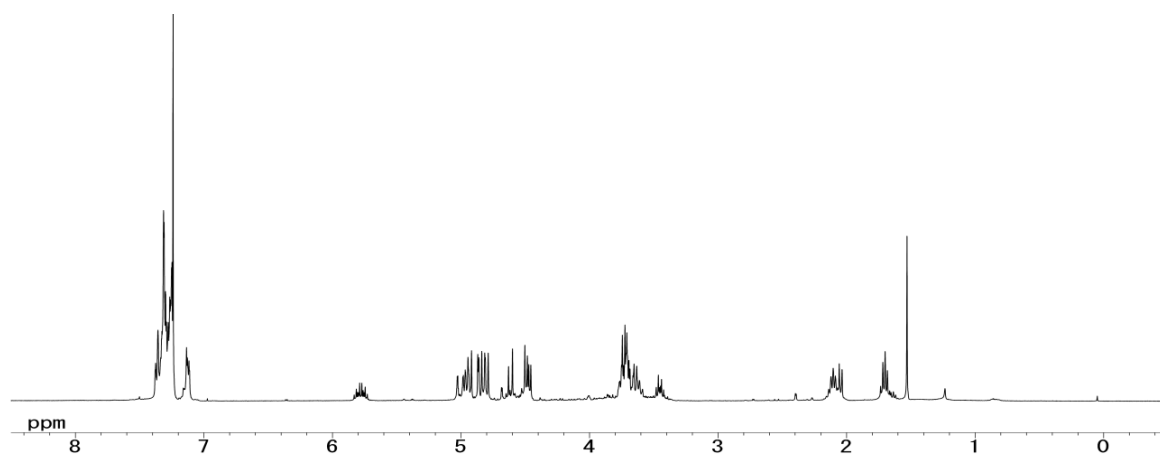
Figure 3.7 1 H NMR spectrum of 5α (400 MHz, CDCl 3 , 293 K).
