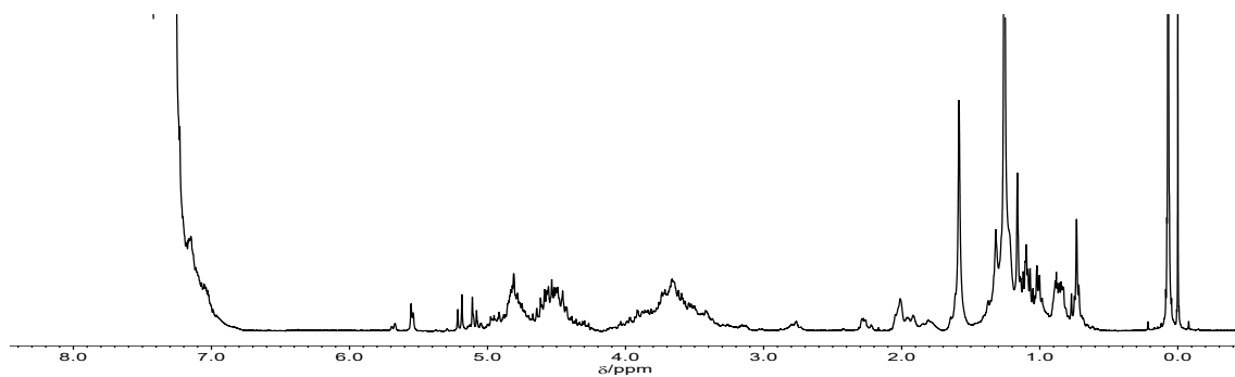
Figure 4.7 ^1\text{H} NMR spectrum of Poly-6 (400 MHz, \text{CDCl}_3 , 298 K).
