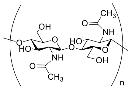
Figure 1.6 Structure of chitin.
