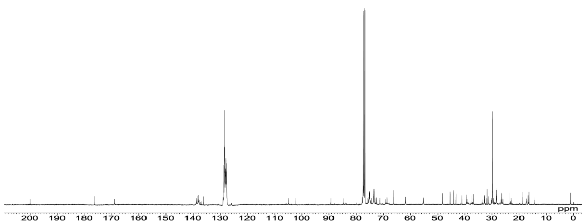
Figure S14. ^{13}\text{C} NMR spectrum of Poly-6 (100 MHz, \text{CDCl}_3 , 298 K).
