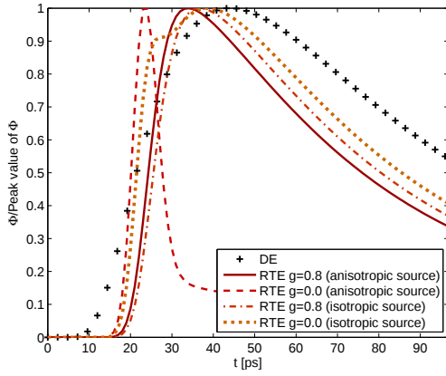
Figure 4: Calculated temporal profiles of the fluence rates \Phi at detector D1 inside the medium with the source-detector distance \rho = 0.5 cm shorter than \rho_{DA} . Crosses represent calculated results of \Phi based on the DE, solid curves those based on the RTE with g = 0.8 and the anisotropic source (\Omega_{sx}, \Omega_{sy}) = (1, 0) , dashed curves those with g = 0.0 and the anisotropic source (\Omega_{sx}, \Omega_{sy}) = (1, 0) , dash-dot (chain) curves with g = 0.8 and the isotropic source, and dotted curves those with g = 0.0 and the isotropic source.
