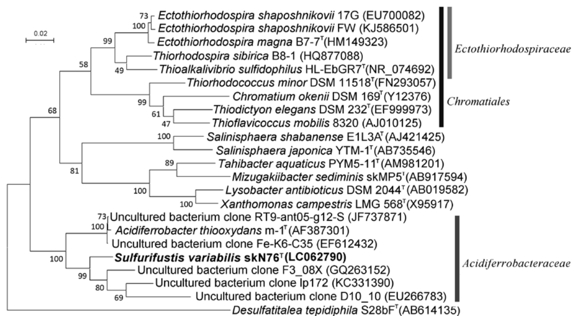
Fig. S1. Maximum-likelihood tree showing the phylogenetic position of strain skN76 T within within the class Gammaproteobacteria . Desulfatitalea tepidiphila is included as an outgroup. Numbers on nodes represent percentage values of 1000 bootstrap resampling.
