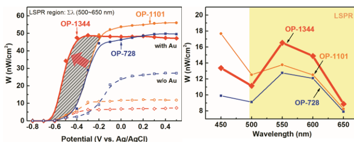
Figure 2. The output power density of the electrodes by coupling size-controlled PbS QDs with LSPR in the visible light range.
