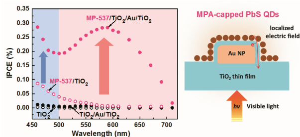
Figure 1. Enhanced photoelectric conversion efficiency not only in long wavelength range (red area) but also in short wavelength range (blue area) by coupling PbS QDs (MP-537) with Au NPs.
