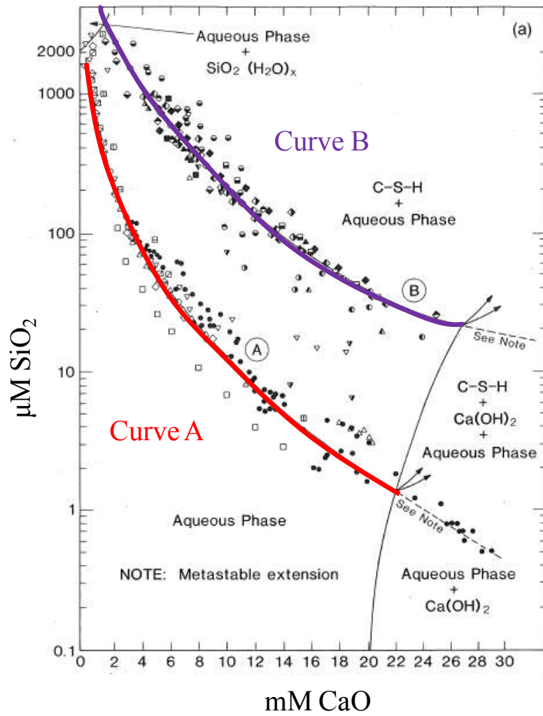
Fig. 2 The product formation due to hydration reaction of \text{C}_3\text{S}
