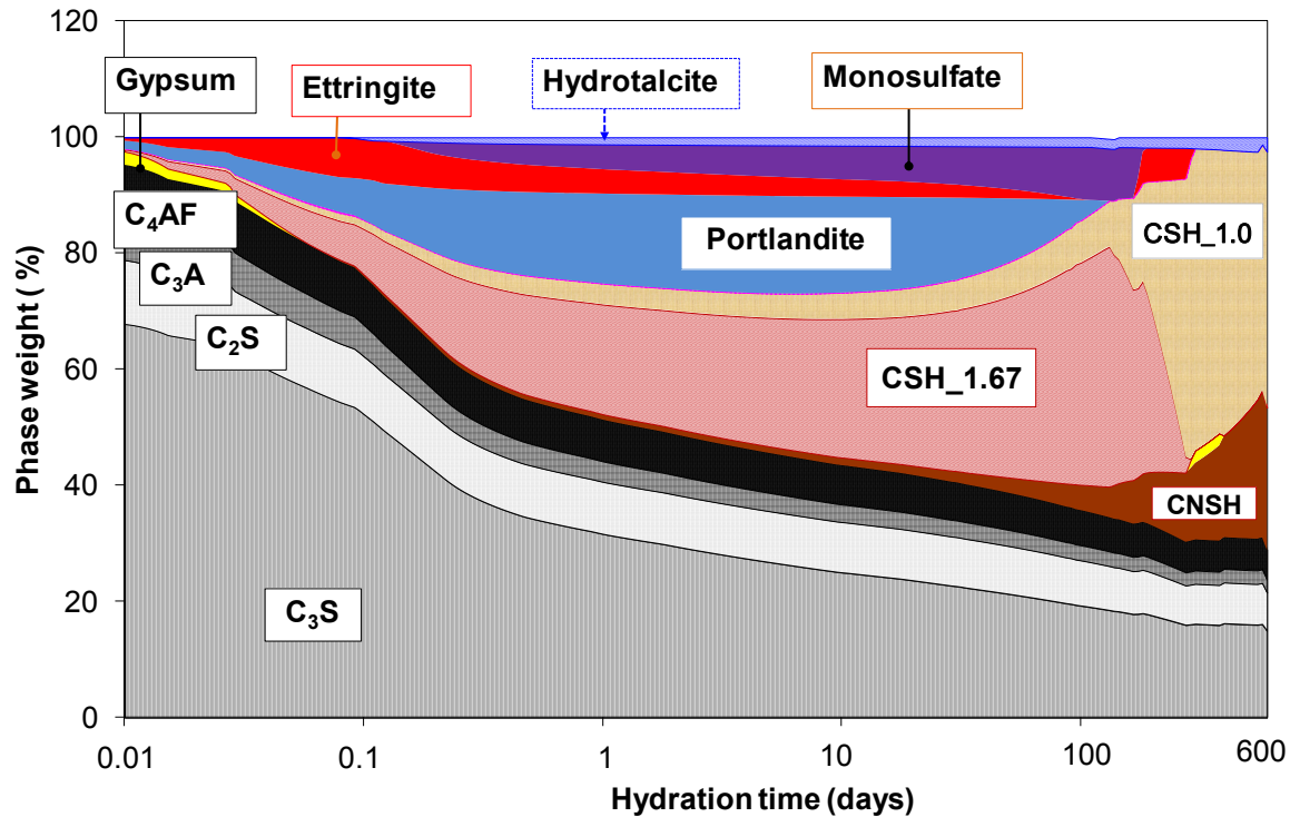
Fig. 6.6 Simulation result of PG-100 mortar
