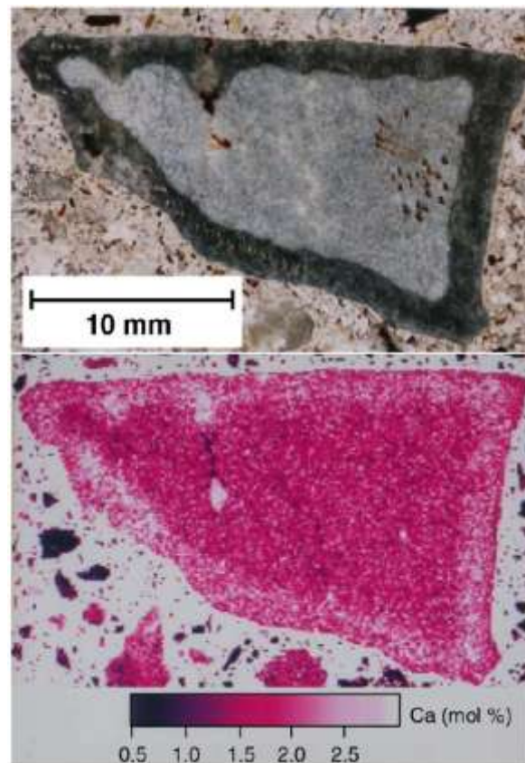
Fig. 2.2 Cross section (top) and its false color element mapping of calcium (bottom) for ASR-affected andesite.
