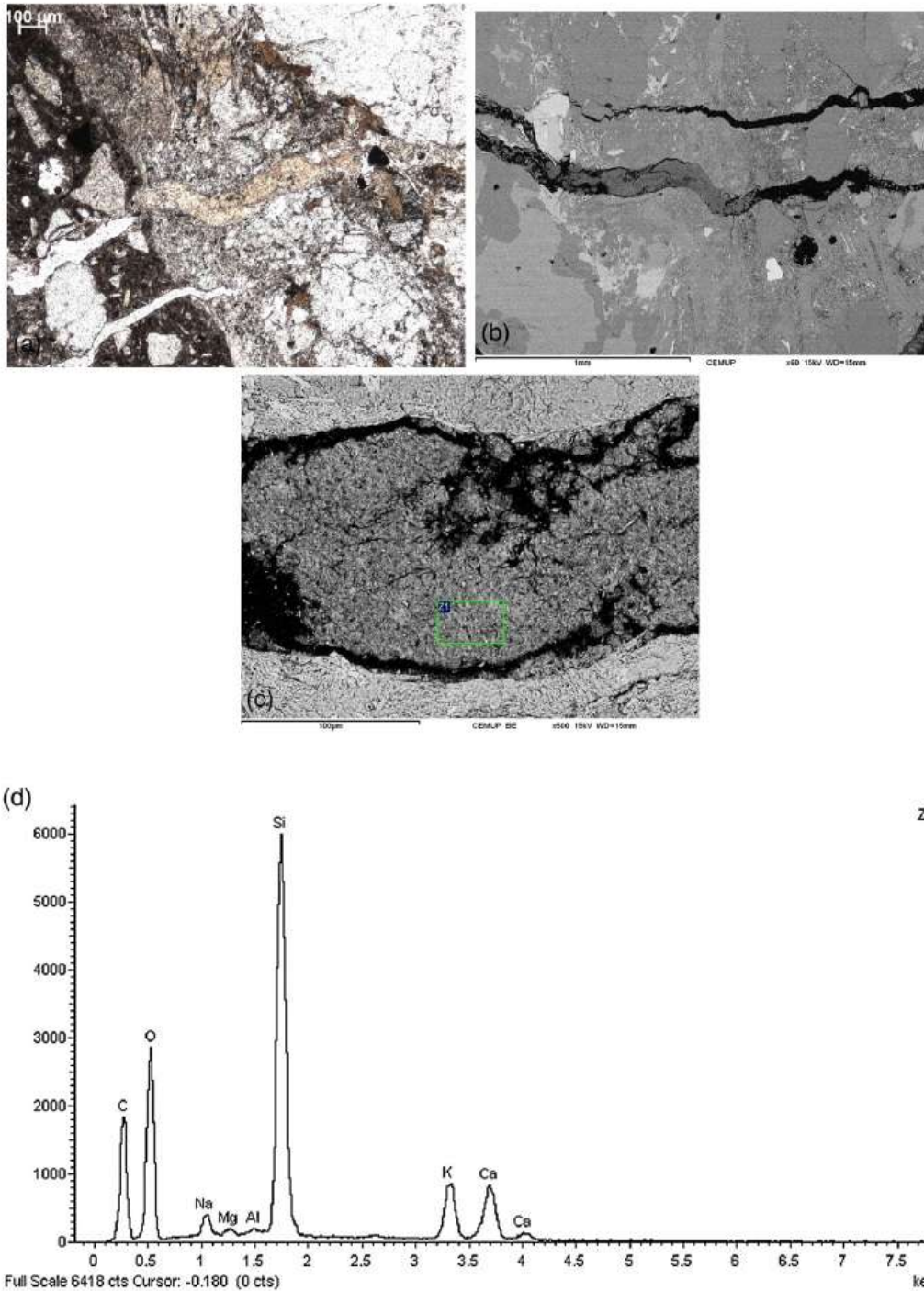
Fig. 2.8 Photomicrograph of a thin section of deteriorated structure (a) Gel partially filling cracks in the aggregate particle and extending to the cement paste, observed by polarizing microscope. (b-c) image of the same cracks by SEM (d) EDX at location Z1 in C
