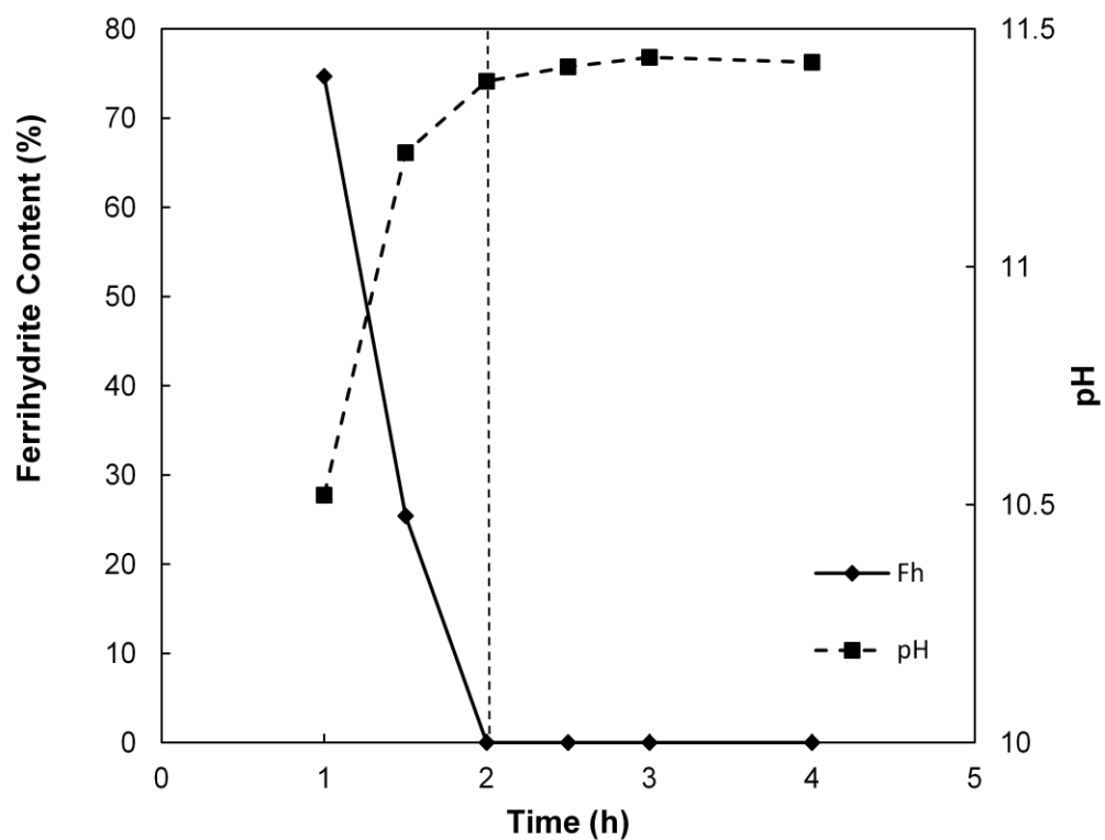
Fig. S2: Change in ferrihydrite content and pH as a function of time in Si/Fe = 0, 80°C.
