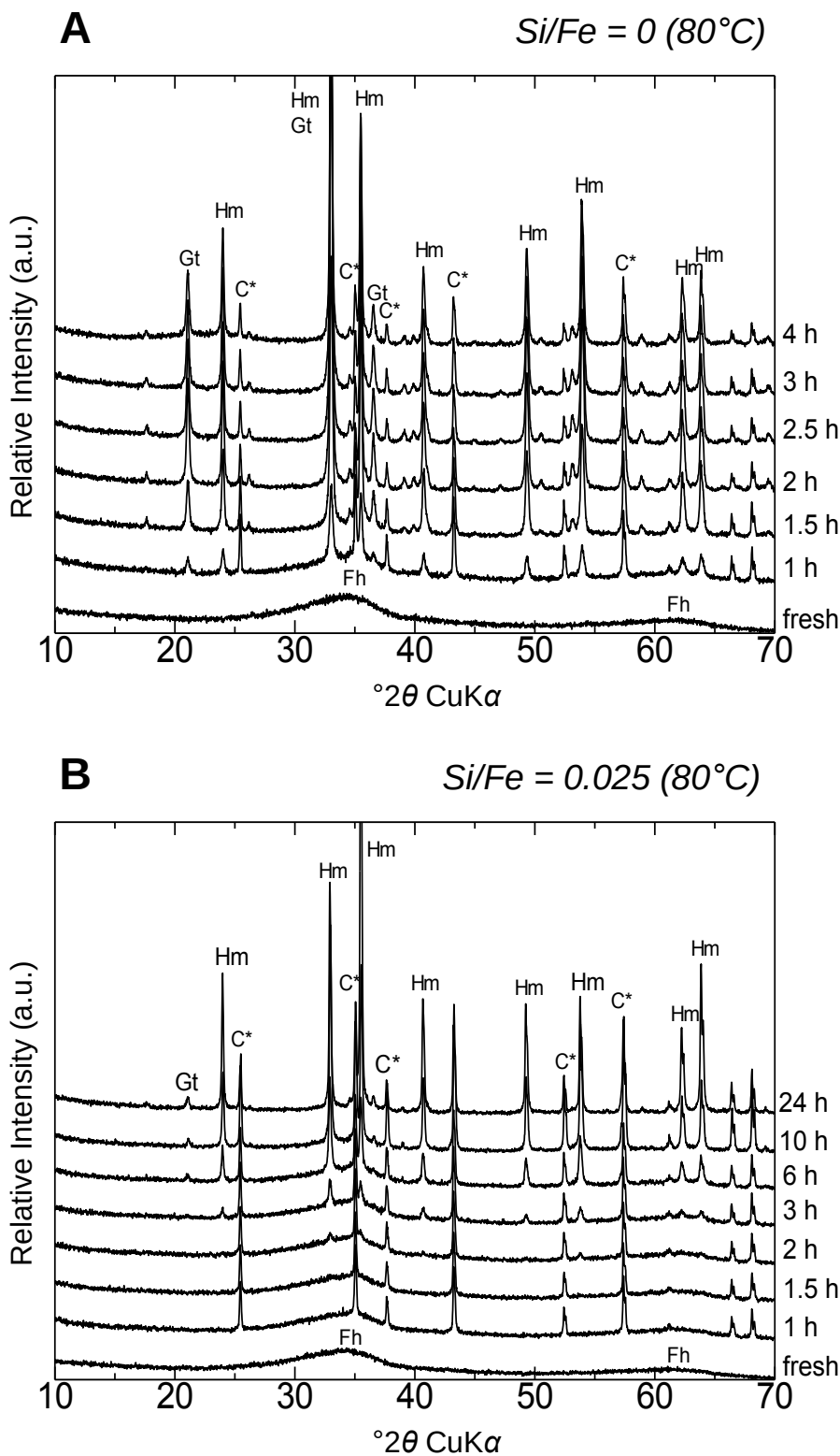
Fig. 4. XRD profiles for samples with different Si/Fe ratios (A. Si/Fe=0, pure system; B. Si/Fe=0.025) heated at 80^{\circ}C showing the crystallization over time of goethite and hematite from ferrihydrite. ( Fh : Ferrihydrite; Gt : Goethite; Hm : Hematite; C* : Corundum internal standard).
