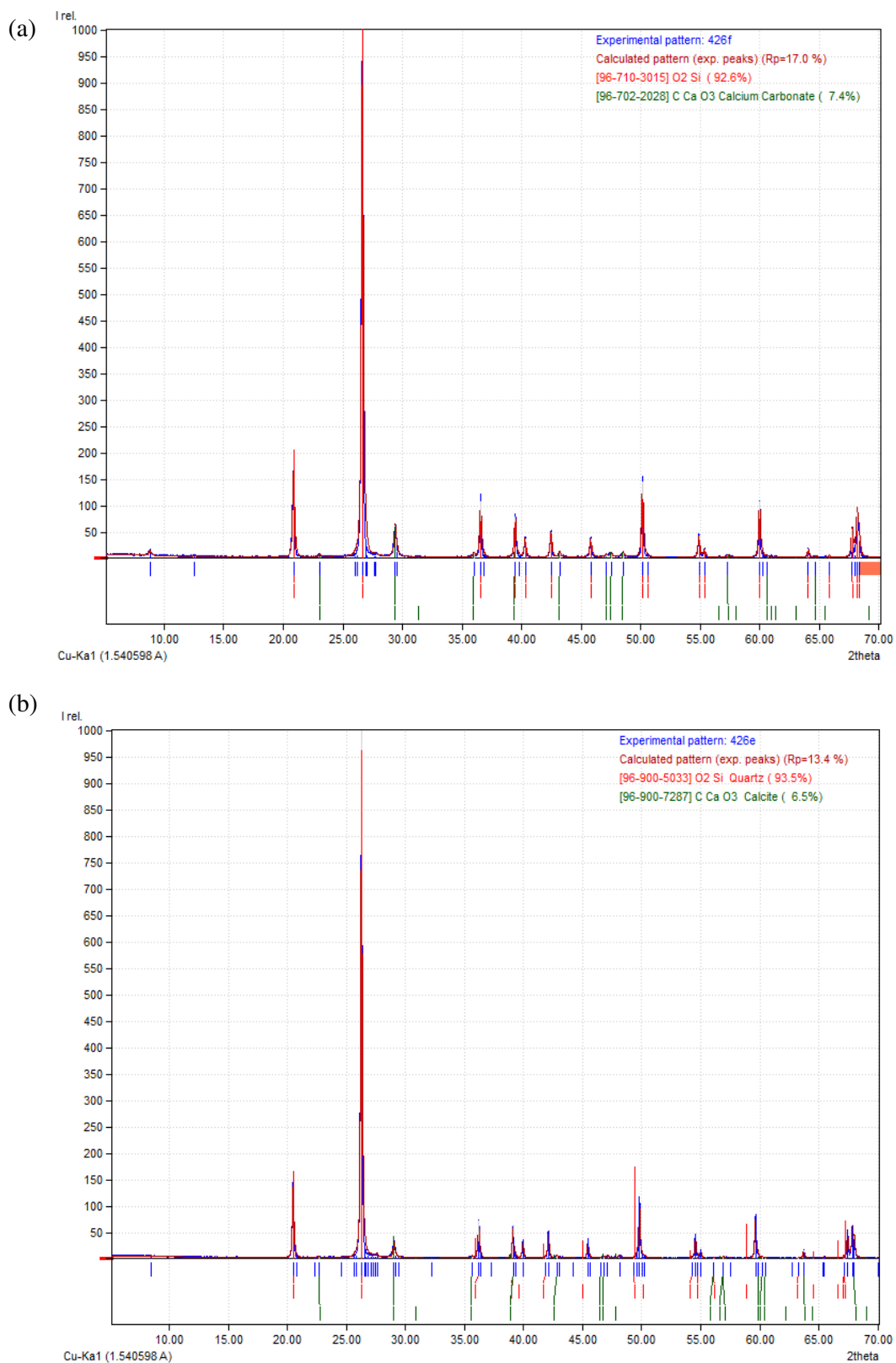
Fig. 5.41: XRD results for horizontally cored sample; (a) at the edge which is near to the outlet of the sample and (b) at the opposite edge of the sample.
