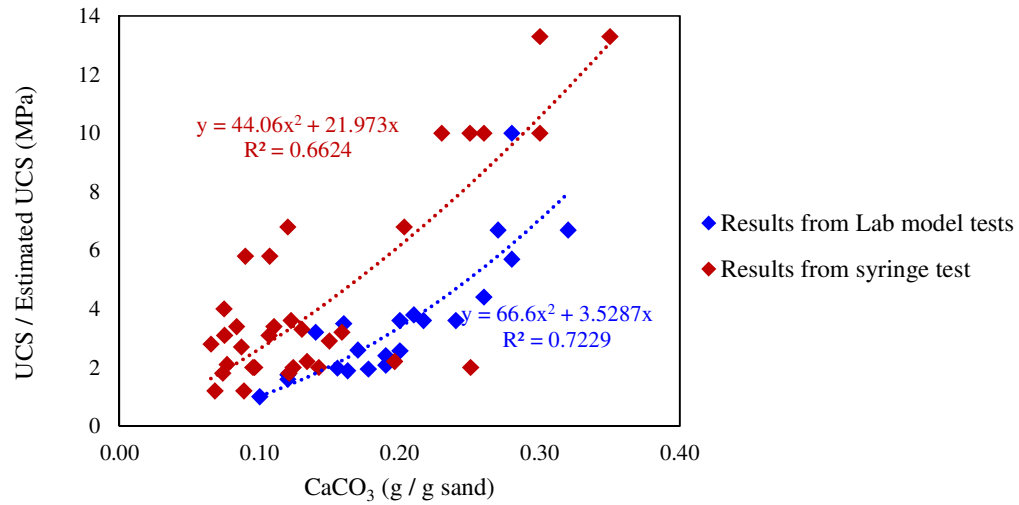
Fig. 5.44: Relationship between estimated UCS / UCS and total \text{CaCO}_3 precipitation content for syringe test and model test.
