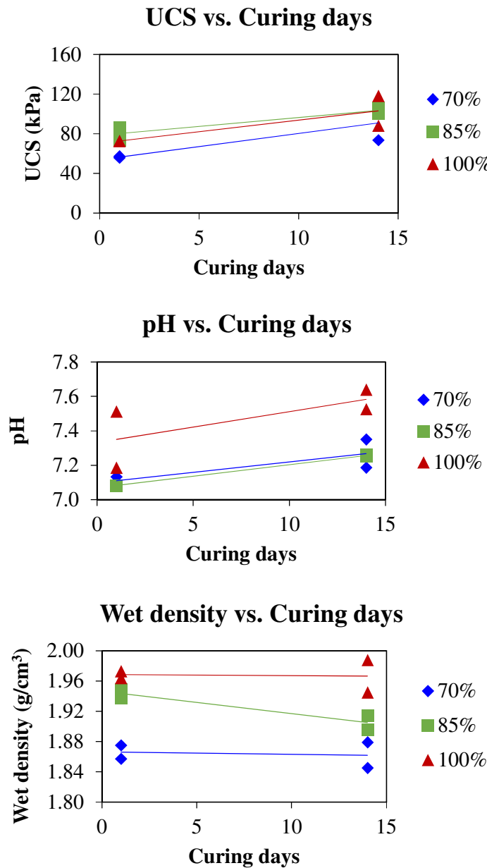
Fig. 2.20: Average UCS value, pH and wet density with the time.
