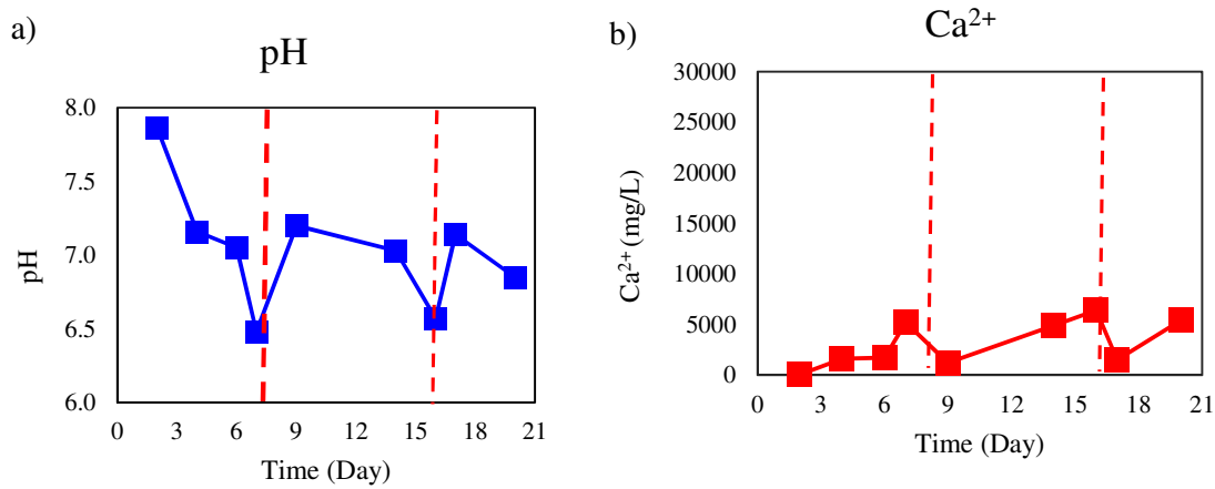
Fig. 5.32: (a) Changing pH value with the time and (b) \text{Ca}^{2+} concentration of the outlet solution of the Testing case 04.
