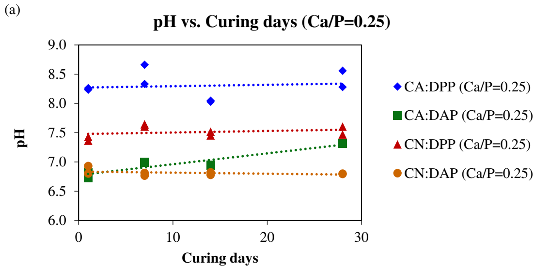
Fig. 2.11 (a): Relationship between pH and curing time of Toyoura sand test pieces cemented by \text{Ca/P} = 0.25 .
