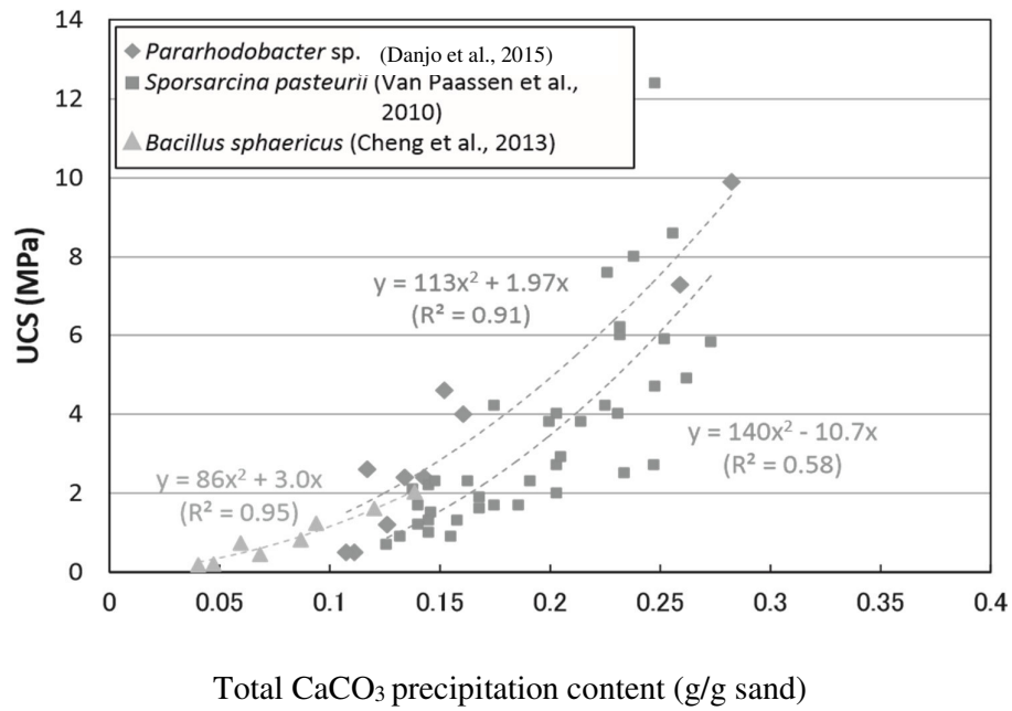
Fig. 4.23: Relationship between UCS and total \text{CaCO}_3 precipitation content for previous studies.
