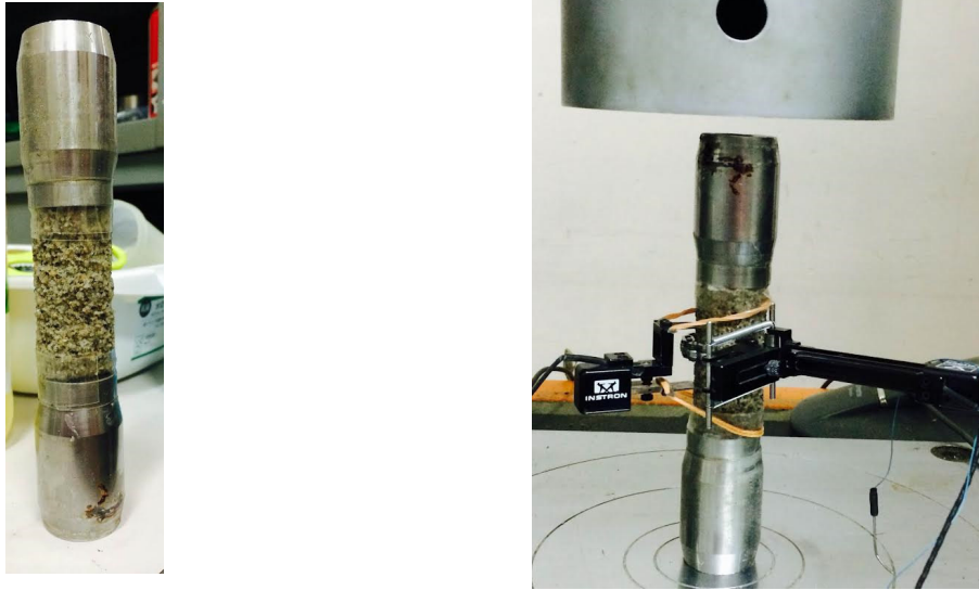
Fig. 5.5: Sample preparation before conducting UCS test.
