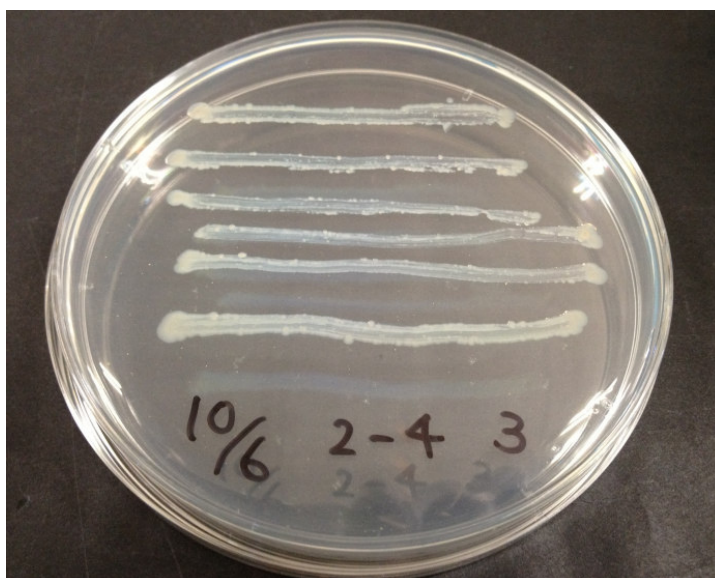
Fig. 4.2: Cultivation of Pararhodobactor sp.
