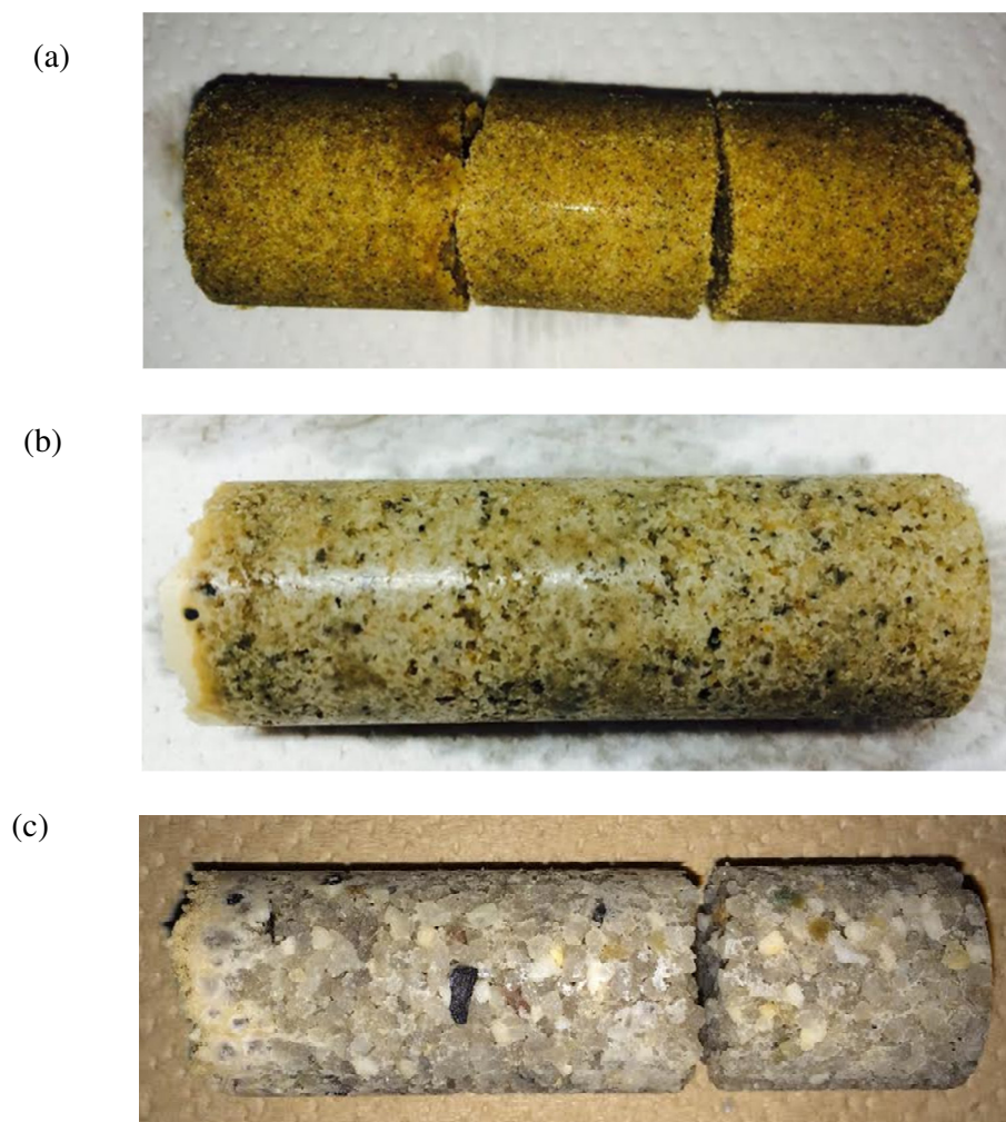
Fig. 4.20: (a) Solidified sample with Mikawa sand, (b) solidified sample with Toyoura sand and (c) solidified sample with Mizunami sand.
