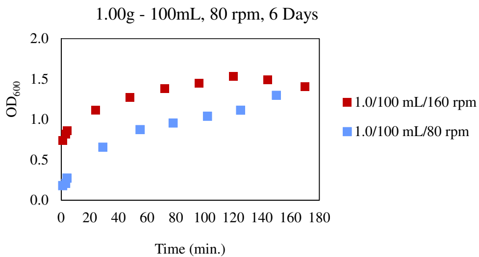
Fig. 4.10: Results of the the bacterial population in the culture solution when changing the speed of shaking.
