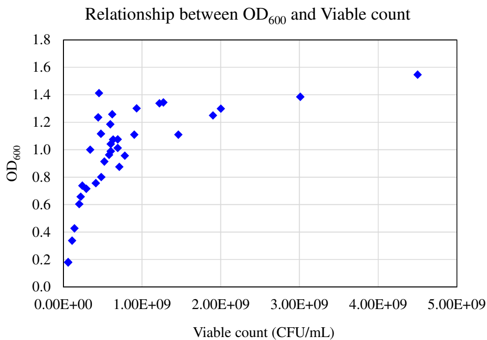
Fig. 4.11: Relationship between OD 600 and viable count measurement.
