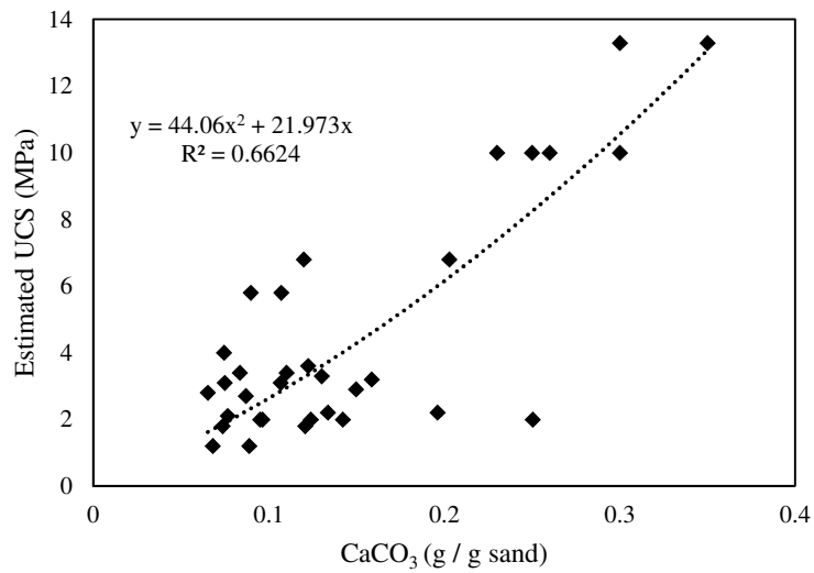
Fig. 4.24: Relationship between estimated UCS and total \text{CaCO}_3 precipitation content for this studies.
