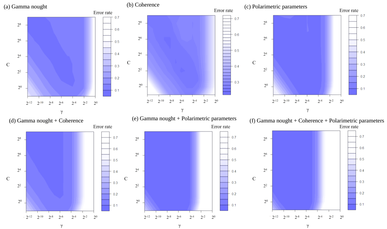
Figure 9 Results of 10-fold cross-validation for SVM classification of the training data.
