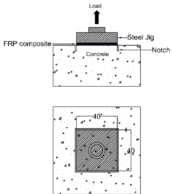
Fig. 3. Details of direct pull-off test specimen (unit: mm)
