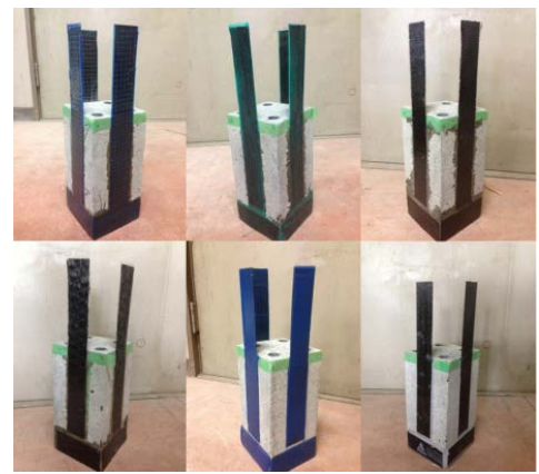
Fig. 4. (a) Preparation of the bond specimens; (b) Sample specimen for each FRP system
