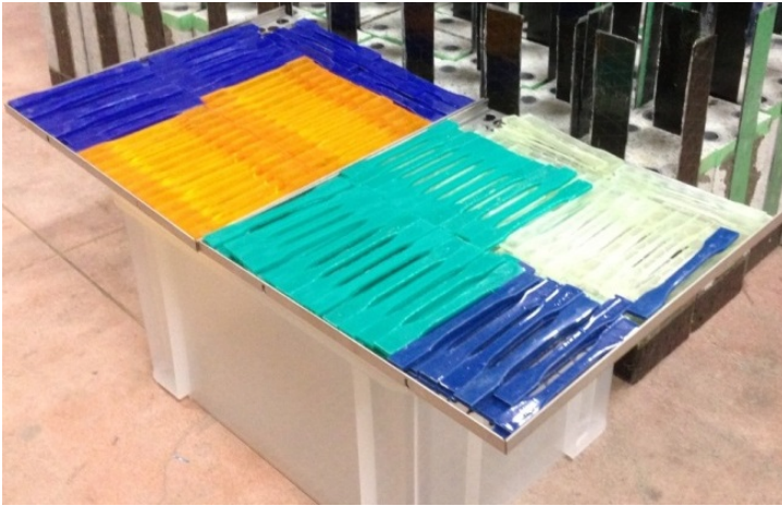
Fig. 1. Epoxy resin specimens for the tensile test
