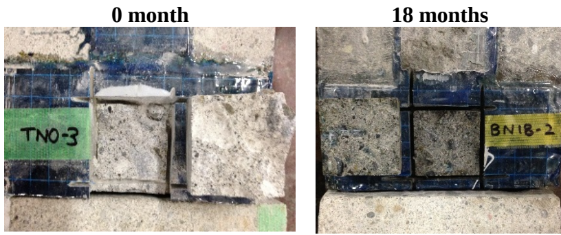
Fig. 20. Comparison of typical failure mode before and after 18 months of exposure
