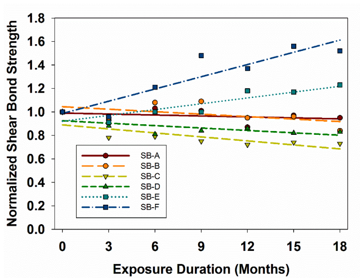
Fig. 15. Relationship between normalized shear bond strength and the exposure duration
