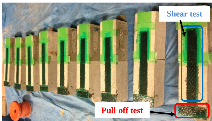
Fig. 4. (a) Preparation of the bond specimens; (b) Sample specimen for each FRP system
